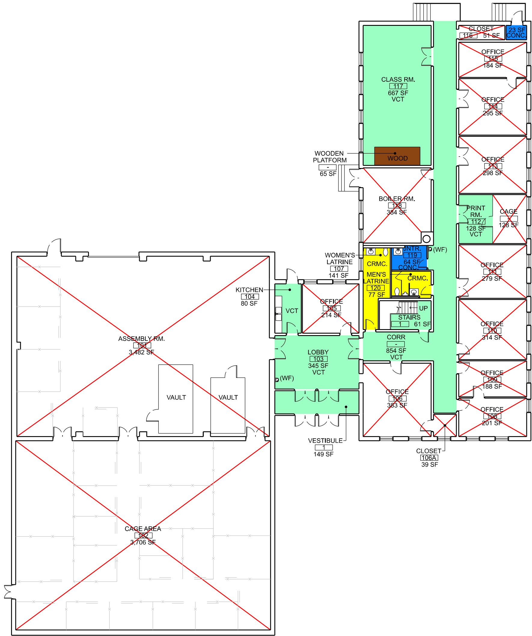
1 FIRST FLOOR CUSTODIAL SERVICE PLAN - USARC SCALE: 1/16" = 1'-0"
