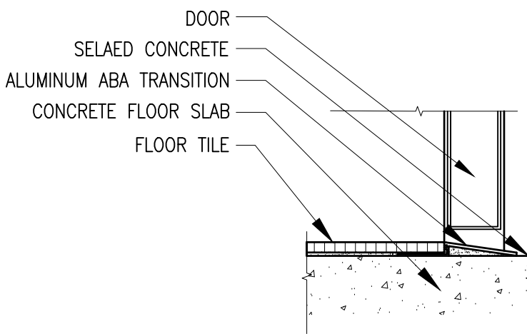
B4 PT TO SC TRANSITION SCALE: 1:5 IN601
