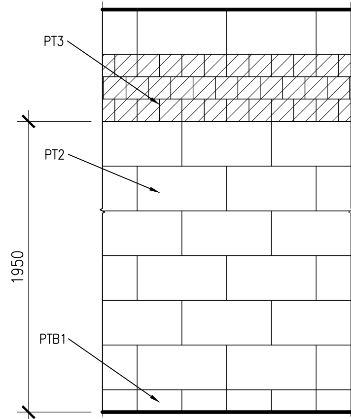
C4 ACCENT WALL TILE ELEVATION SCALE: 1:25 IN601
