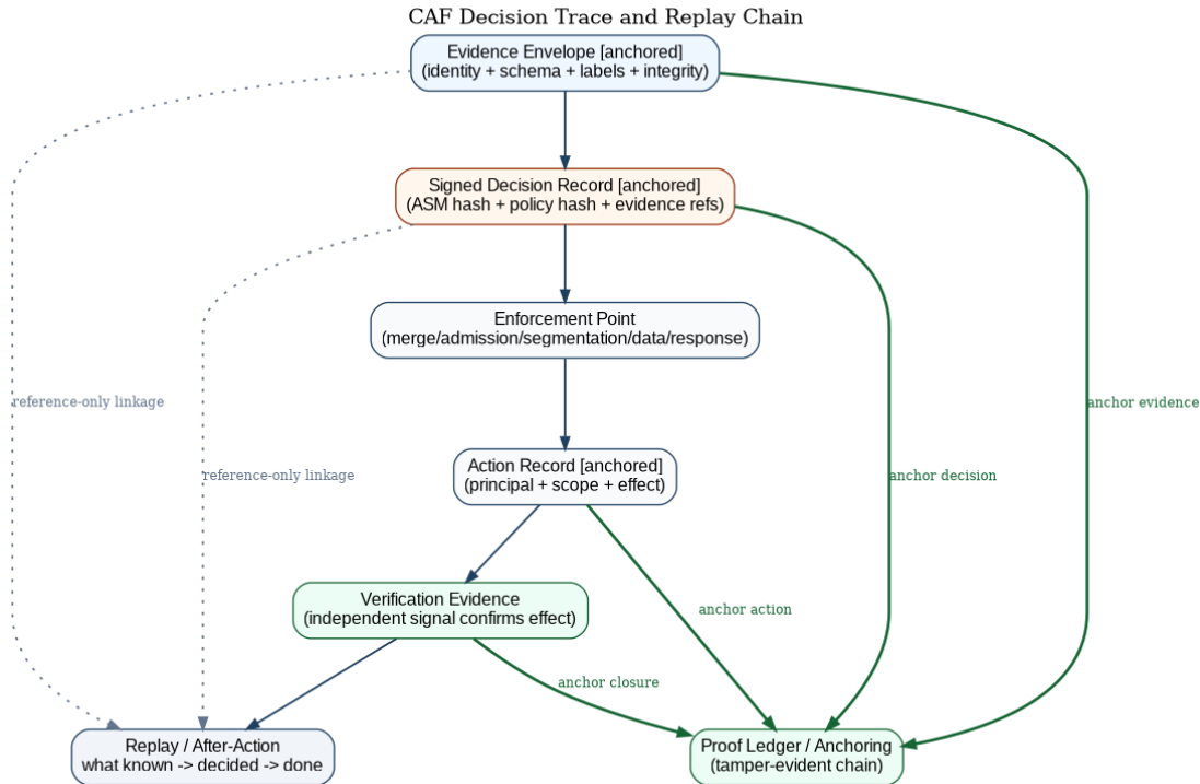
Figure 7: CAF decision trace from evidence to replay, including explicit proof-ledger anchoring on core artifacts
