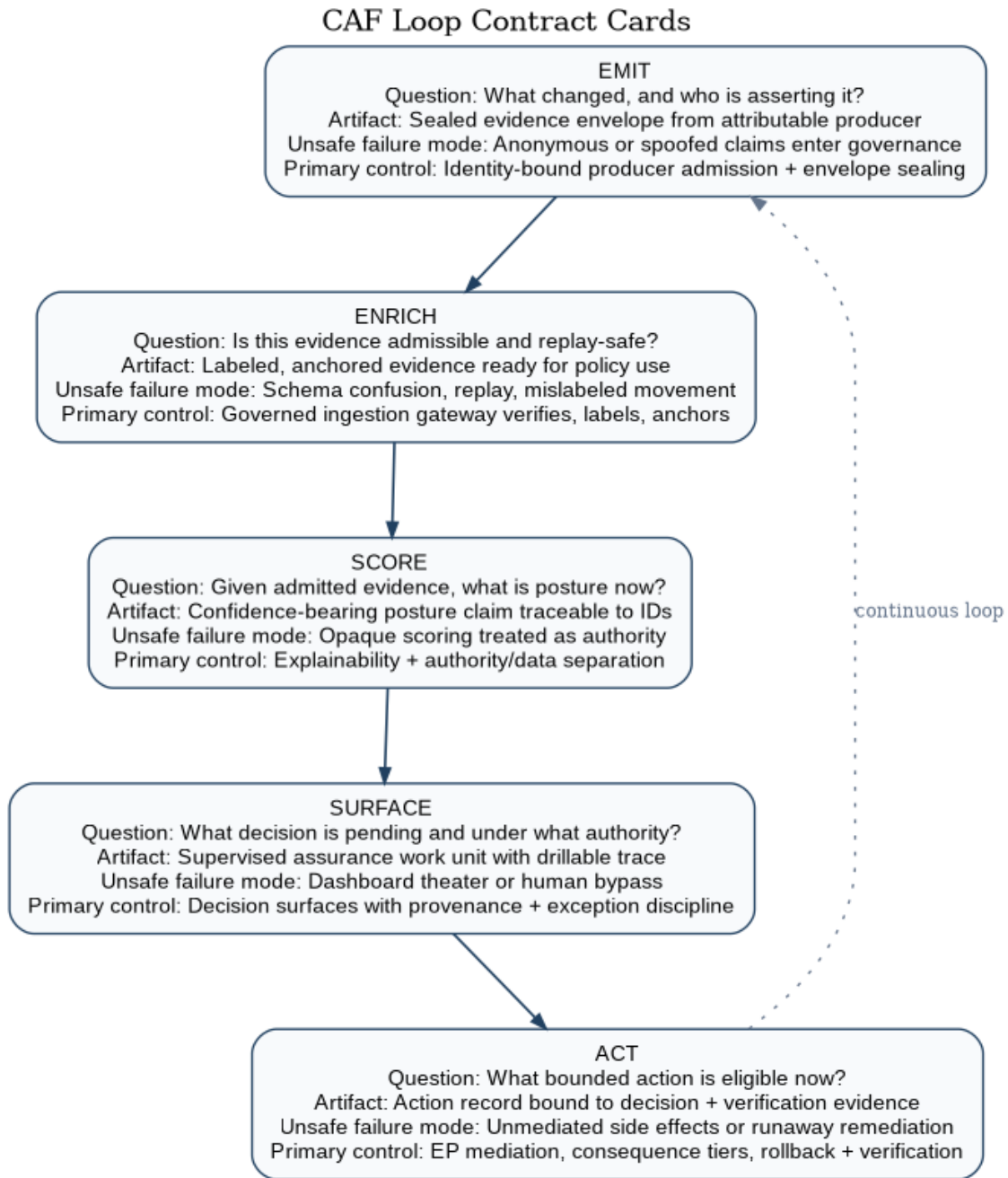
Figure 3: CAF loop contract cards: each stage specifies question, artifact, unsafe failure mode, and primary control
