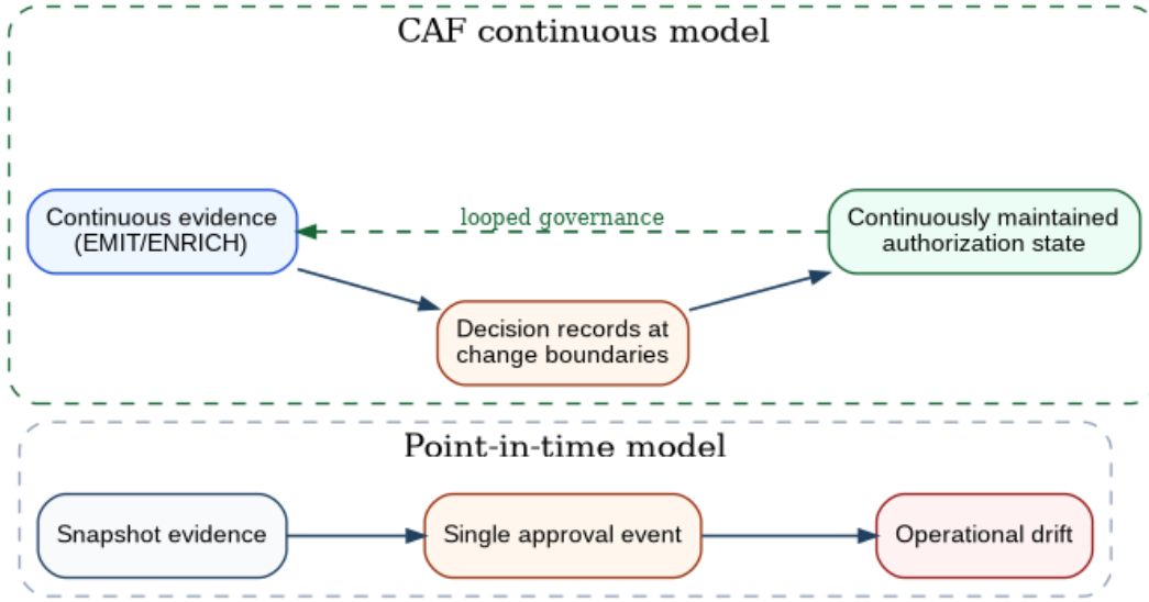
Figure 1: Point-in-time approval drifts; CAF maintains authorization state continuously at governed change boundaries
