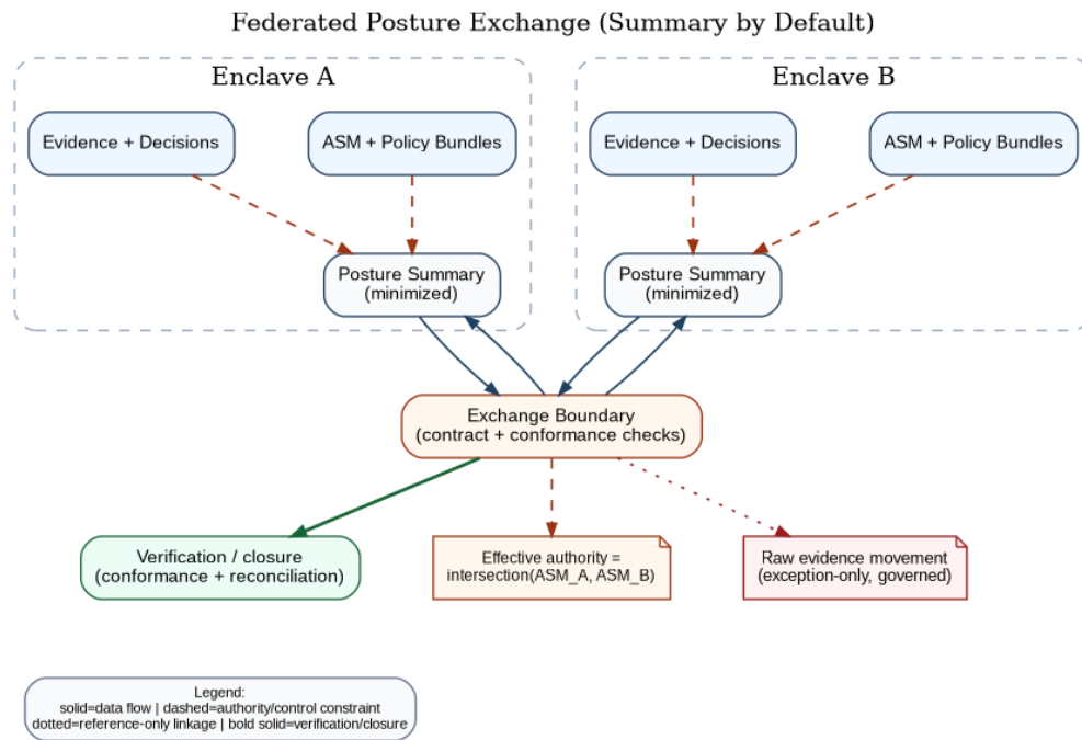
Figure 12: Federated posture exchange with summary-by-default discipline and intersection authority rule
