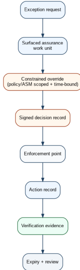
Governed Exceptions and Overrides Sequence
