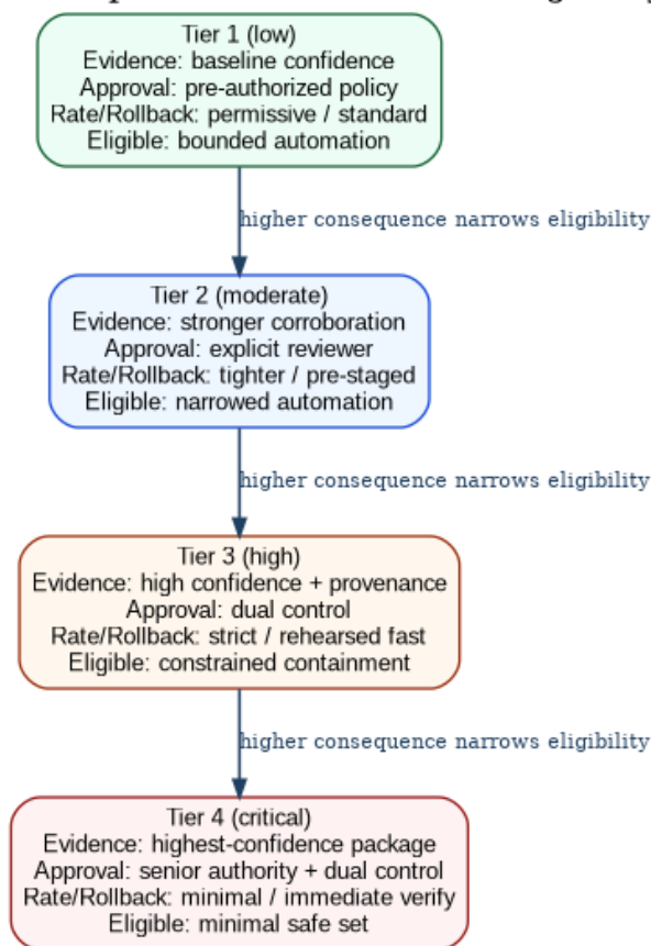
Figure 6: Consequence tiers tighten evidence/approval constraints and narrow action eligibility
