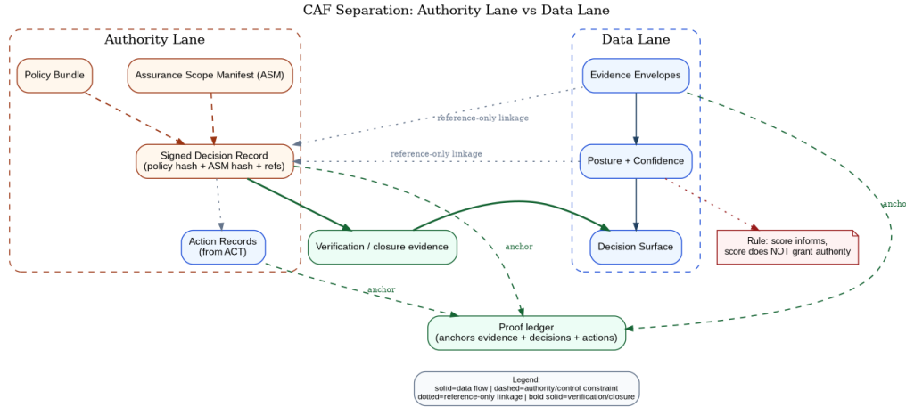
Figure 8: Authority artifacts and data artifacts remain separate while sharing proof-ledger anchoring
