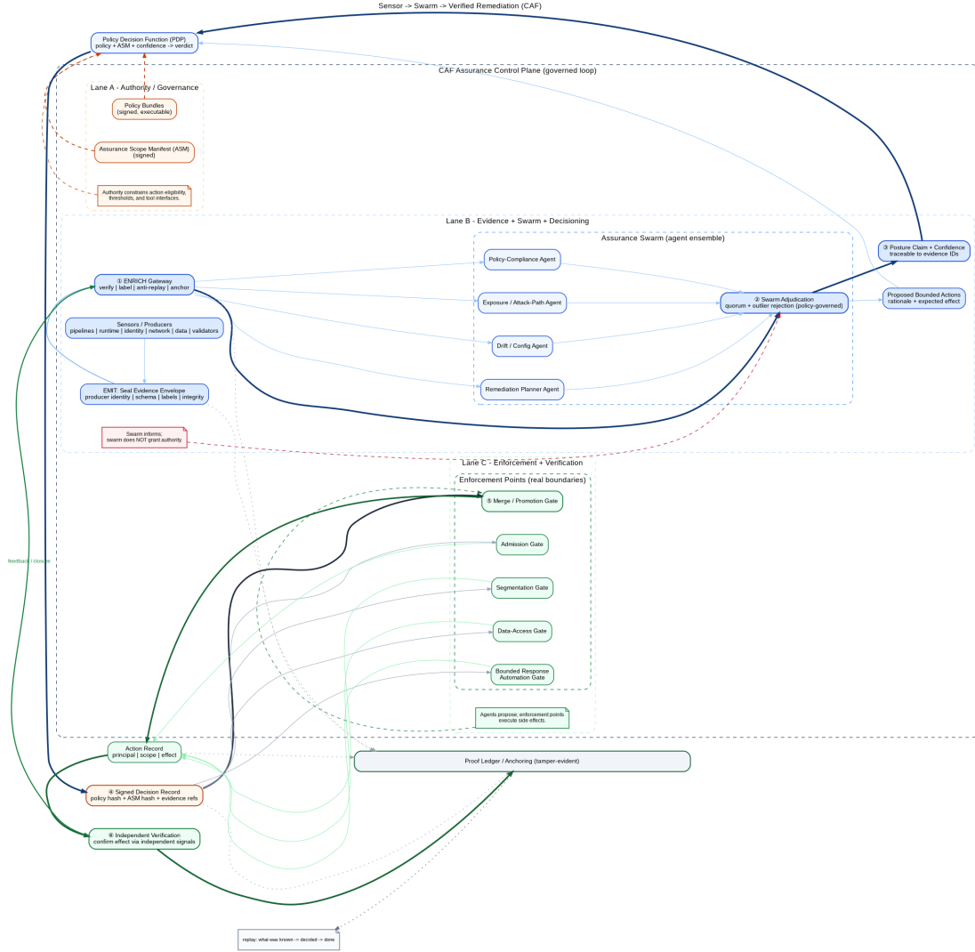
Figure 5: Sensor-to-swarm-to-verified-remediation loop. Sensors emit sealed evidence; an assurance swarm adjudicates with quorum/outlier rejection to produce posture + confidence and bounded recommendations; policy + manifests issue a signed decision record; enforcement points execute bounded action; independent verification closes the loop and anchors proof for replay.
