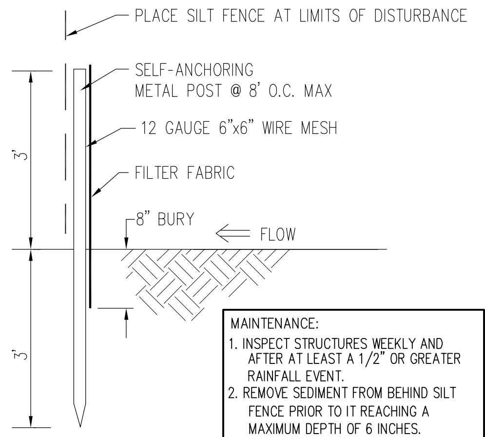
A1 SILT FENCE NOT TO SCALE
