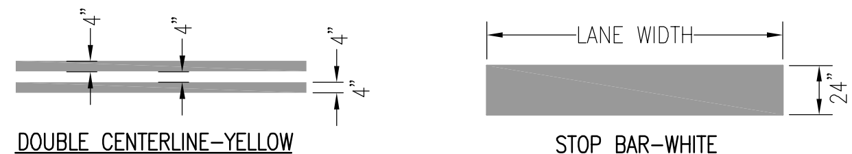
D4 PAVEMENT MARKINGS NOT TO SCALE
