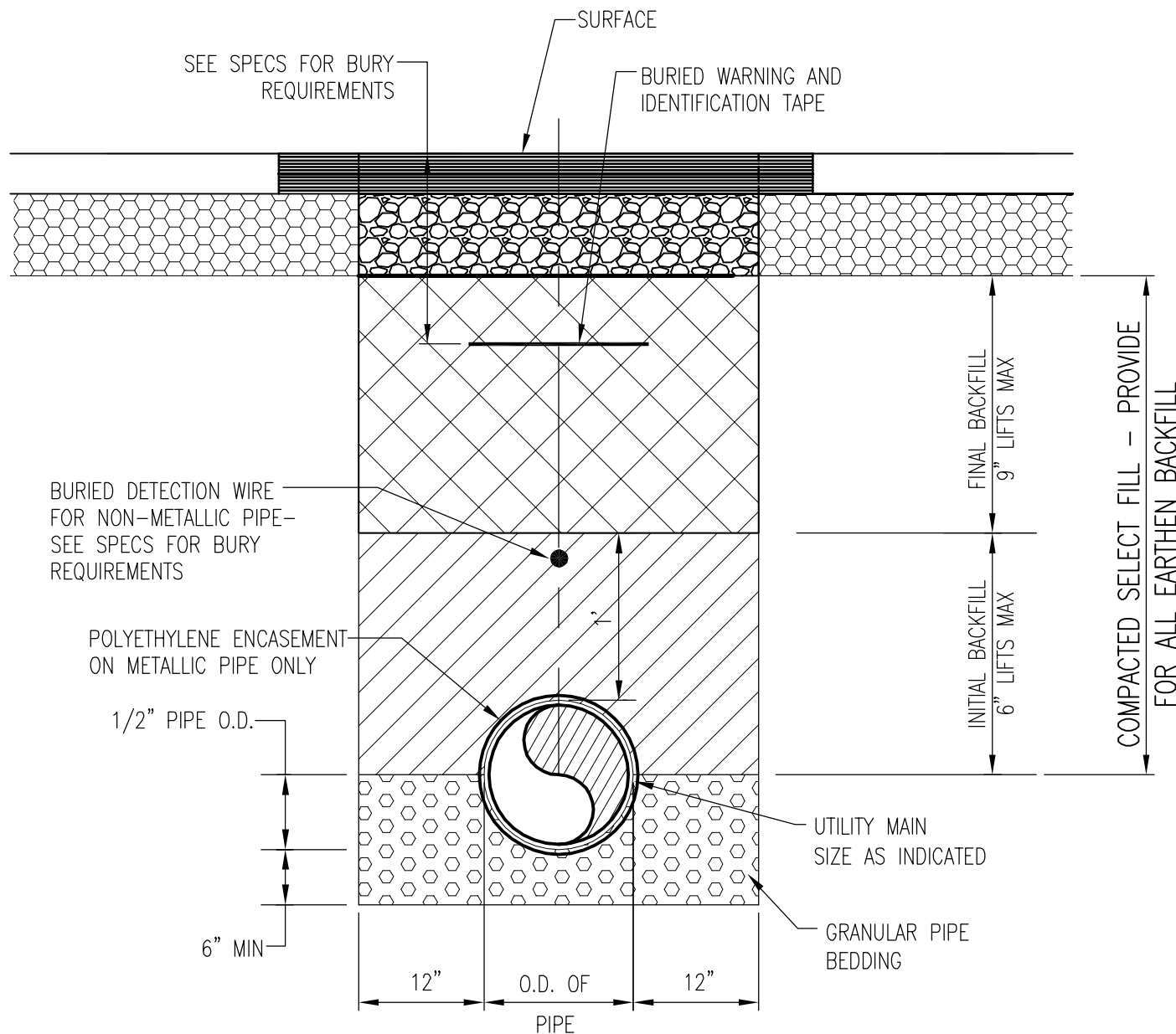
A3 TRENCH SECTION NOT TO SCALE
