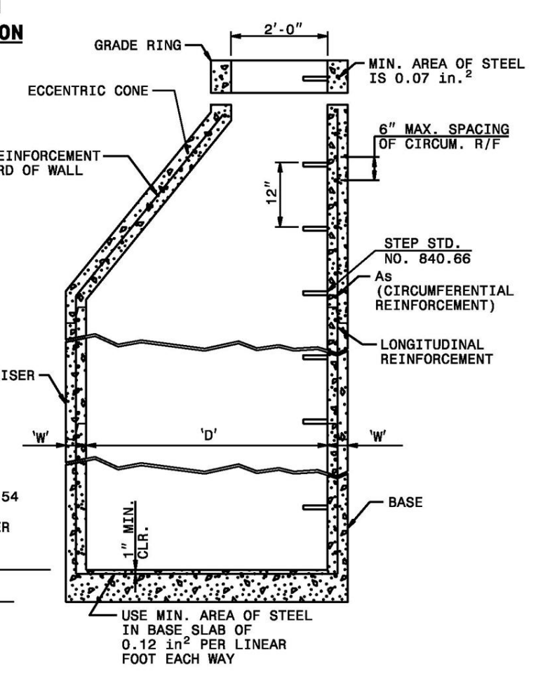
TYPICAL MANHOLE SECTION
