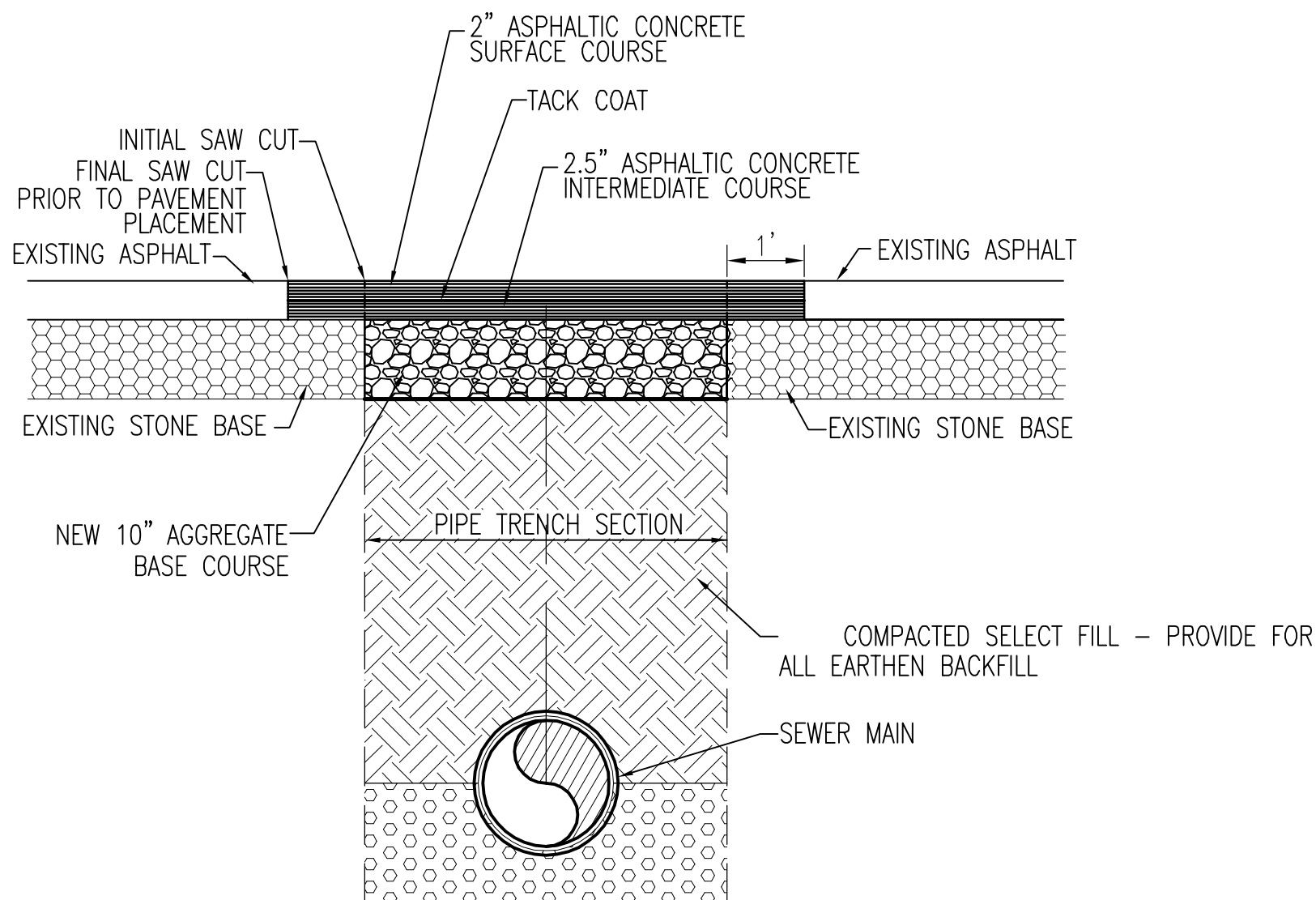
C1 ASPHALT CUT AND PATCH NOT TO SCALE
