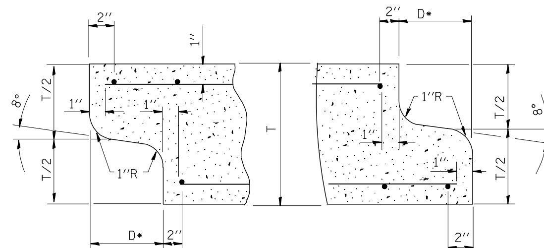
DETAIL A (TYP INLET END)
