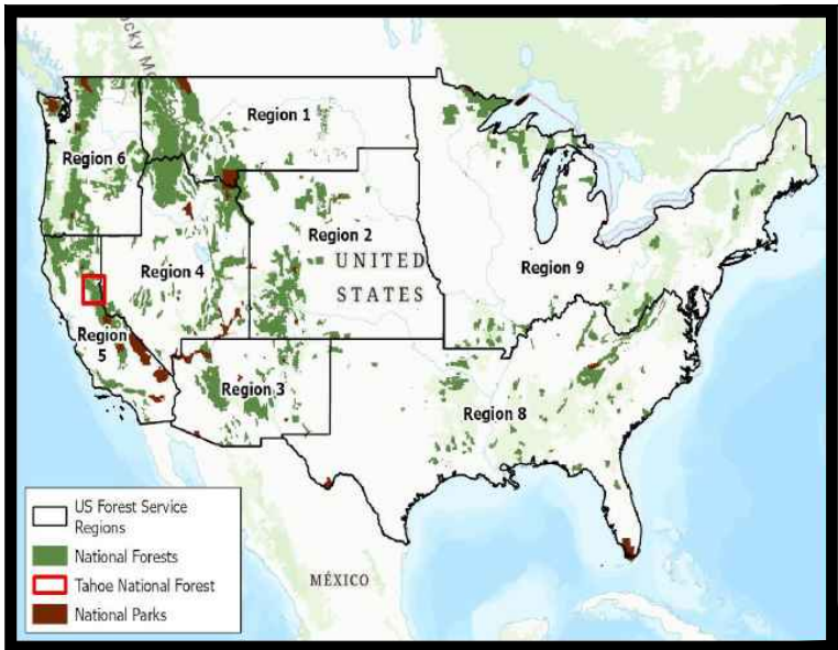
VICINITY MAP
