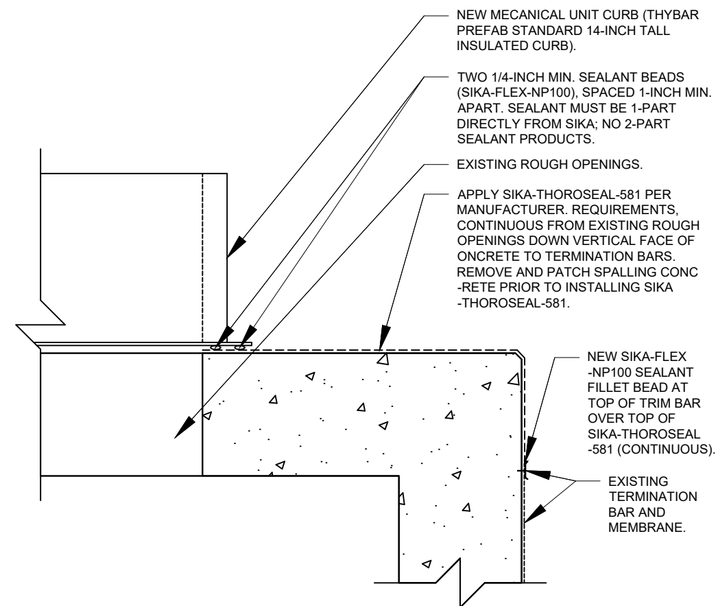
WEATHER RESISTANT BARRIER COATING DETAIL
