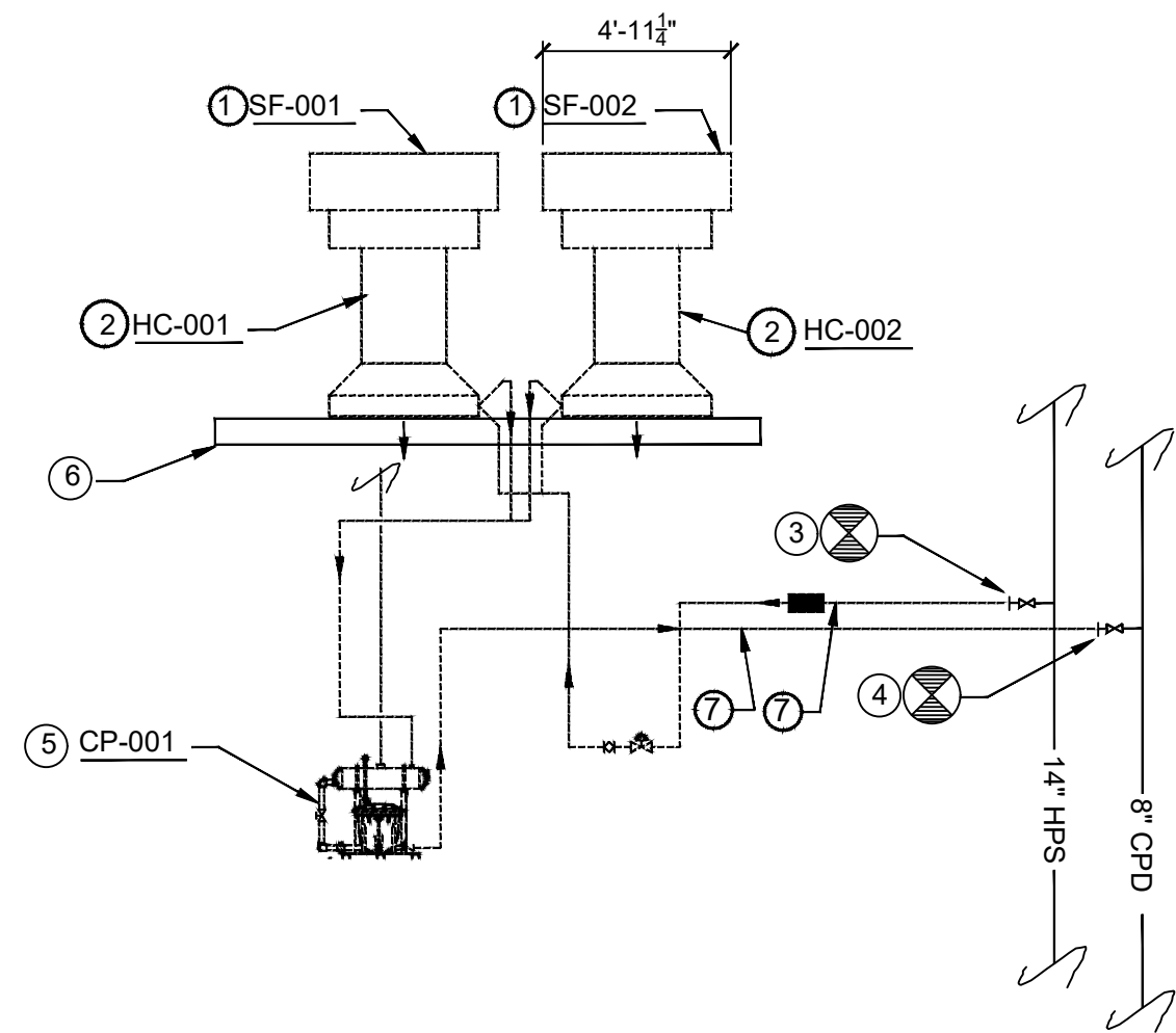
VENTILATION AND STEAM SYSTEM DEMOLITION
