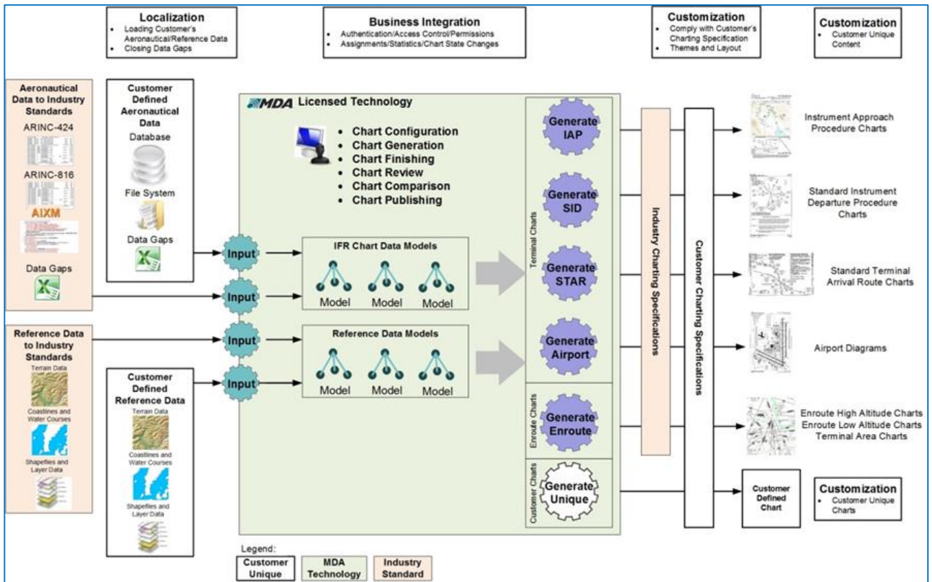
Figure 2: A sample ACE architecture.
