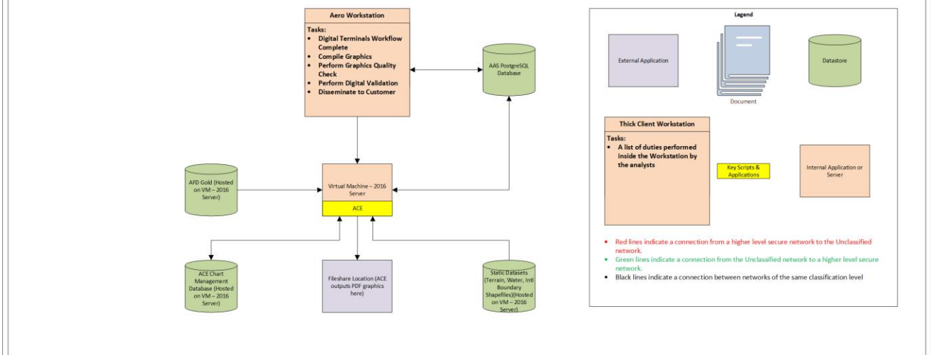
Figure 3: SFA As-Is Architecture Diagram.
