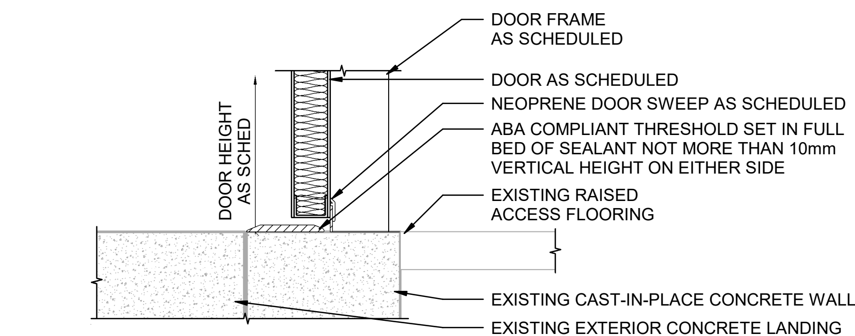
A1 SILL DETAIL AT EXISTING CONCRETE WALL 1:5
