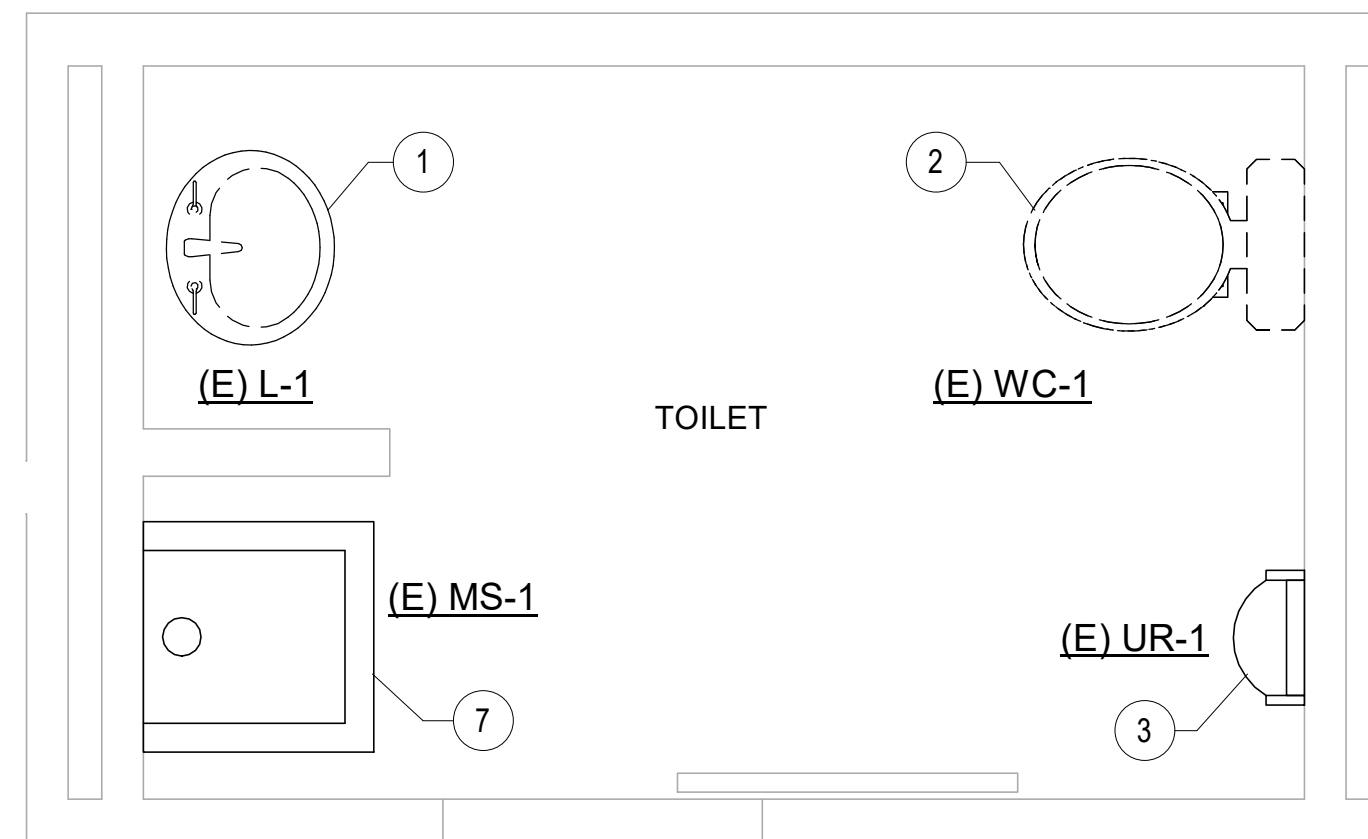
ENLARGED PLUMBING DEMOLITION PLAN - AREA B
