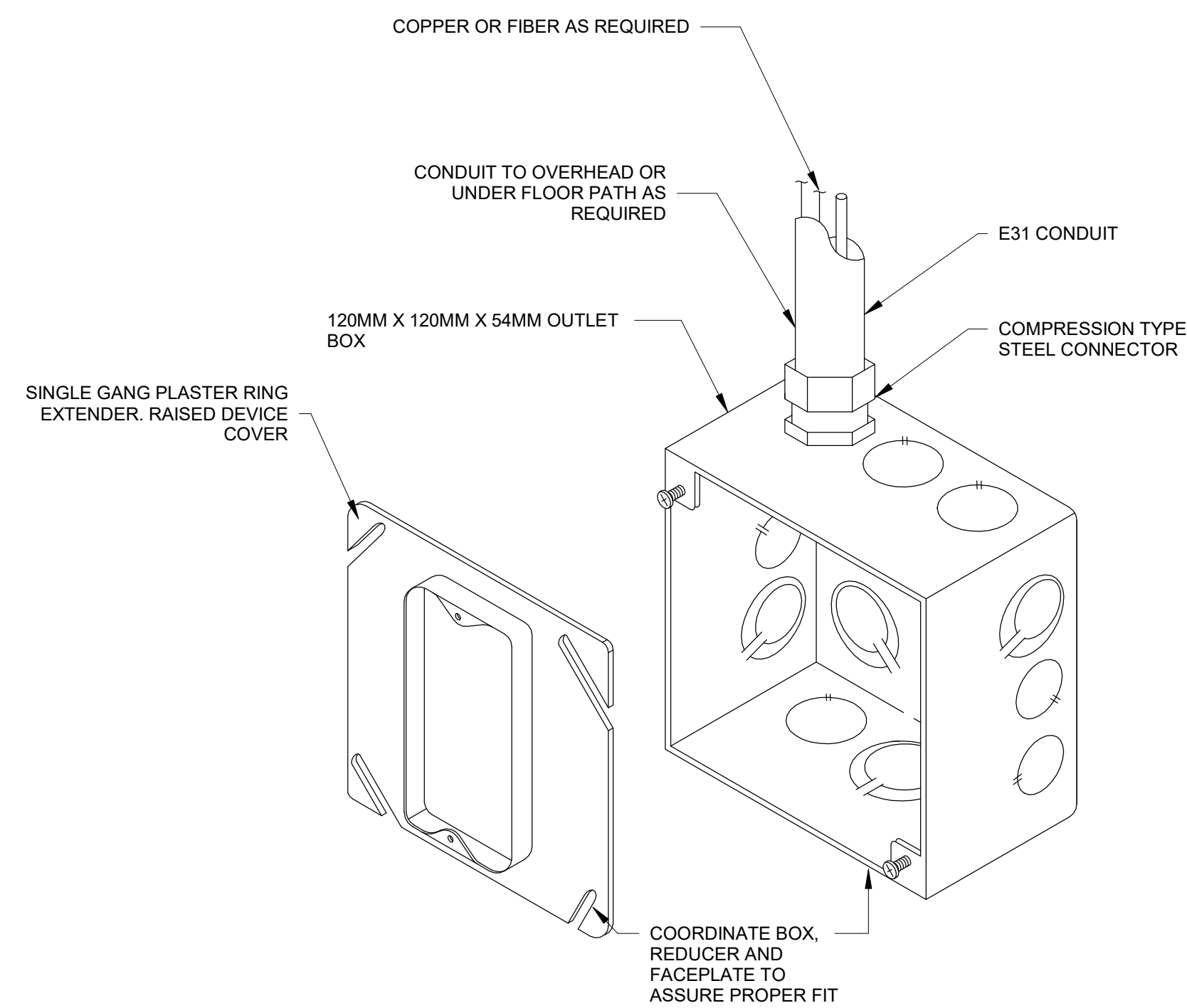
A1 WALL-MOUNTED OUTLET BOX DETAIL
