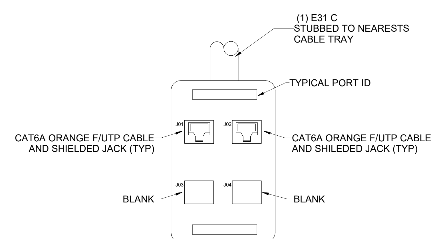
E8 TYPICAL 2-CAT6 "2S", DATA FACE PLATE (SECURE)
