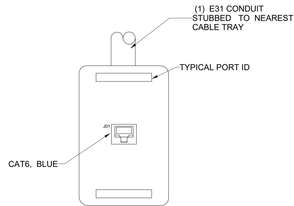
TYPICAL 1-CAT6 "1N" DATA FACE PLATE (UNSECURED)
