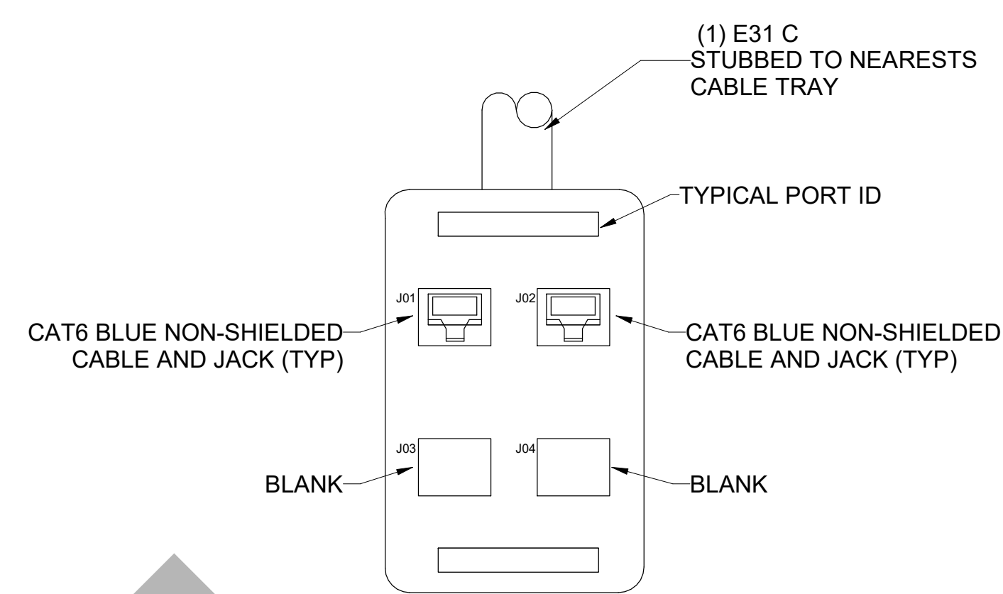
E4 TYPICAL 2-CAT6 "2N", DATA FACE PLATE (UNSECURE)
