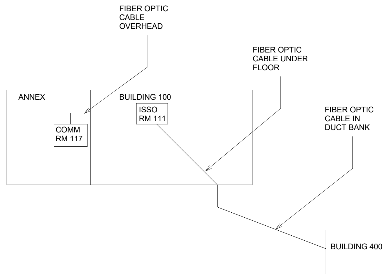
A1 FIBER RISER DIAGRAM (E) - PHASING
