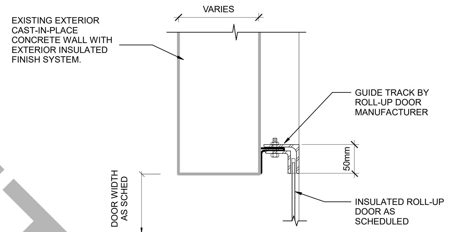
C7 OVERHEAD COILING DOOR JAMB DETAIL 1:5
