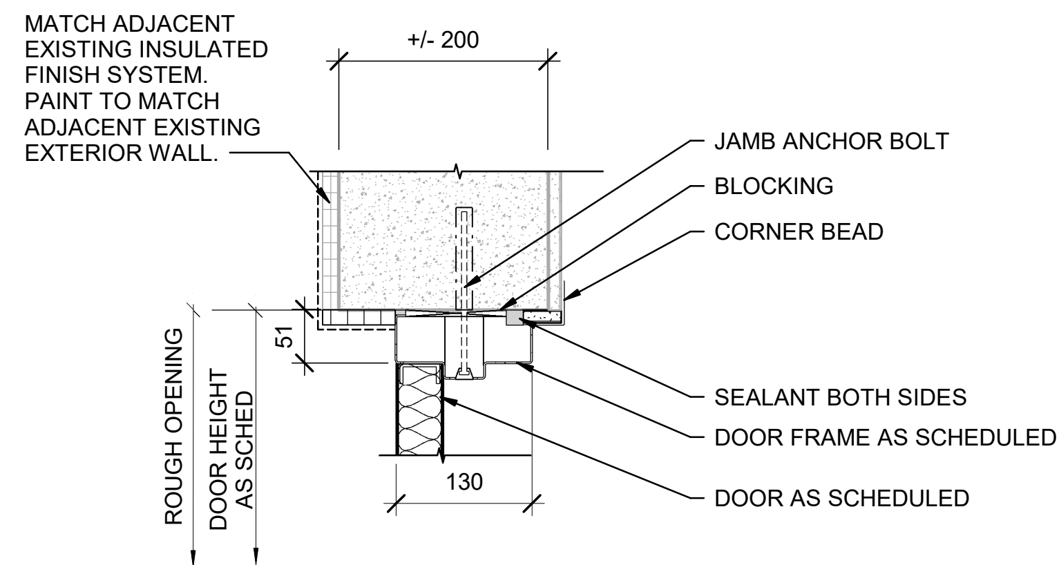
B1 JAMB DETAIL AT EXISTING CONCRETE WALL 1:5
