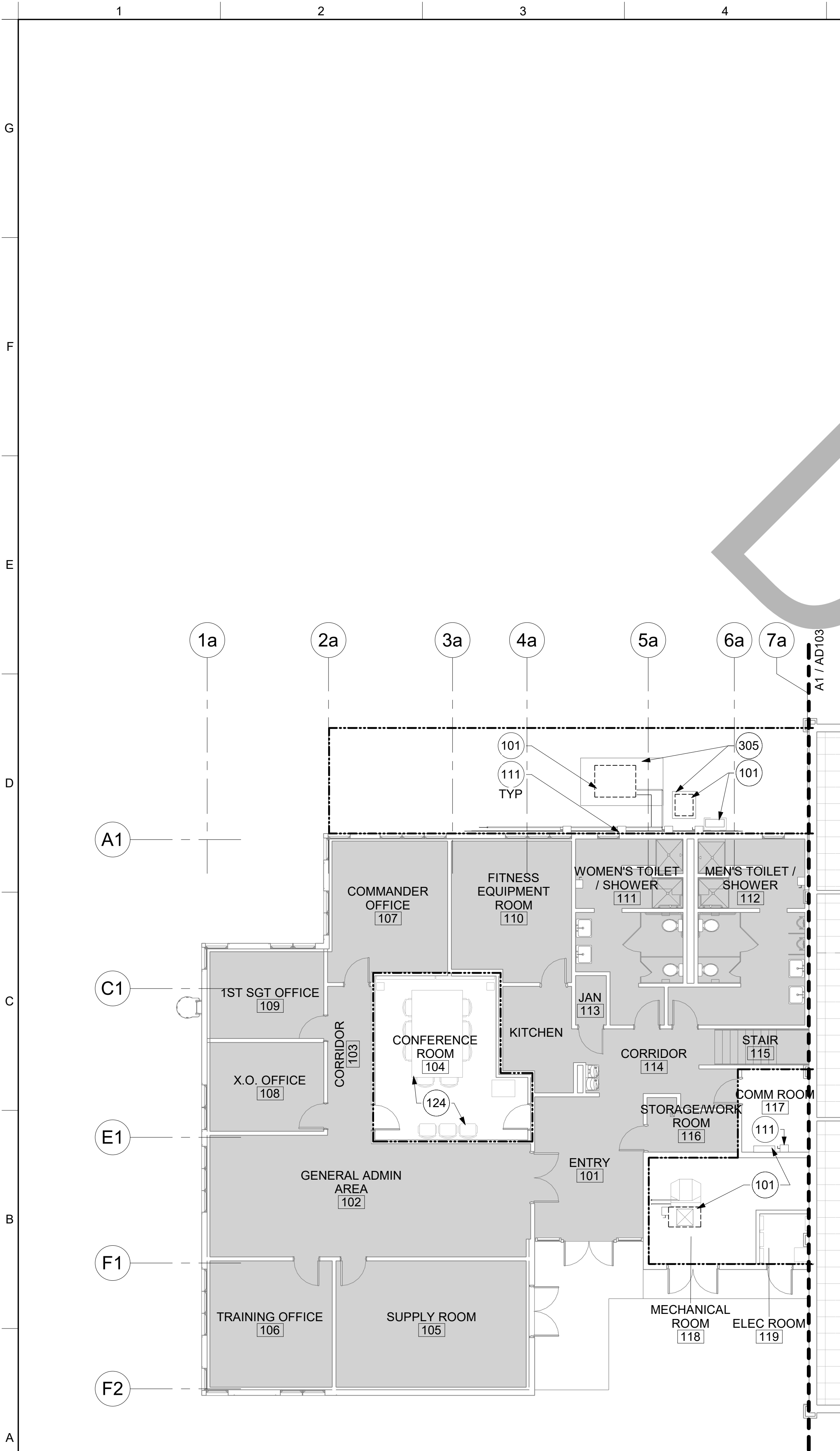
A1 PARTIAL DEMOLITION FLOOR PLAN - AREA A 1 : 100
