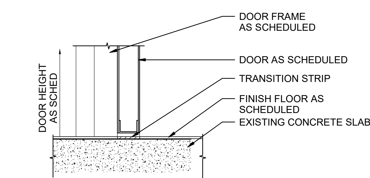
A4 SILL DETAIL AT METAL STUD WALL 1:5
