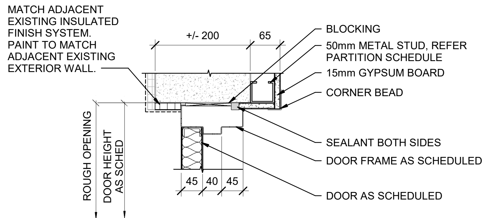
D1 HEAD DETAIL AT EXISTING CONCRETE WALL 1:5
