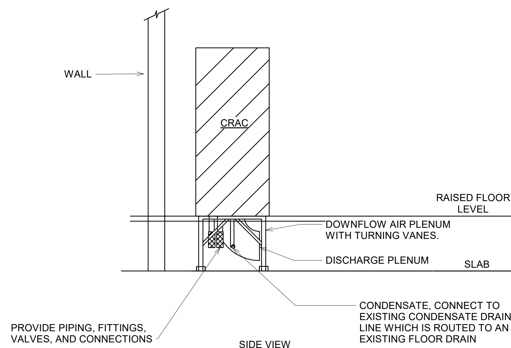
E1 TYPICAL CRAC DETAIL (DOWNFLOW) NTS
