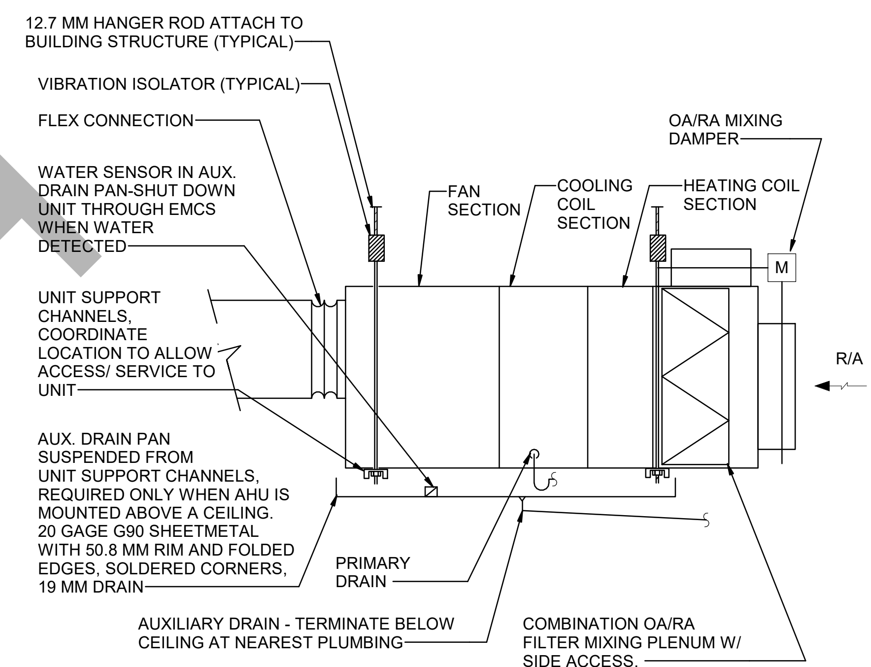
A8 FCU MOUNTING DETAIL
