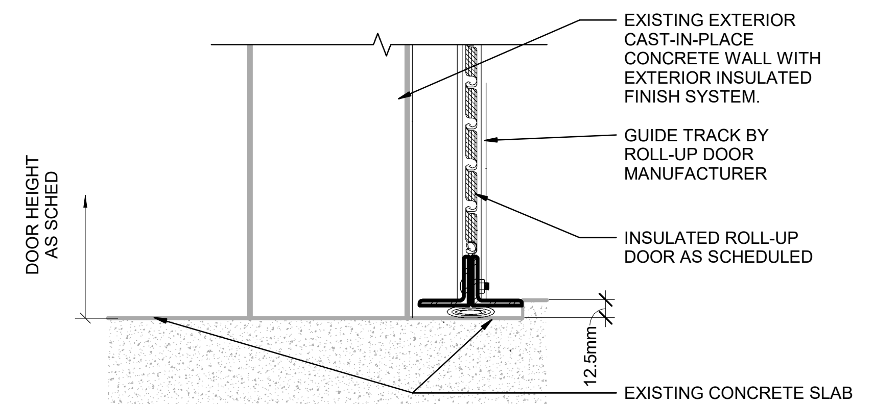
A7 OVERHEAD COILING DOOR SILL DETAIL 1:5
