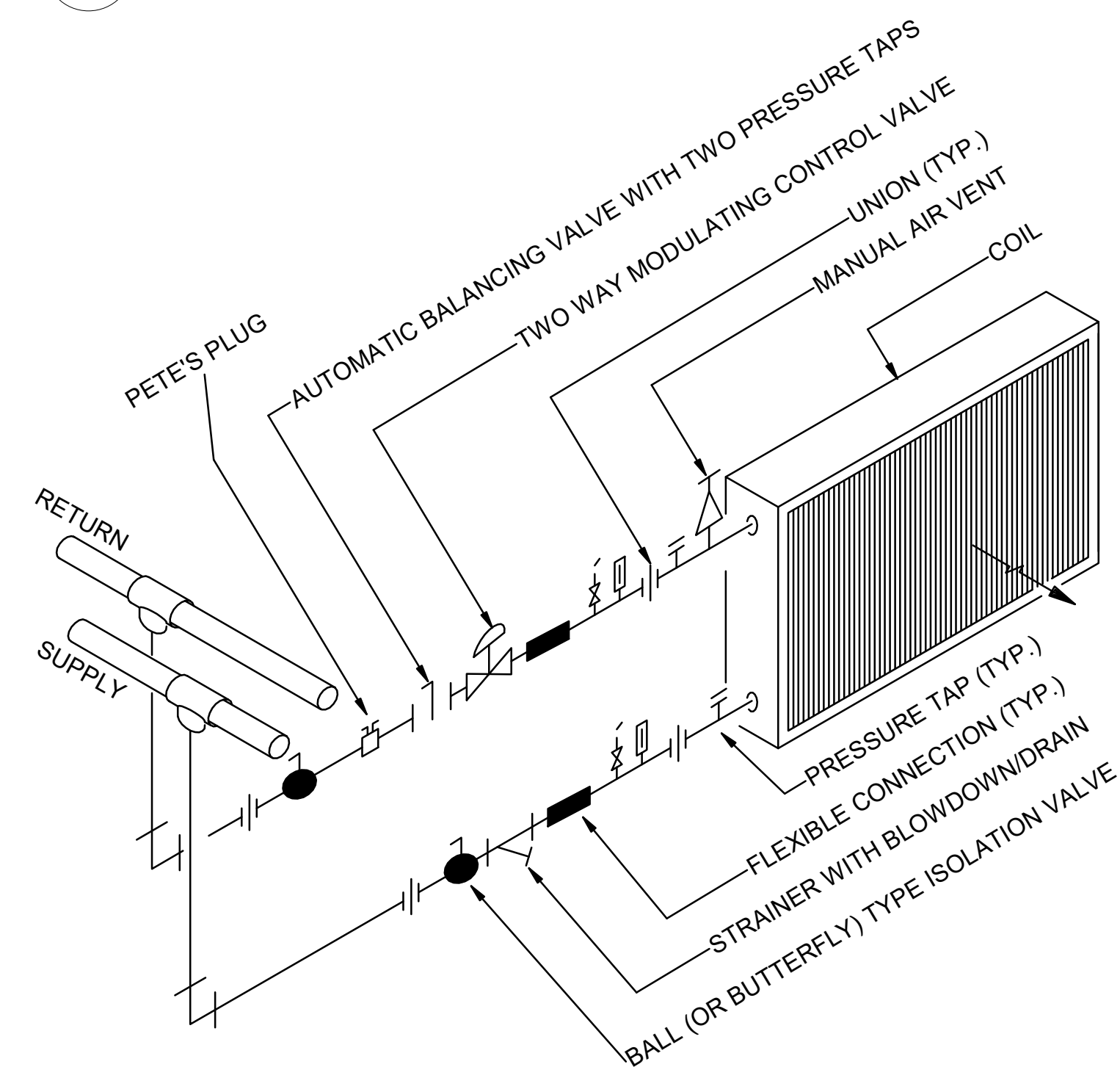
WATER COIL PIPING (TWO-WAY VALVE SINGLE COIL)
