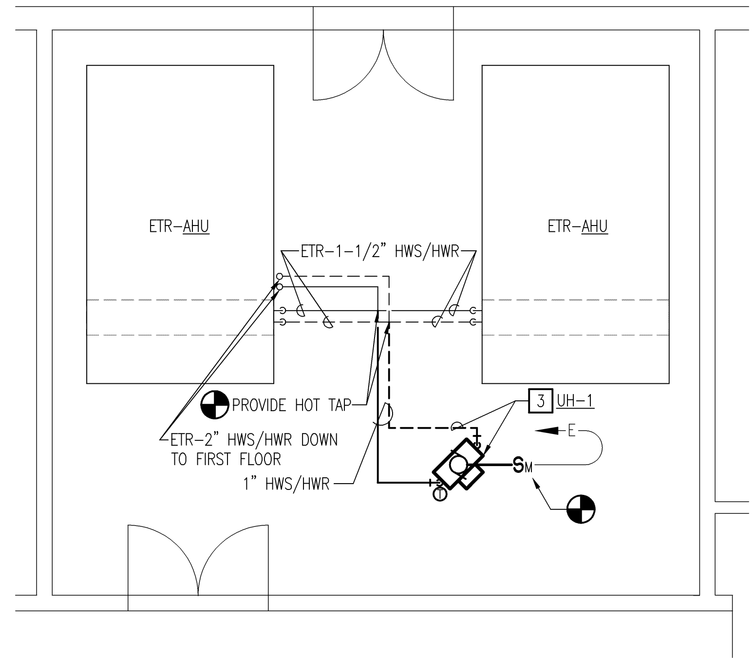
MECH./ELEC. NEW WORK PLAN - SECOND FLOOR SCALE: 1/4" = 1'-0"
