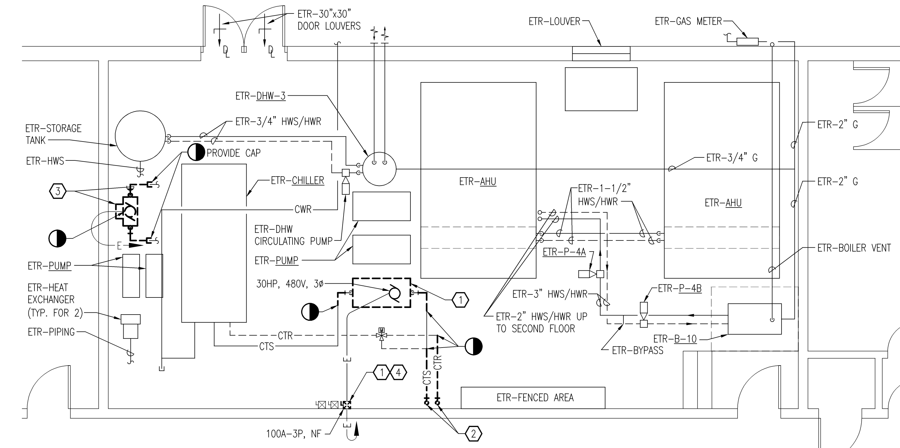
MECHANICAL/ELECTRICAL DEMOLITION PLAN - FIRST FLOOR SCALE: 1/4" = 1'-0"
