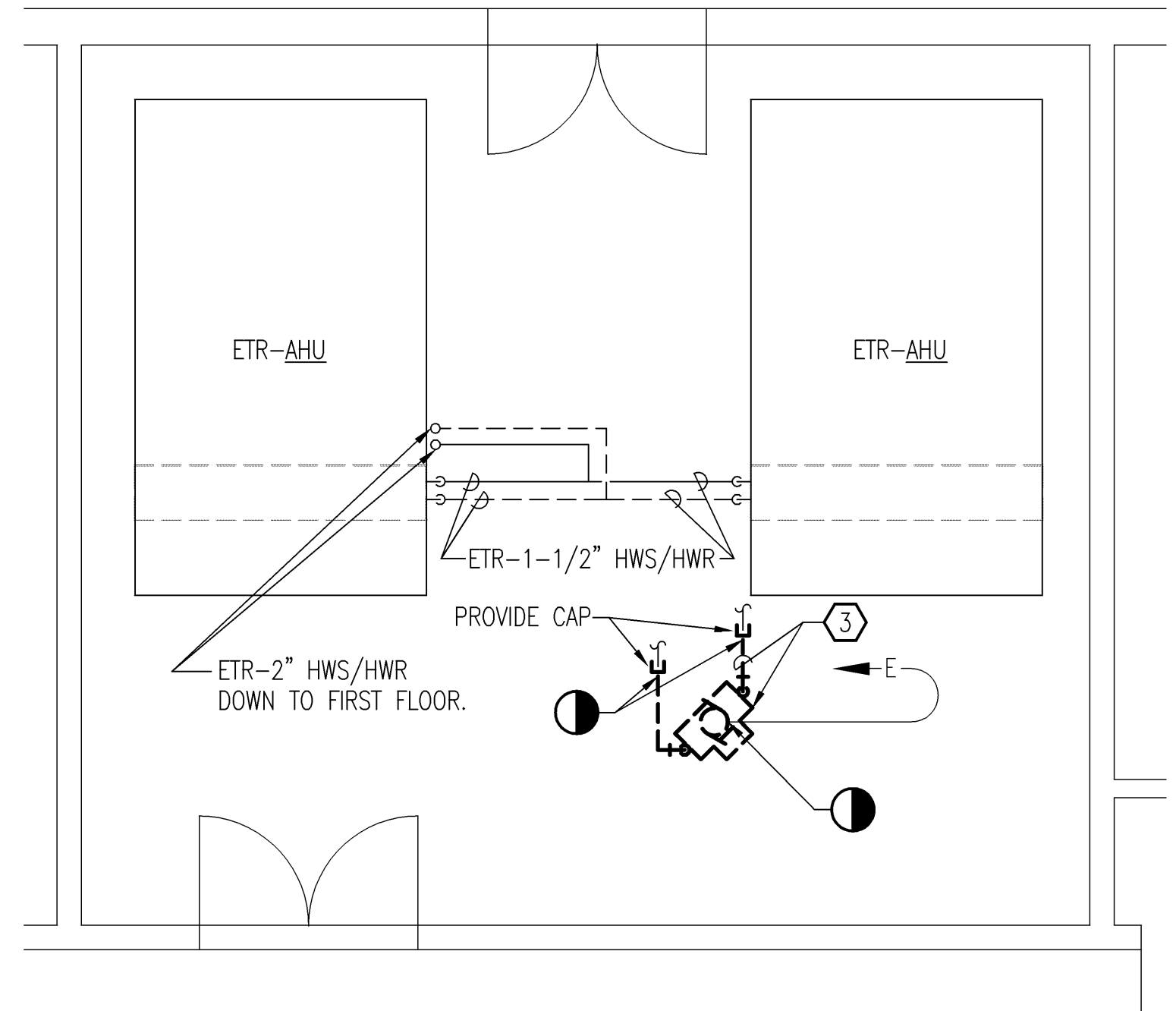
MECH./ELEC. DEMOLITION PLAN - SECOND FLOOR SCALE: 1/4" = 1'-0"
