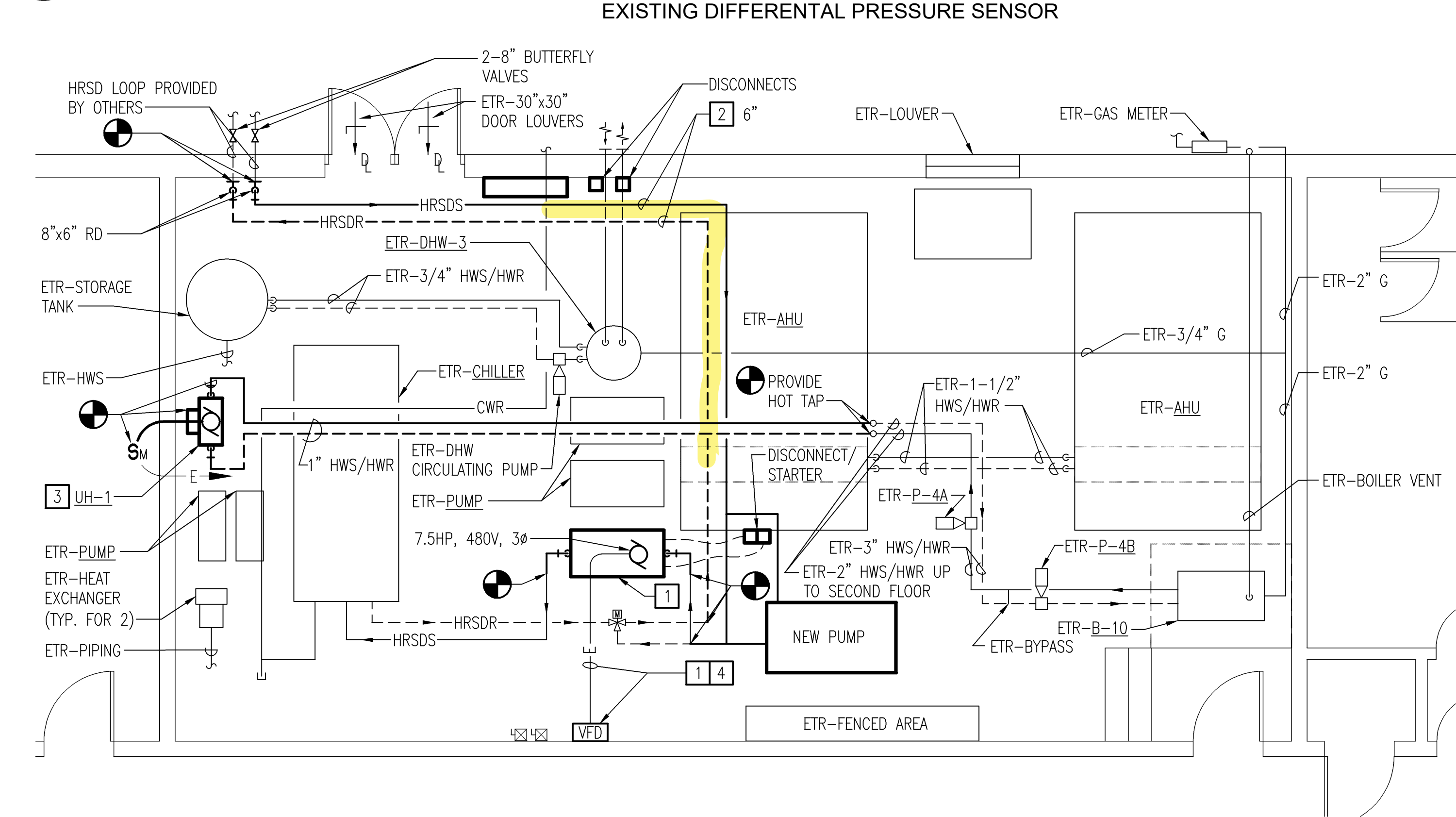
MECHANICAL/ELECTRICAL NEW WORK PLAN - FIRST FLOOR SCALE: 1/4" = 1'-0"
