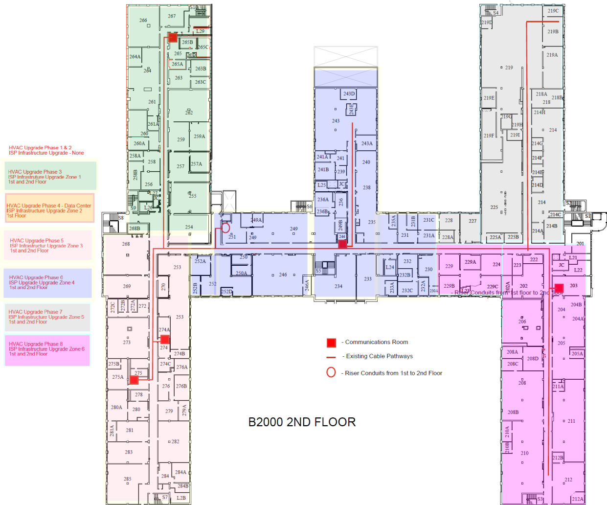
FIGURE 2 B2000 2 nd Floor Layout Communication Room Location and Cable Pathways
