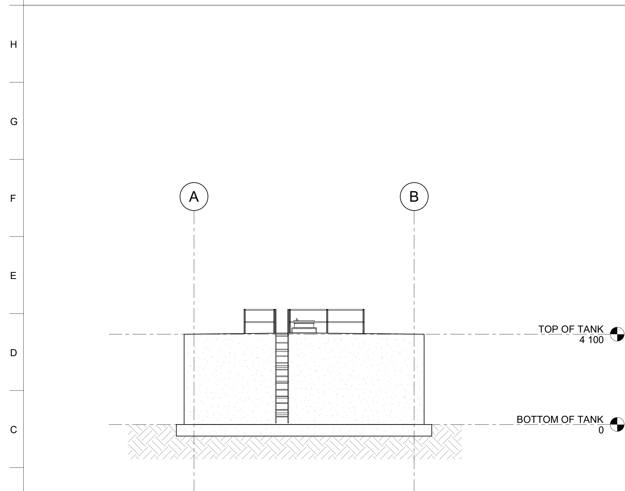
11 WT - EXTERIOR ELEVATION EAST (CLIN 0001) SCALE 1 : 100
