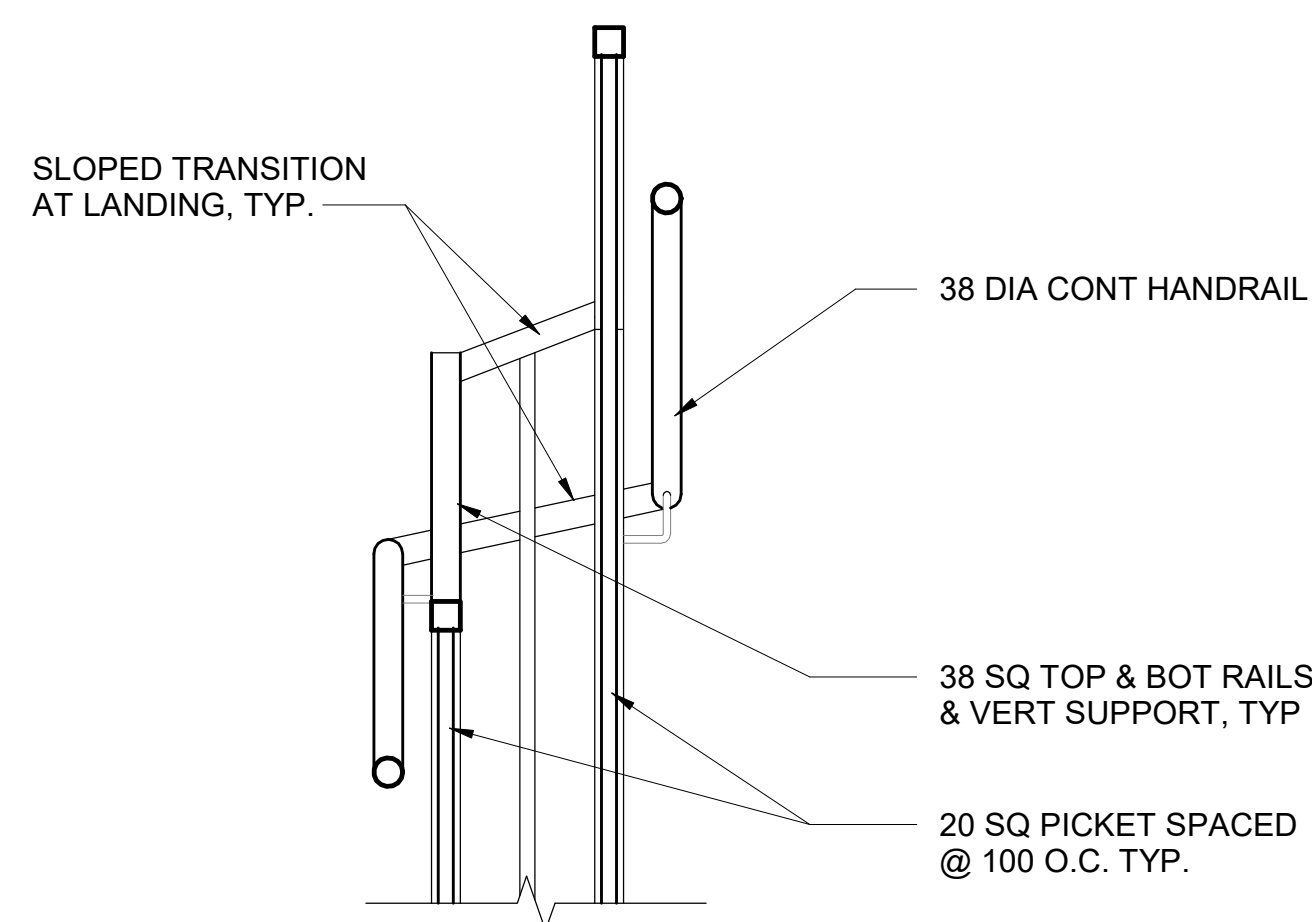
B1 RAILING TRANSITION AT LANDING
