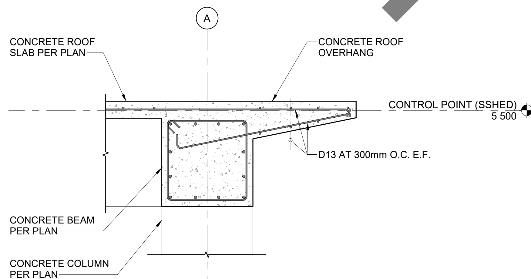
A9 OVERHANG DETAIL SCALE 1 : 20
