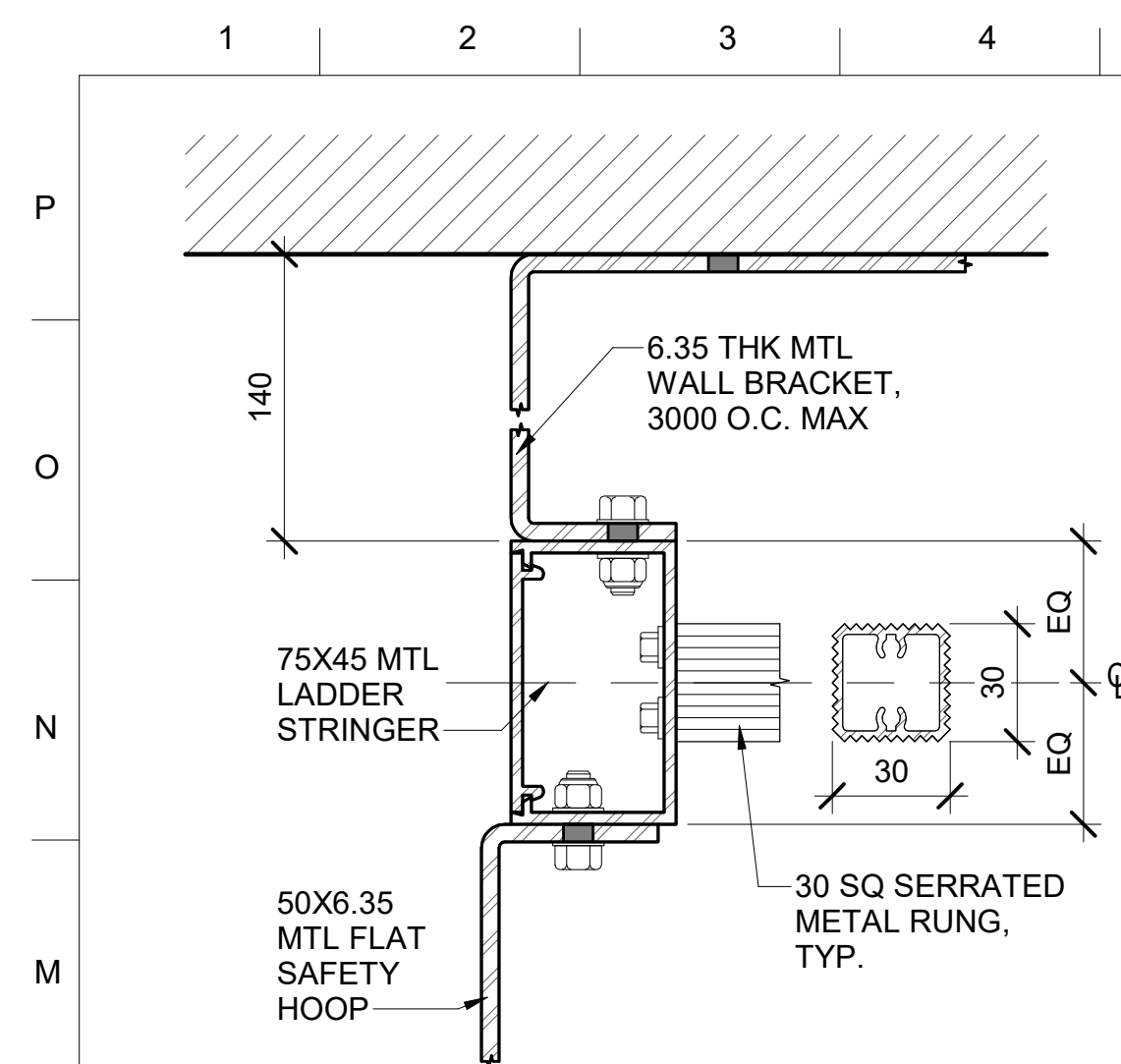
L1 CAGE LADDER TREAD
