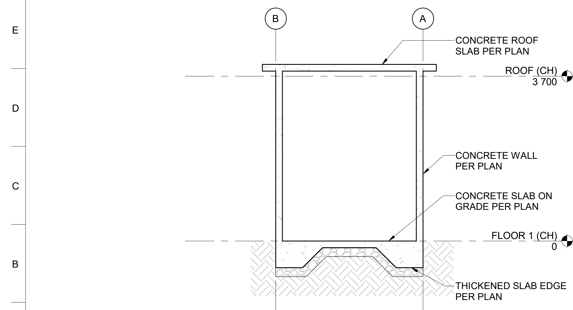
A1 CH - BUILDING SECTION (CLIN 0001) SCALE 1 : 50
