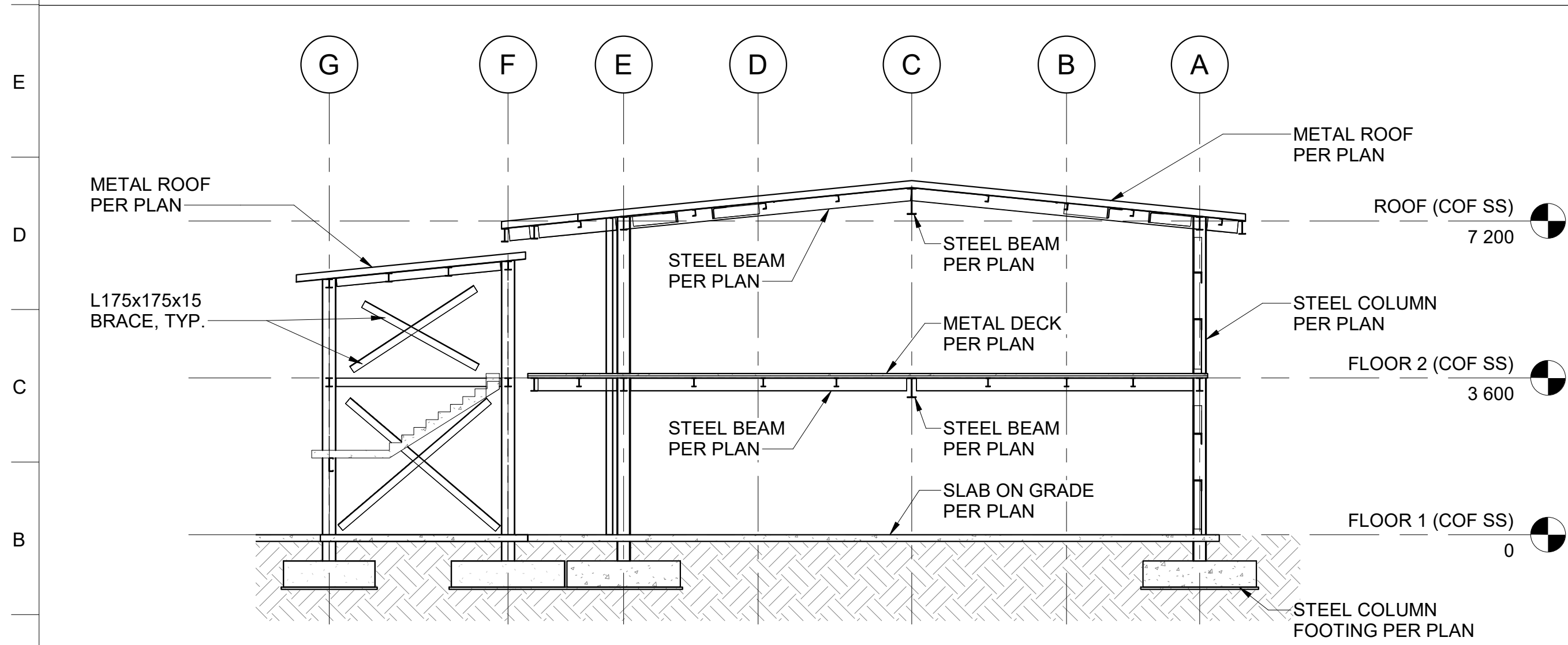
A1 COF SS - BUILDING SECTIONS (CLIN 0004) SCALE 1 : 100
