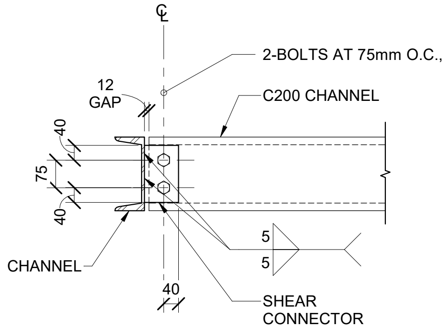
CHANNEL TO CHANNEL CONNECTION
