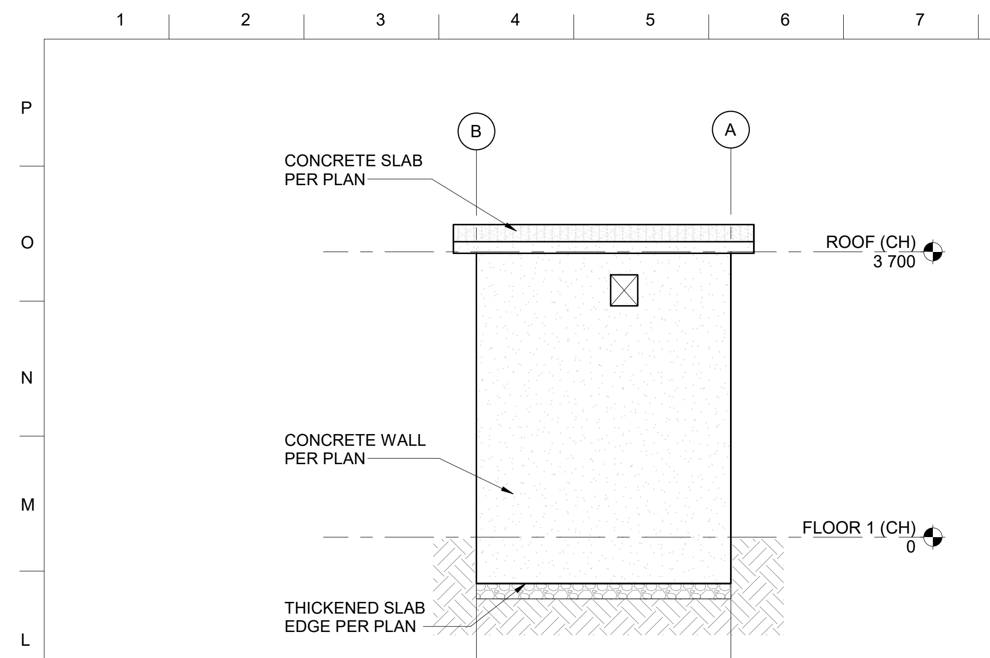
K1 CH - EXTERIOR ELEVATION - EAST (CLIN 0001) SCALE 1 : 50
