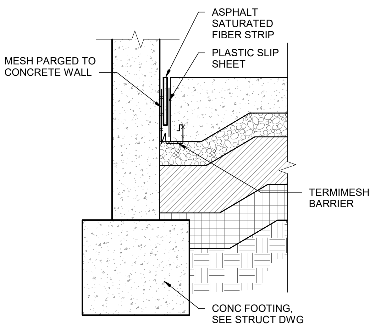
TERMITE MESH @ THICKENED SLAB EDGE DETAIL
