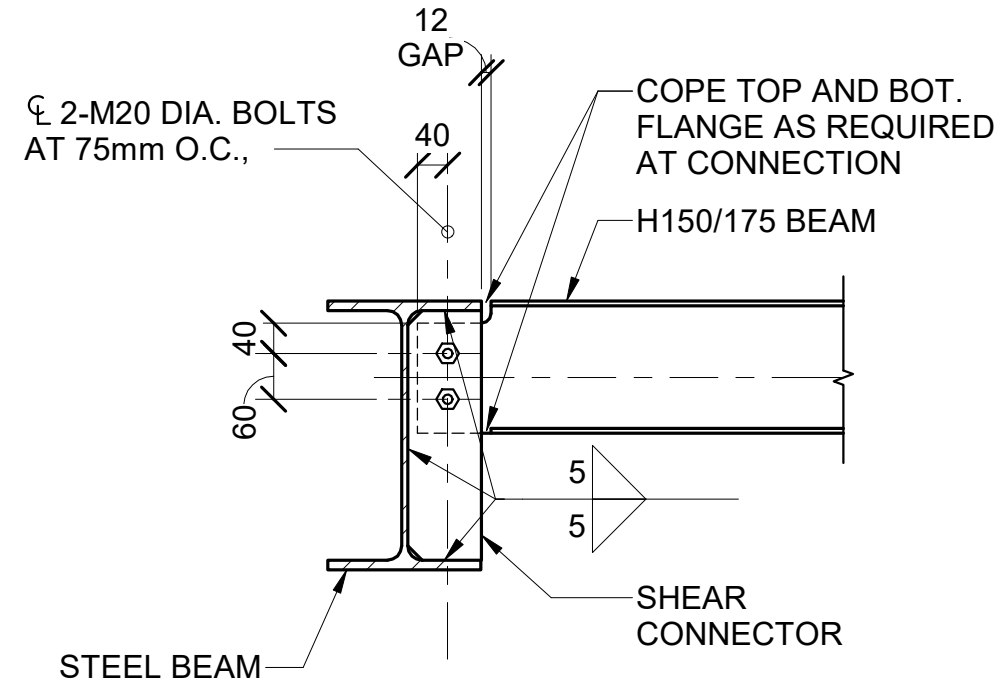
CONDITION AT H150 OR H175 BEAM
