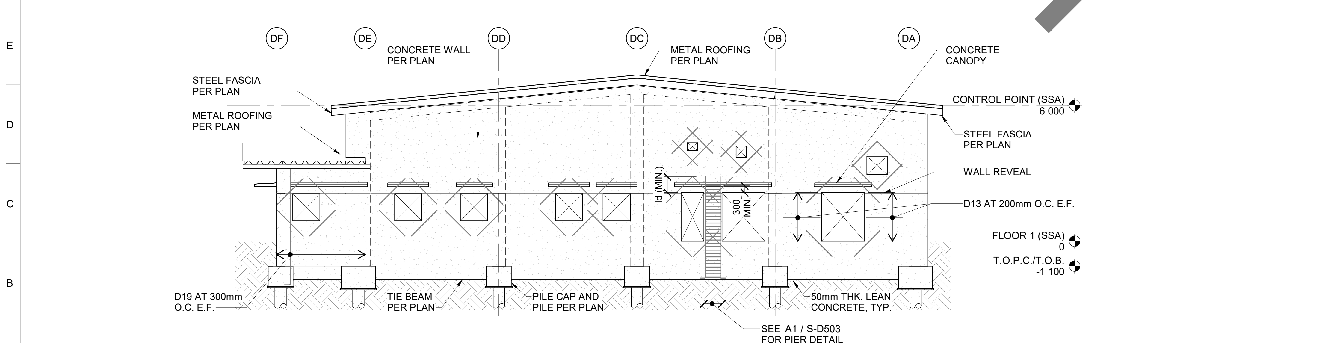
A1 SSAW - EXTERIOR ELEVATION - EAST (CLIN 0004) SCALE 1 : 100
