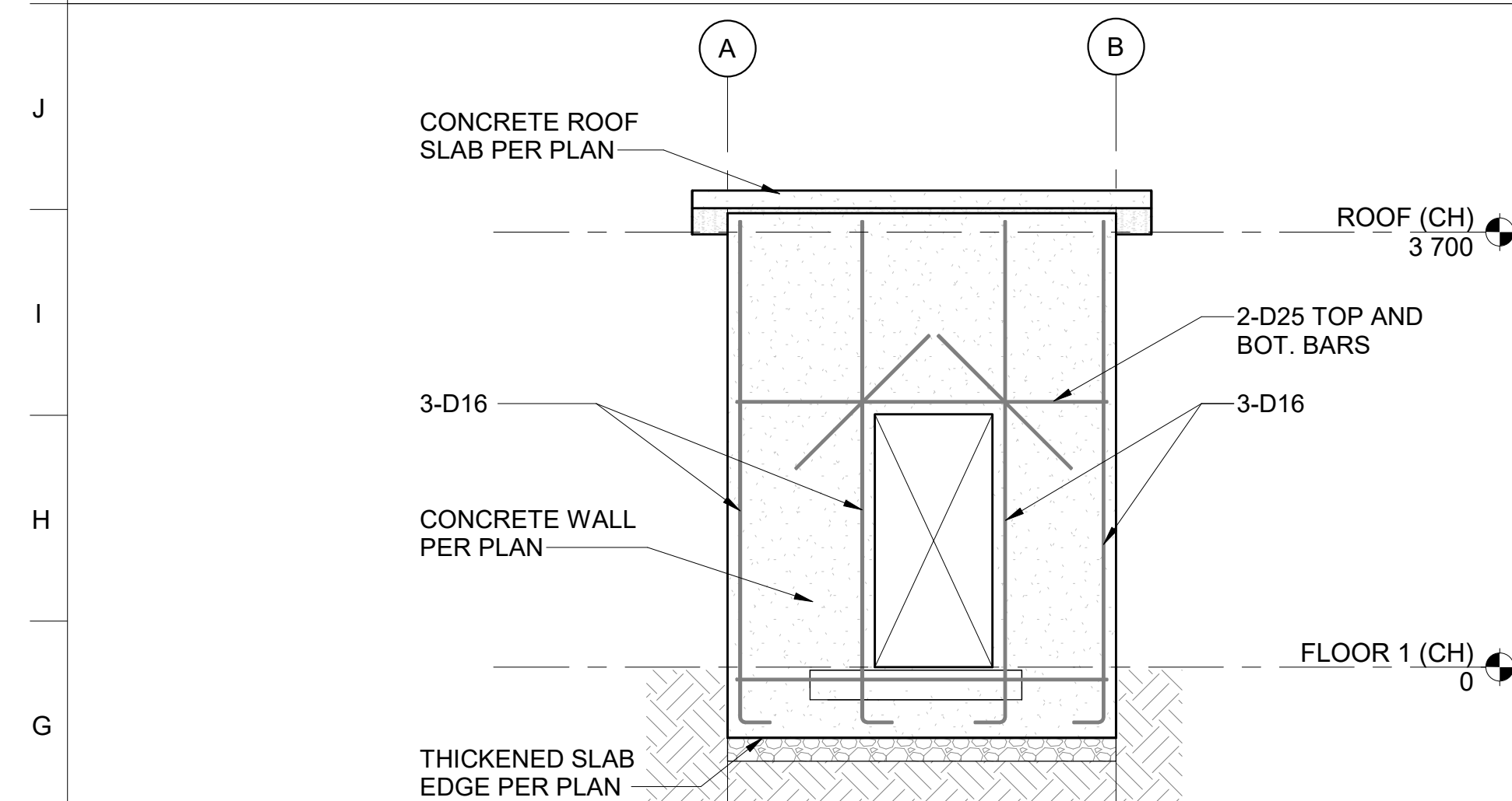
K1 CH - EXTERIOR ELEVATION - EAST (CLIN 0001) SCALE 1 : 50
