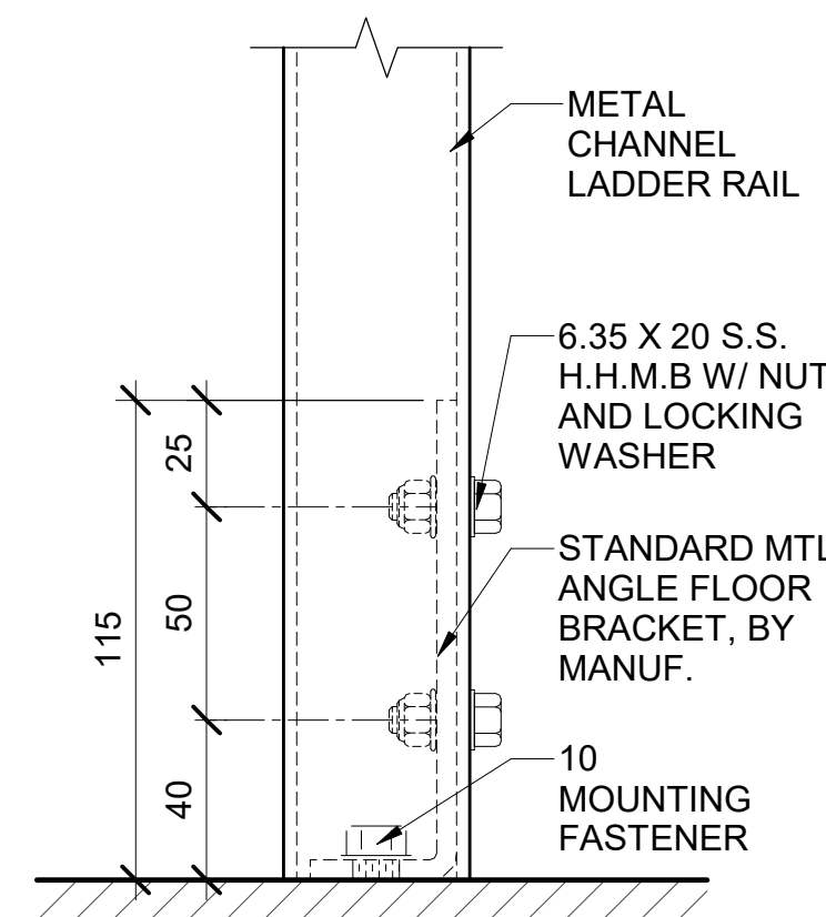
L8 FLOOR MOUNT BRACKET
