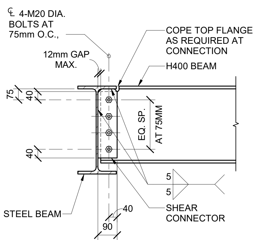
CONDITION AT H400 BEAM
