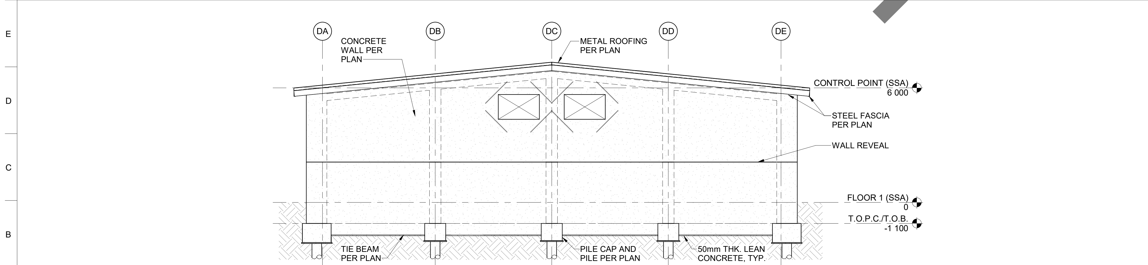
A1 SSAW - EXTERIOR ELEVATION - WEST (CLIN 0004) SCALE 1 : 100
