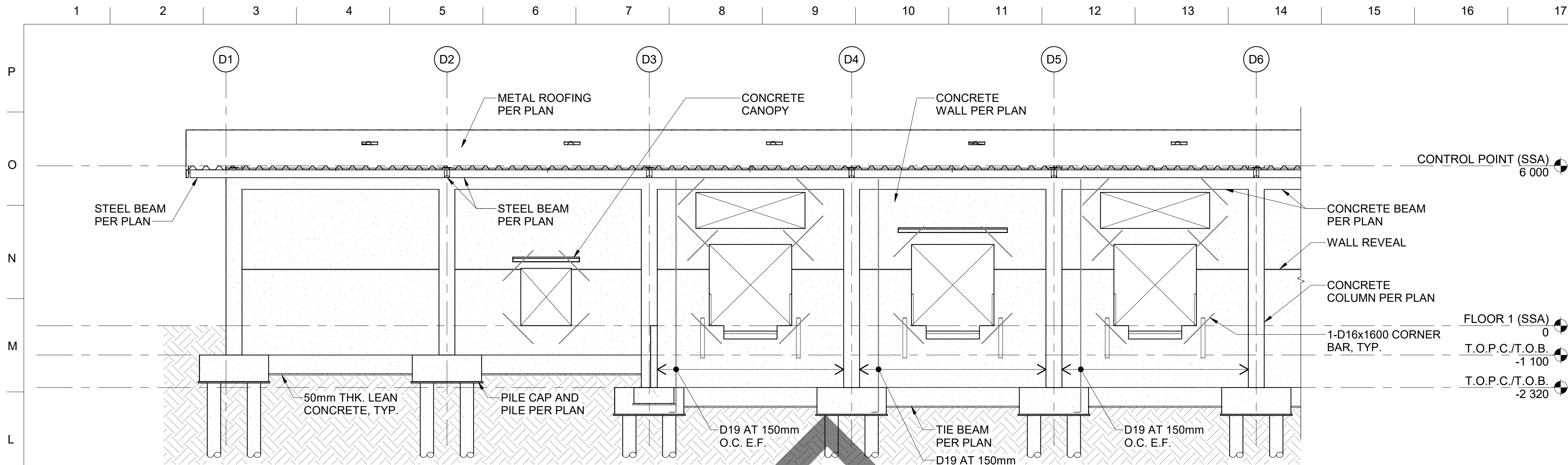
K1 SSAW - PARTIAL EXTERIOR ELEVATION - SOUTH (WEST) (CLIN 0004) SCALE 1 : 100
