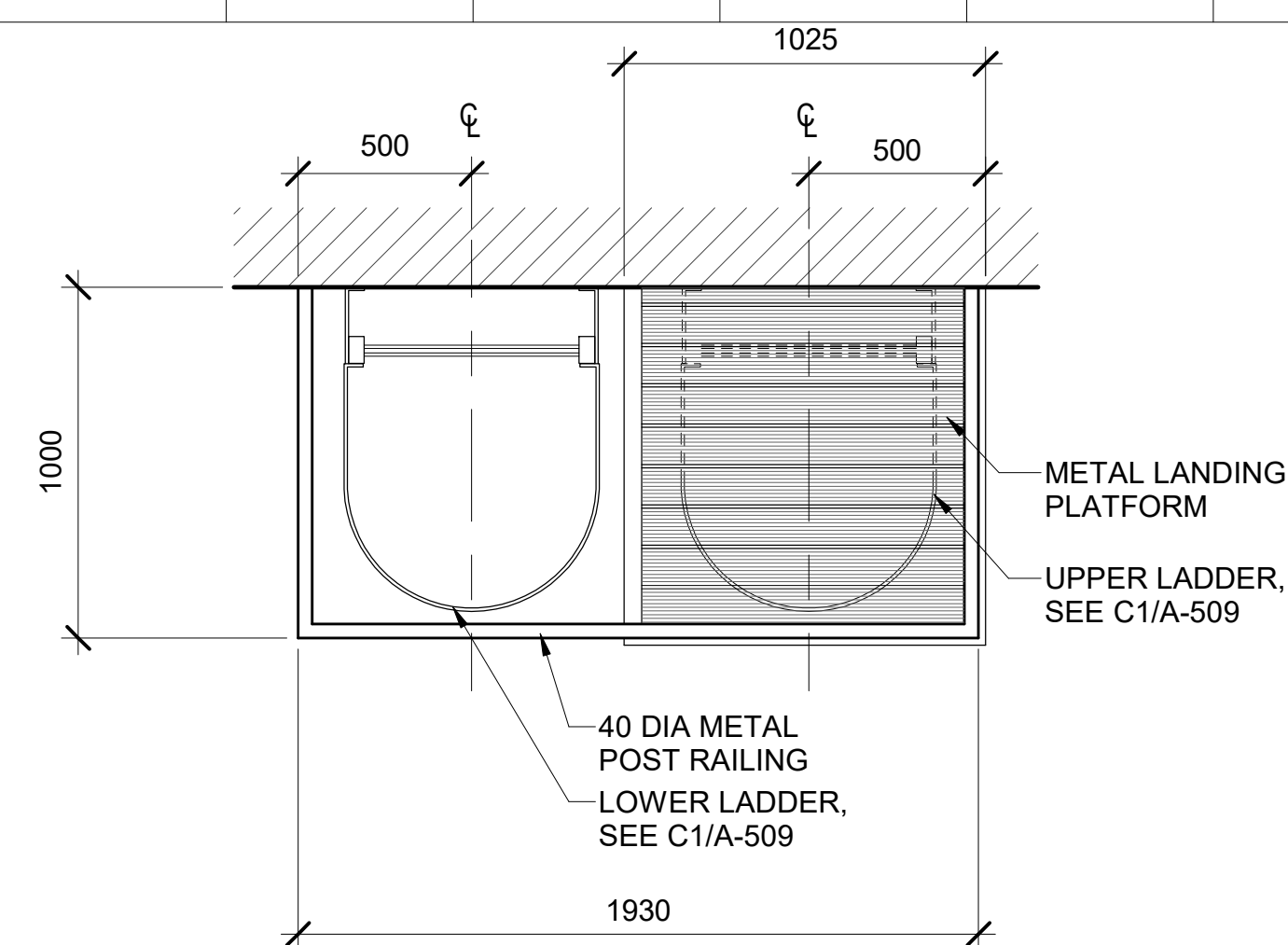
L9 REST PLATFORM PLAN 1 : 20
