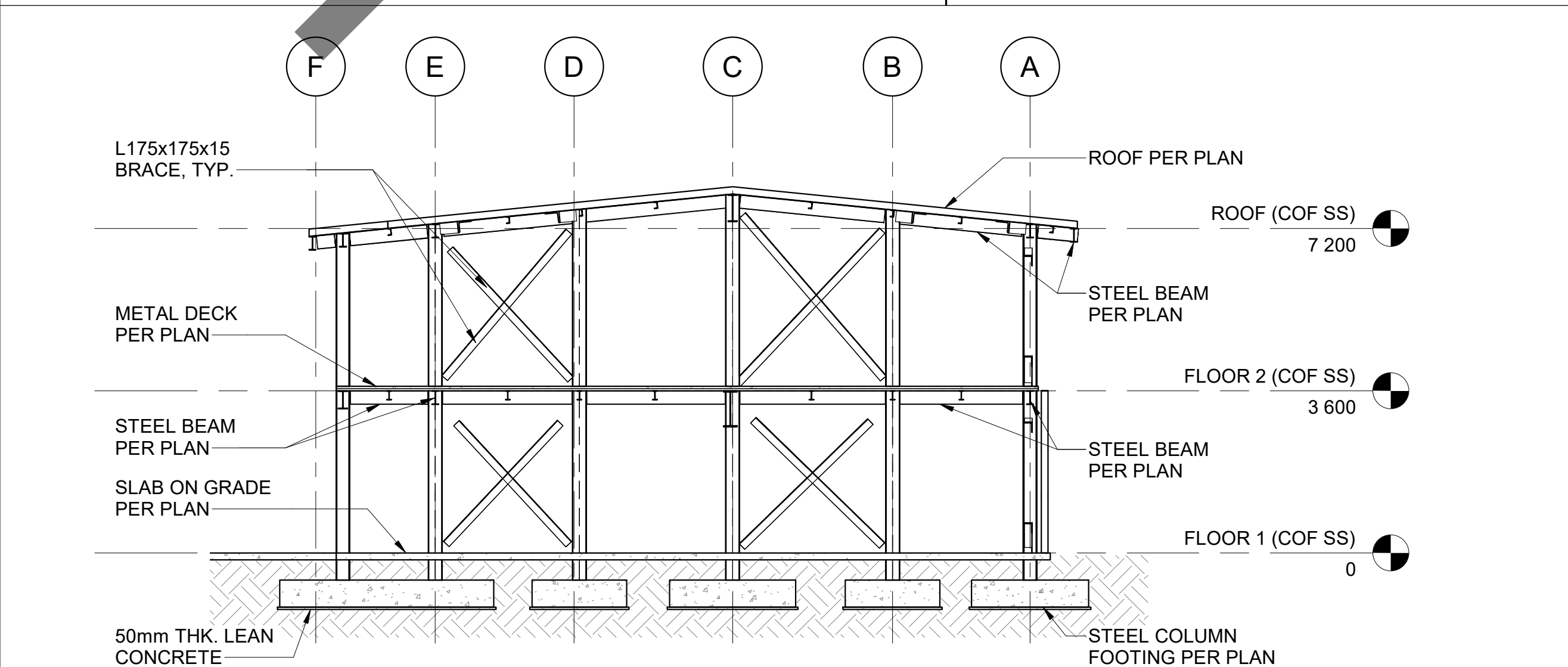
A12 COF SS - BUILDING SECTIONS (CLIN 0004) SCALE 1 : 100
