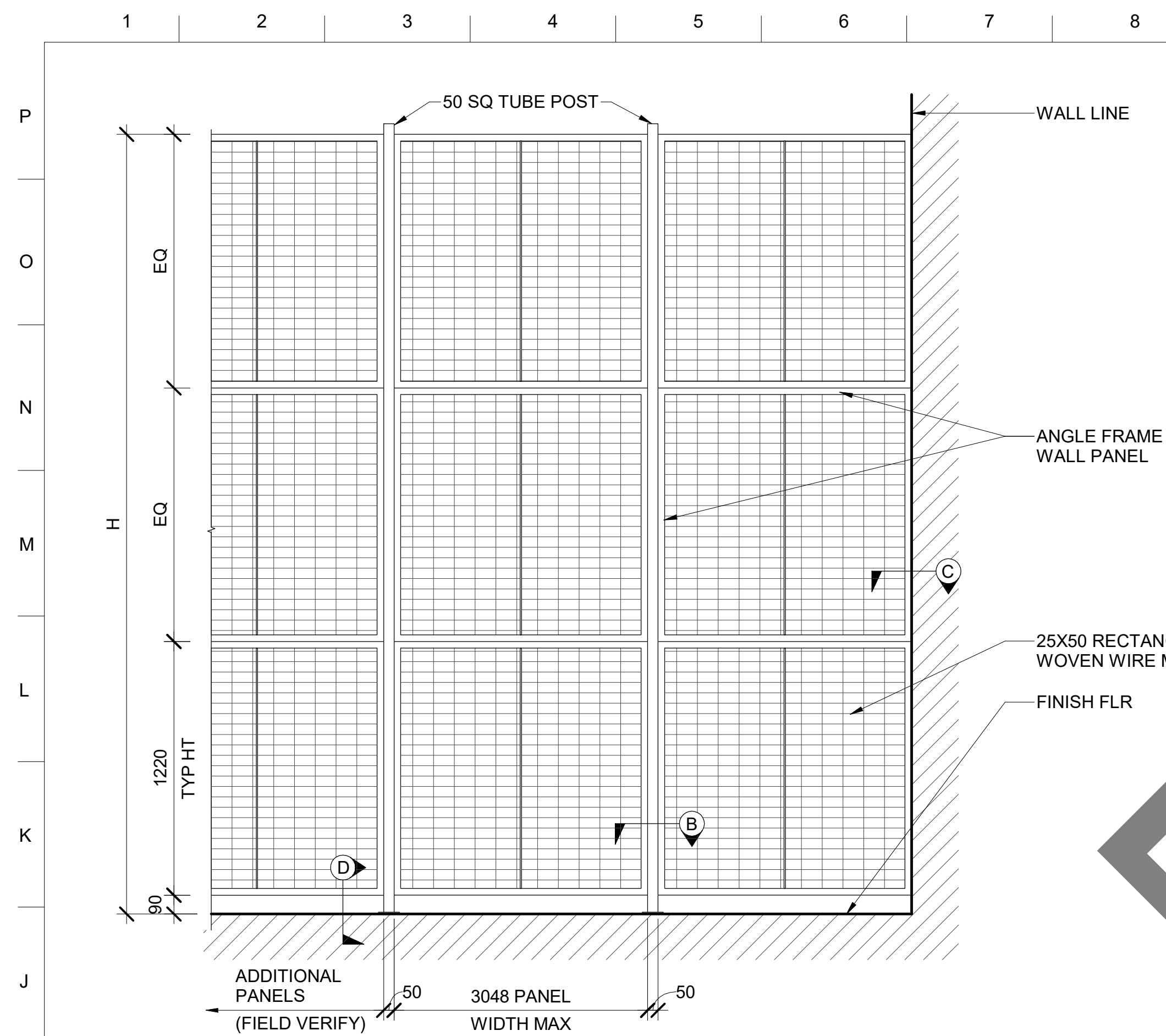
11 WIRE MESH PARTITION ELEVATION
