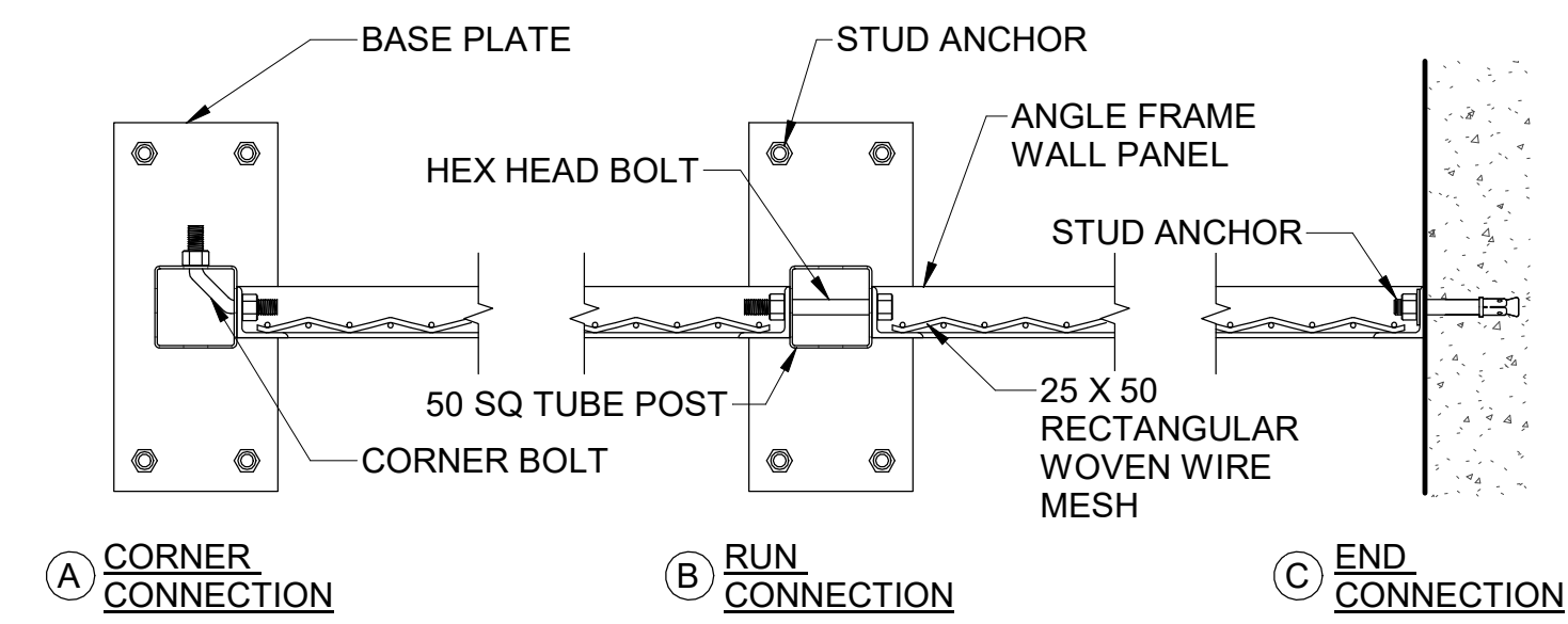
(M9) WIRE MESH PARTITION DETAIL 1:5
