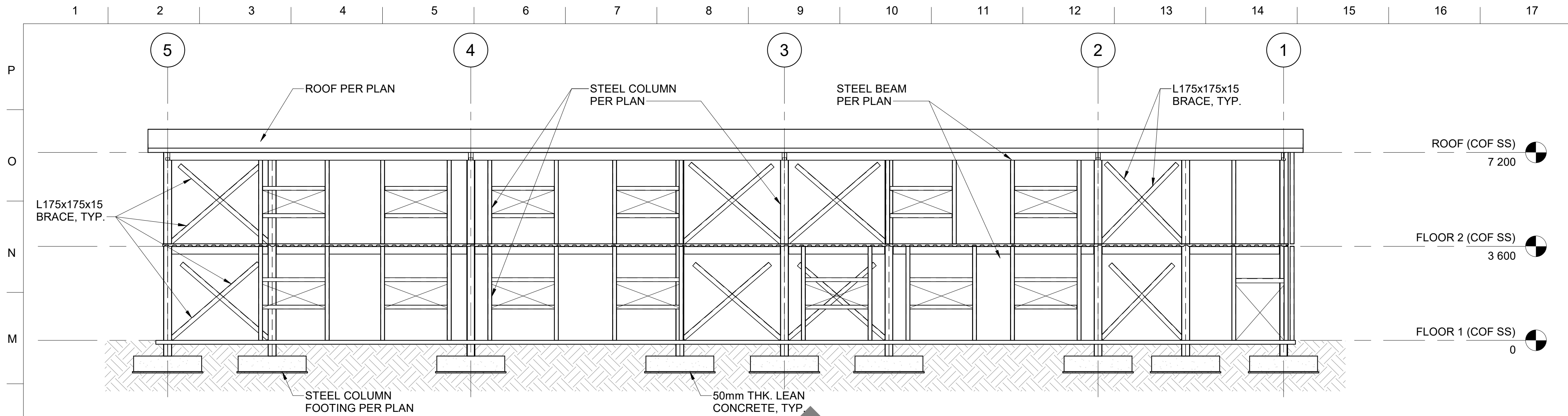
L1 COF SS - EXTERIOR ELEVATION NORTH (CLIN 0004) SCALE 1 : 100
