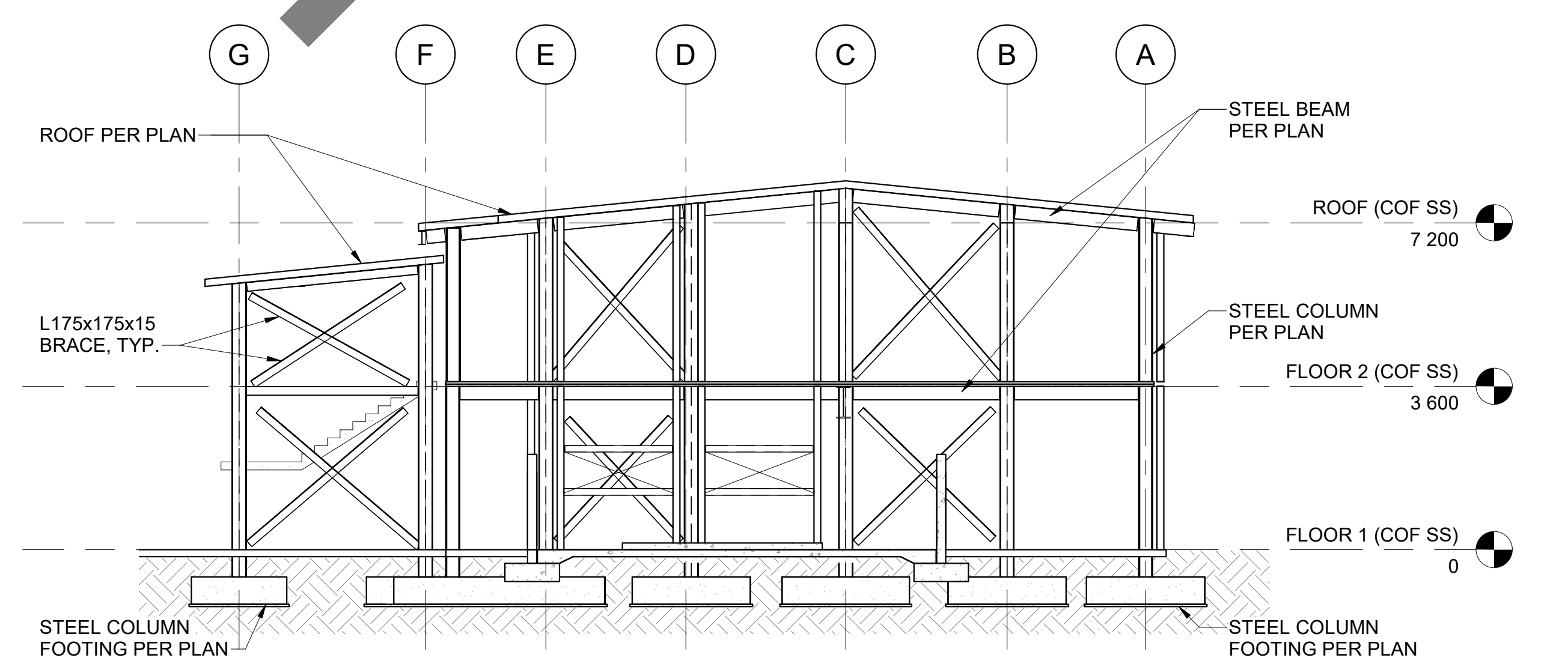
A12 COF SS - EXTERIOR ELEVATION EAST (CLIN 0004) SCALE 1 : 100
