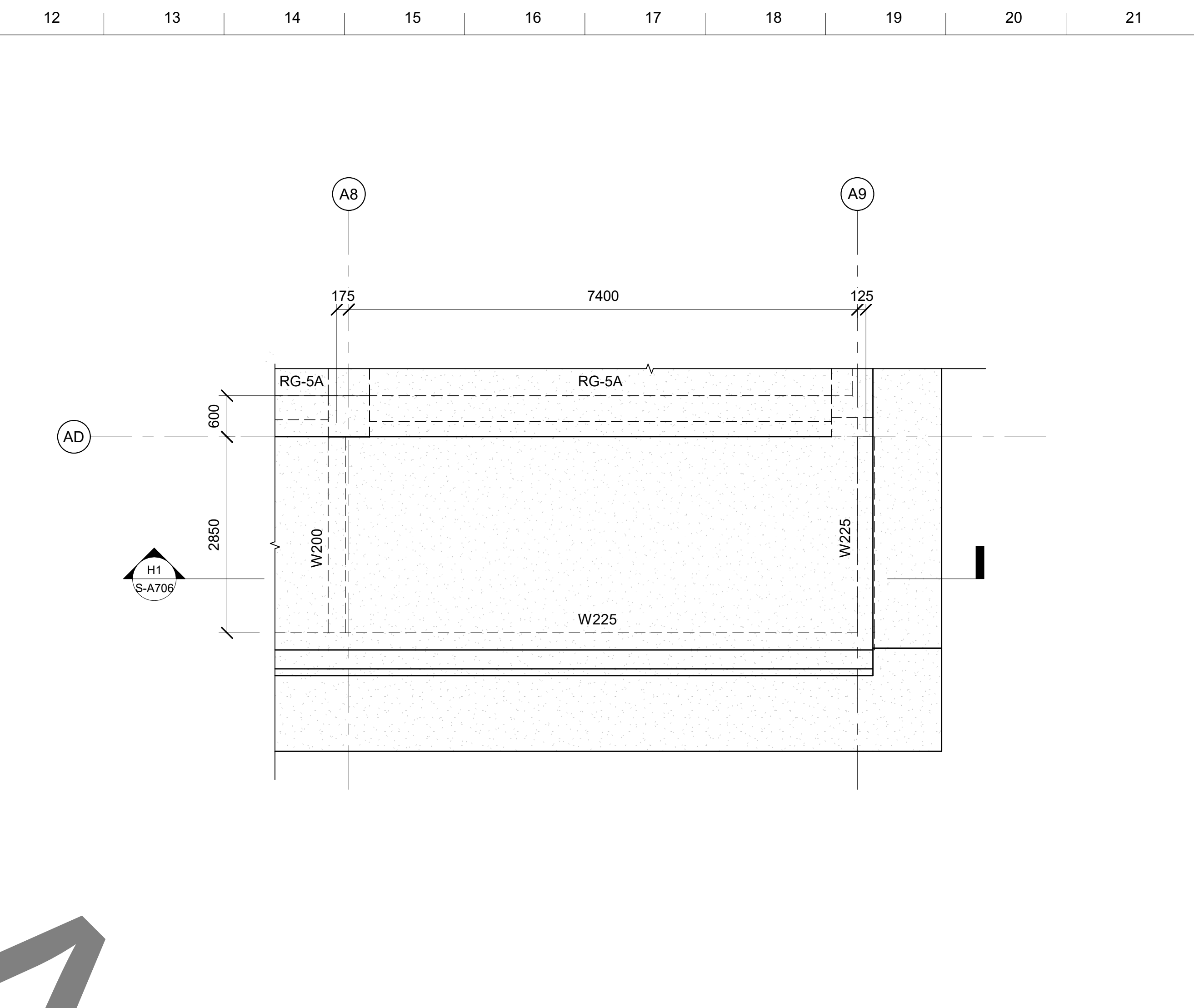
H12 VMS - STAIR 2 ROOF FRAMING PLAN PLAN (CLIN 0001) SCALE 1 : 50
