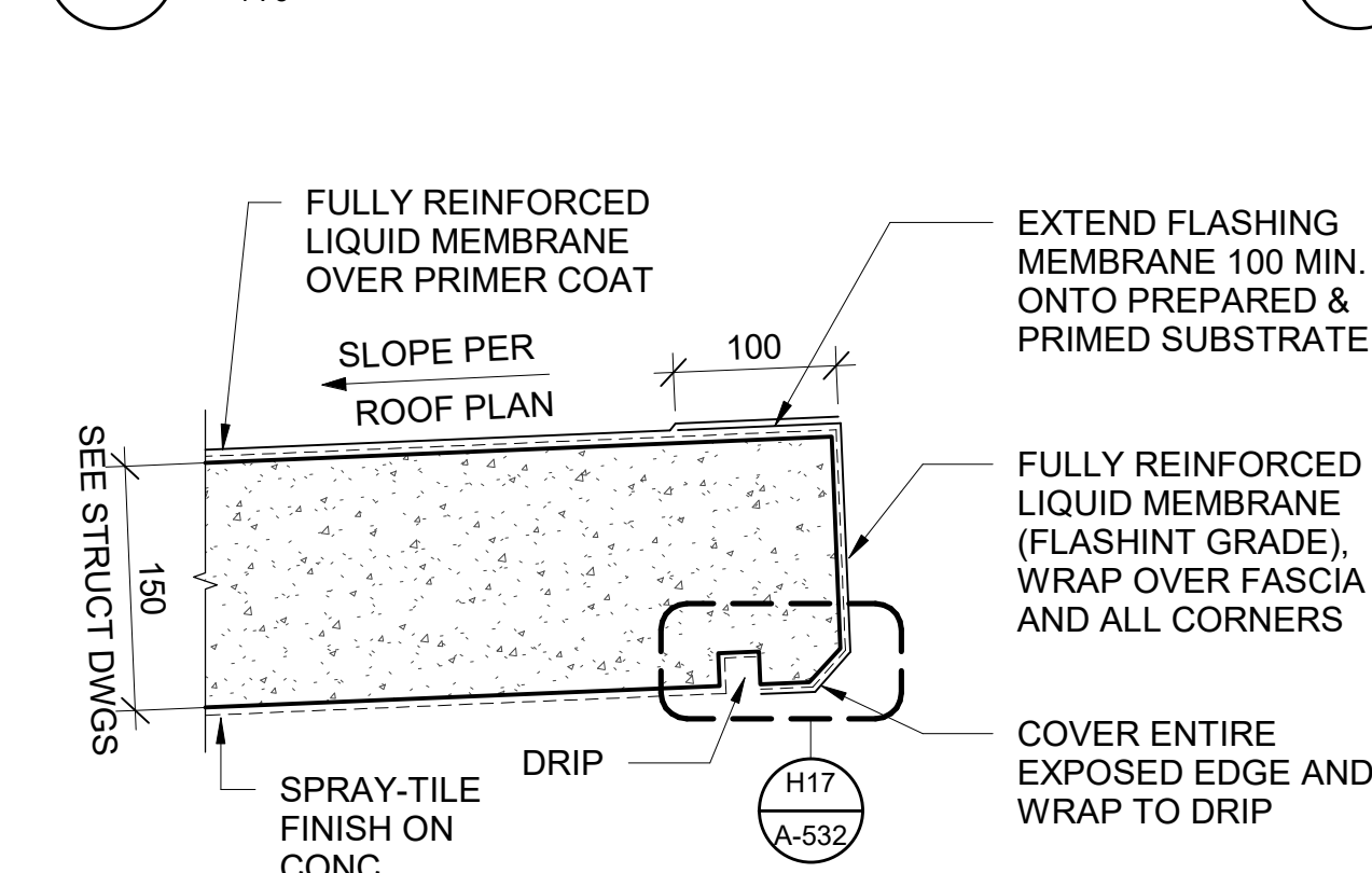
A7 TOP FASCIA - LOW SLOPE
