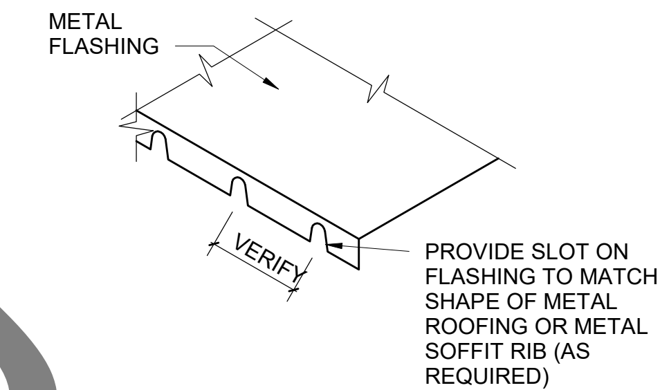
J11 SLOT FLASHING DETAIL
