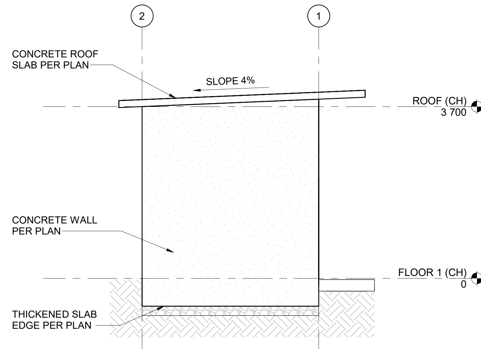
K12 CH - EXTERIOR ELEVATION - NORTH (CLIN 0001) SCALE 1 : 50
