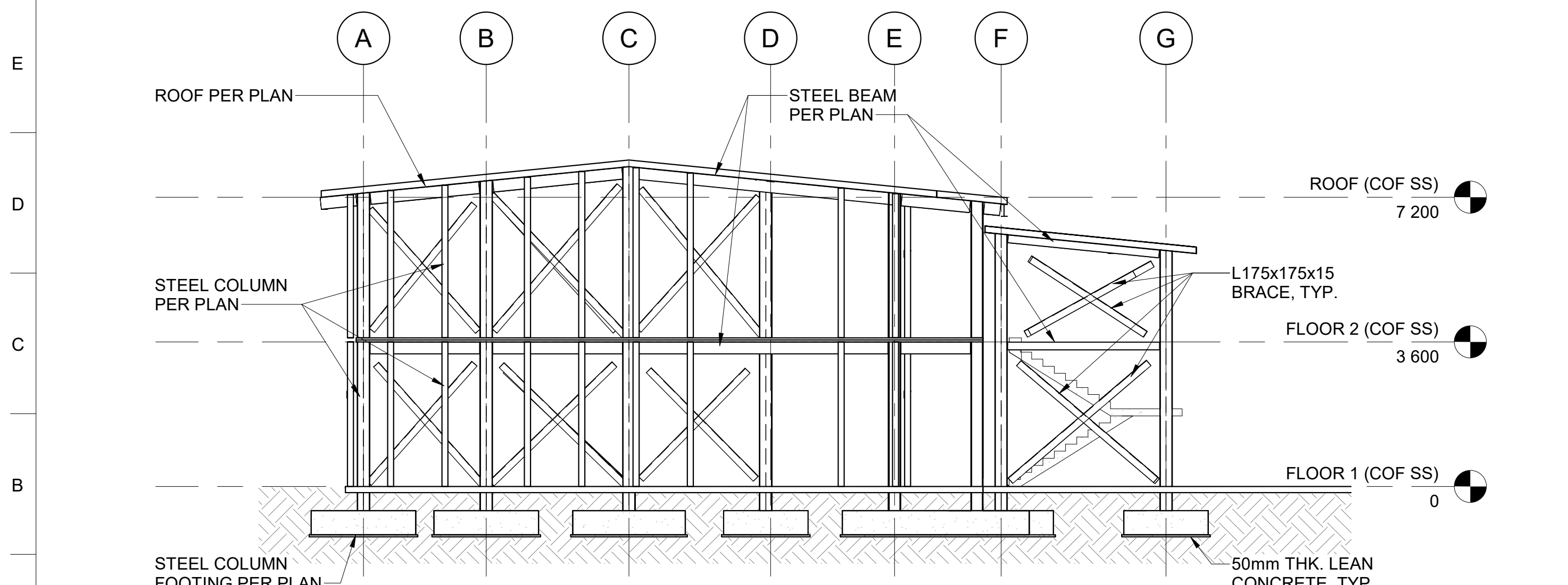
A1 COF SS - EXTERIOR ELEVATION WEST (CLIN 0004) SCALE 1 : 100
