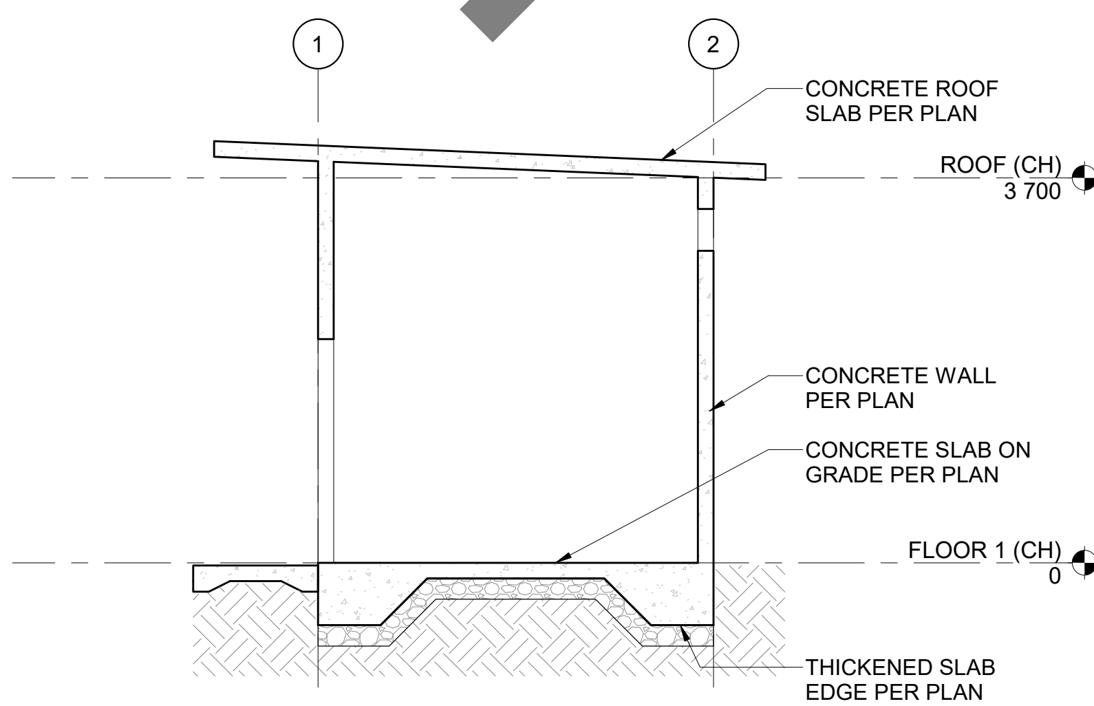
A12 CH - BUILDING SECTION (CLIN 0001) SCALE 1 : 50
