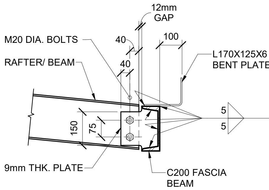
CONDITION AT H175/H200 STEEL RAFTER/B EAM
