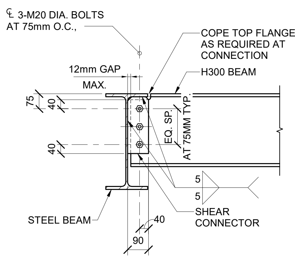
CONDITION AT H300 BEAM
