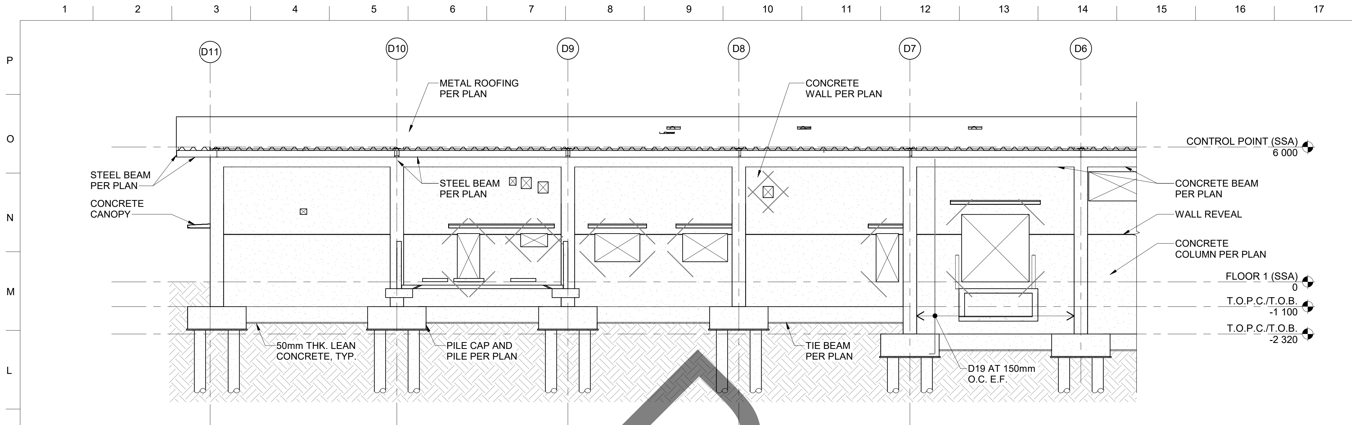
K1 SSAW - PARTIAL EXTERIOR ELEVATION - NORTH (EAST) (CLIN 004) SCALE 1 : 100
