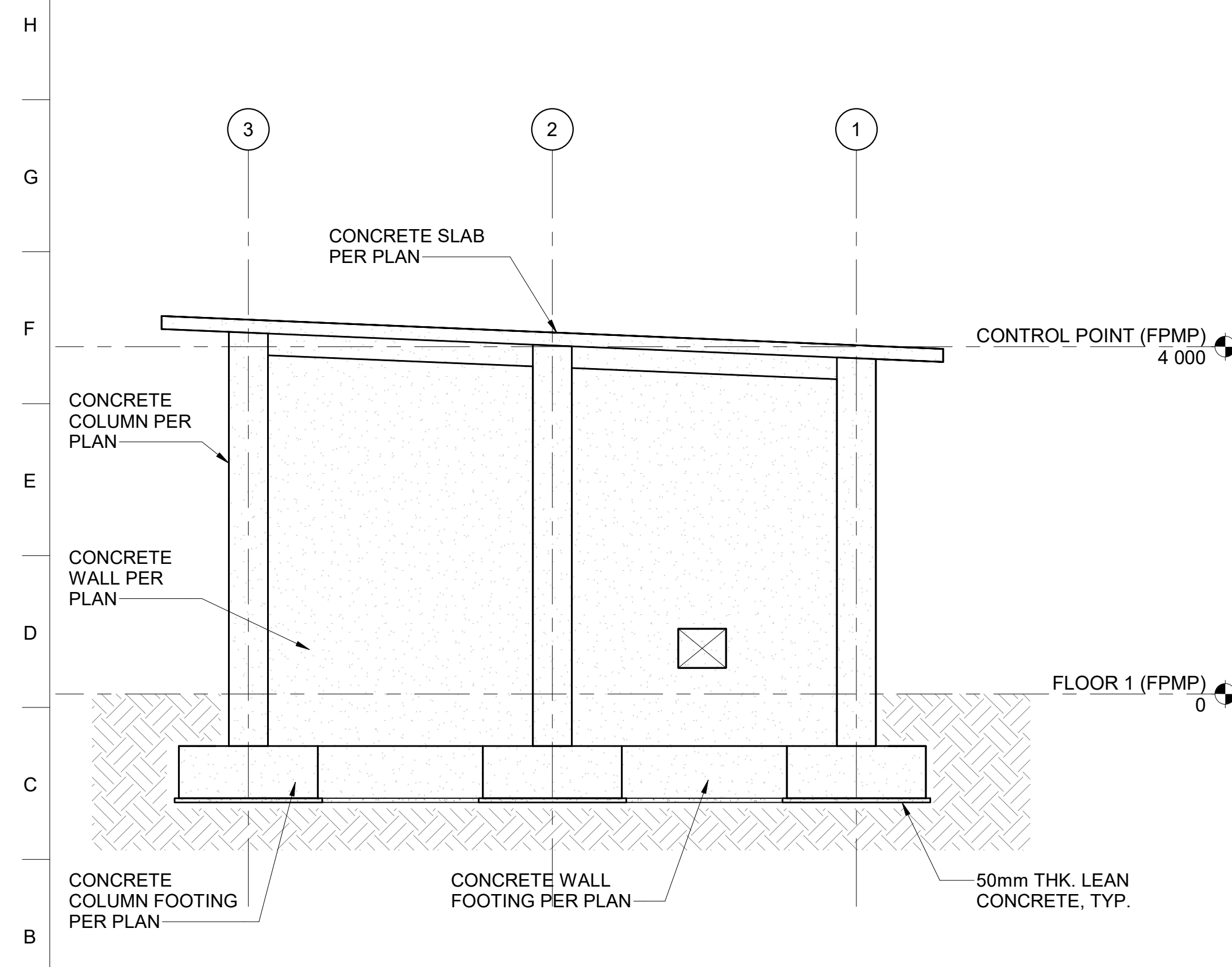
A1 FP - EXTERIOR ELEVATION - NORTH (CLIN 0001) SCALE 1 : 50
