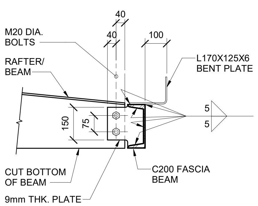
CONDITION AT H250/H300/H400 STEEL RAFTER/B EAM
