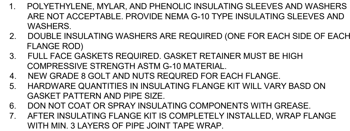
A14 DIELECTRIC INSULATING FLANGE SCALE: NTS
