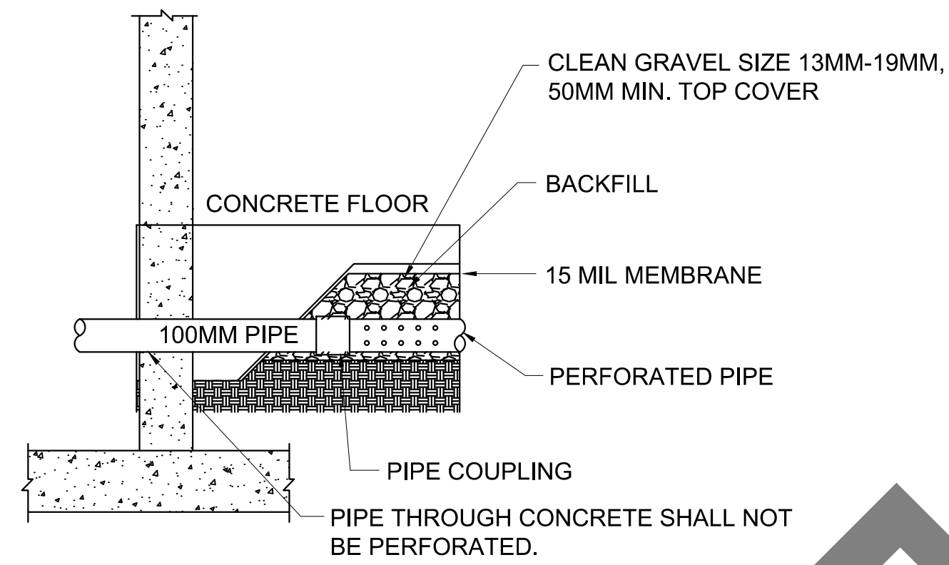
K4 RADON PIPE PENETRATION DETAIL NTS
