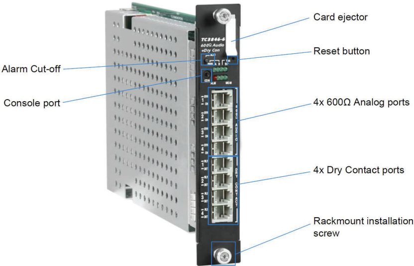
TC3846-6 4-Channel 600Ω Analog & Dry Contact Card
