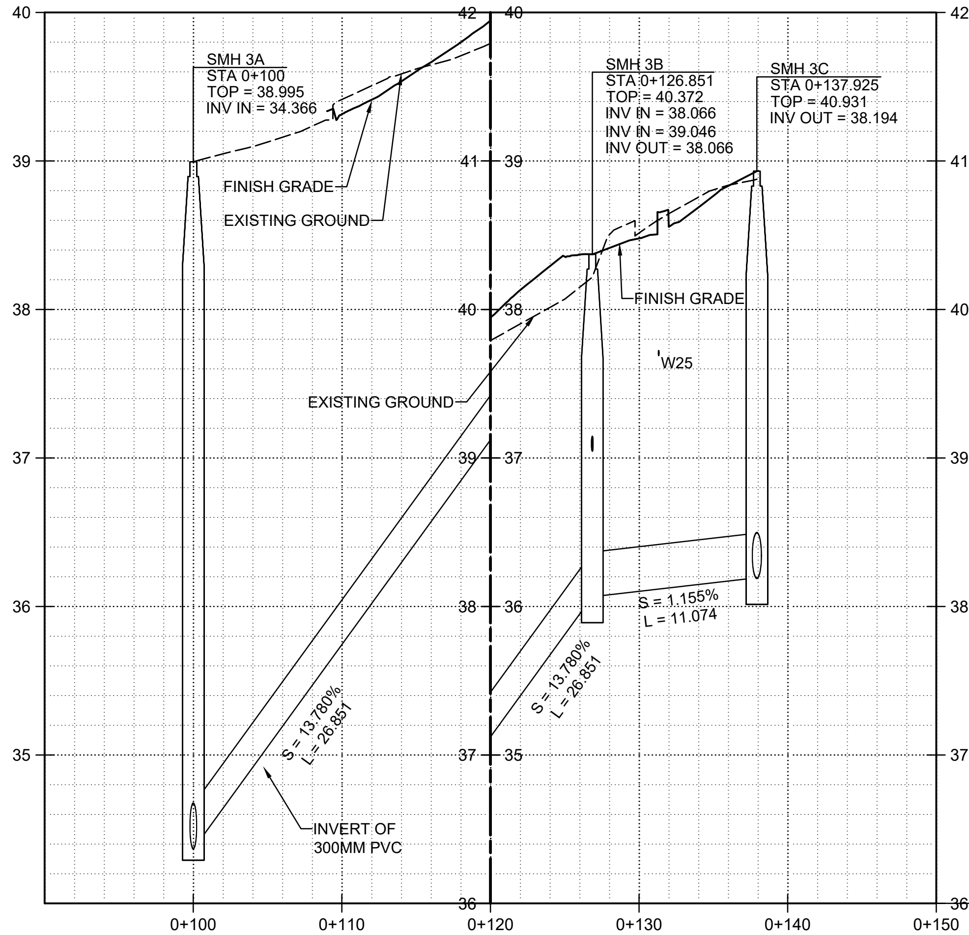
A1 SEWERLINE 3 - PROFILE (CLIN 0001) SCALE: H 1:250 V 1:25
