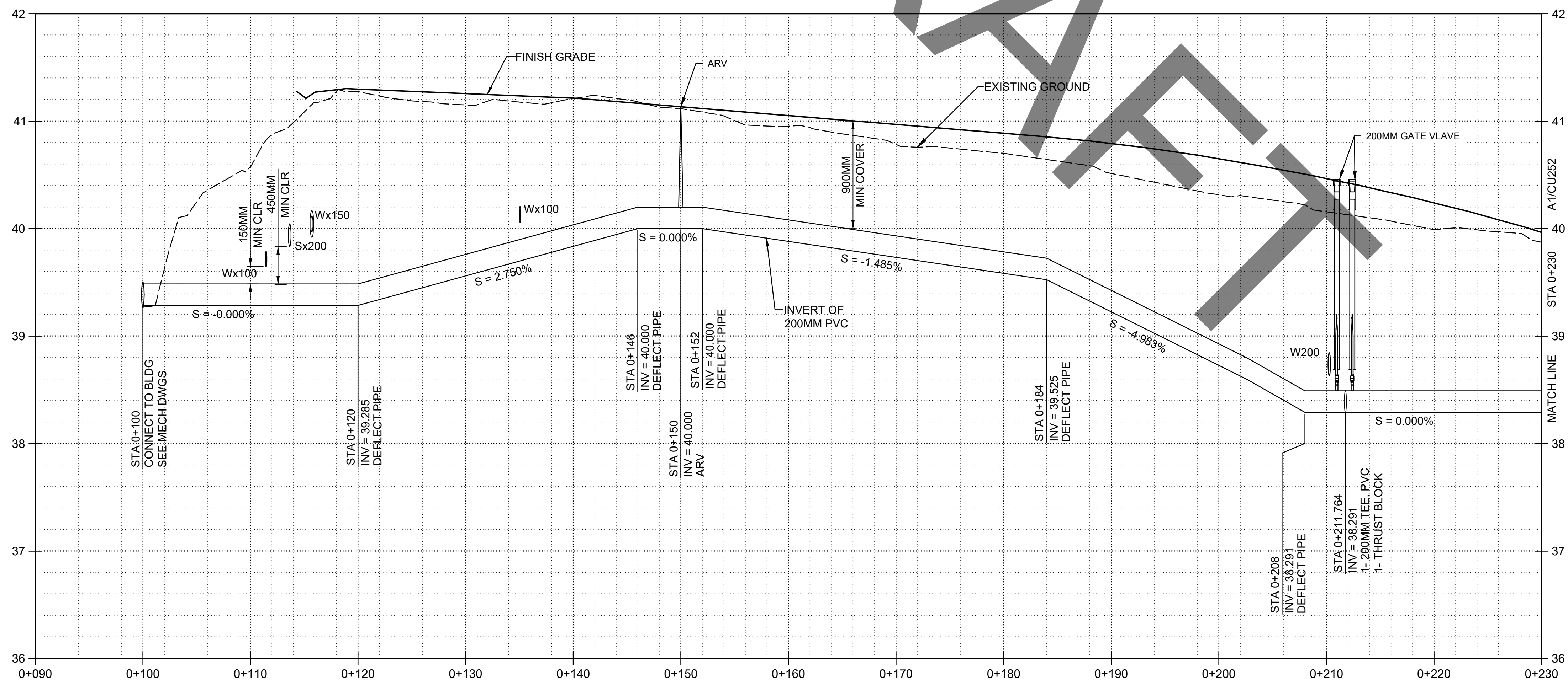
A1 FIRELINE 1 - PROFILE (CLIN 0001) SCALE: H 1:250 V 1:25
