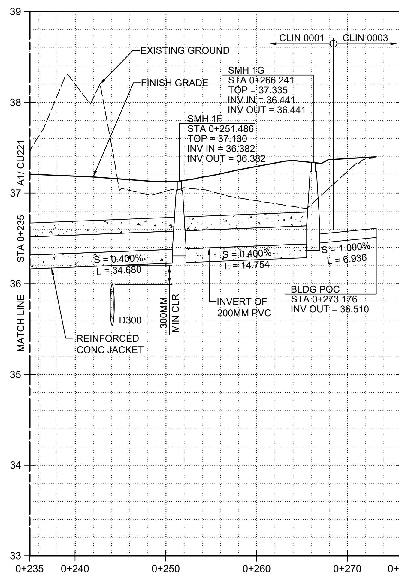
A1 SEWERLINE 1 - PROFILE (CLIN 0001 - CLIN 0003) SCALE: H 1:250 V 1:25
