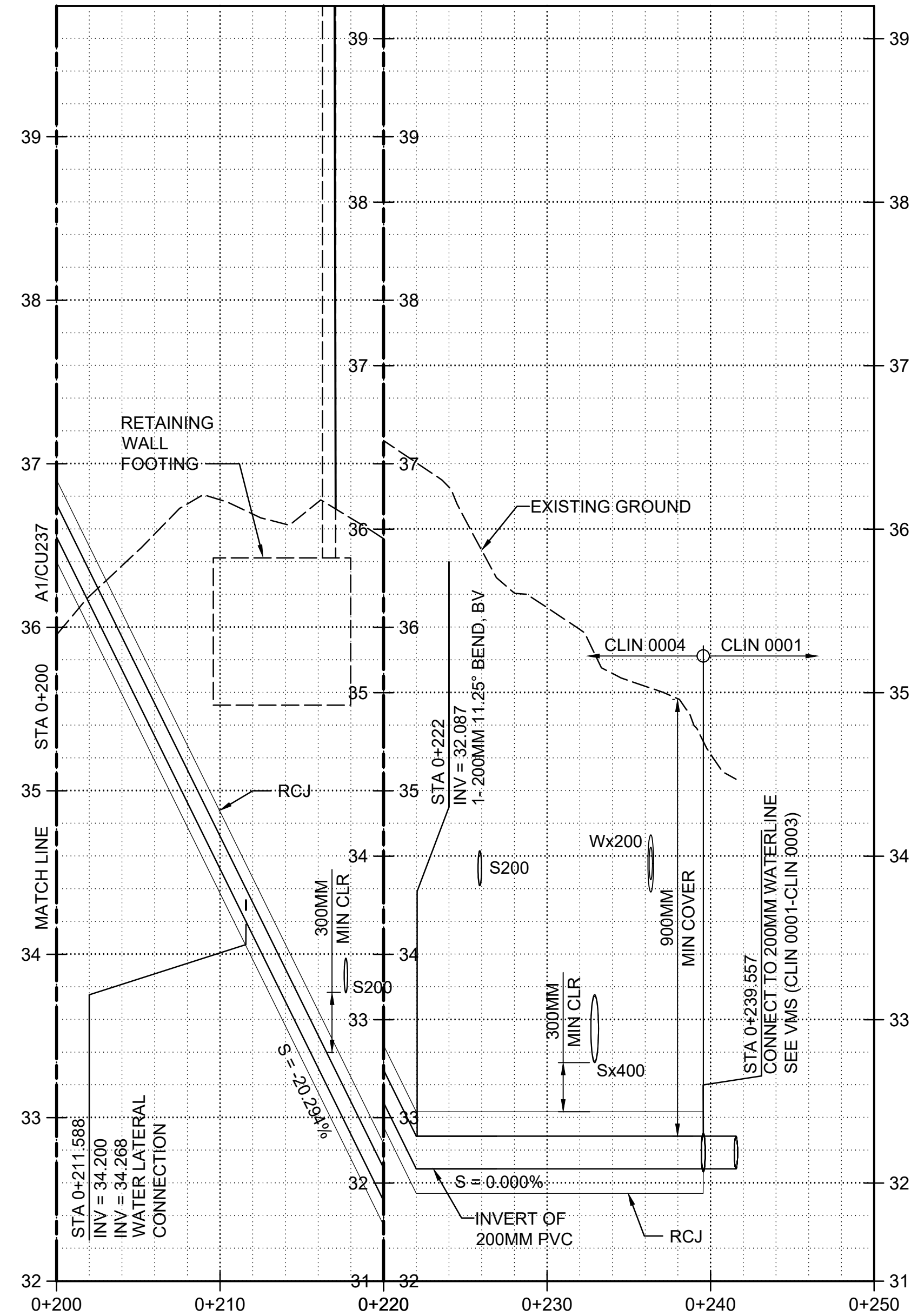
A1 WATERLINE 20 - PROFILE (CLIN 0004) SCALE: H 1:250 V 1:25
