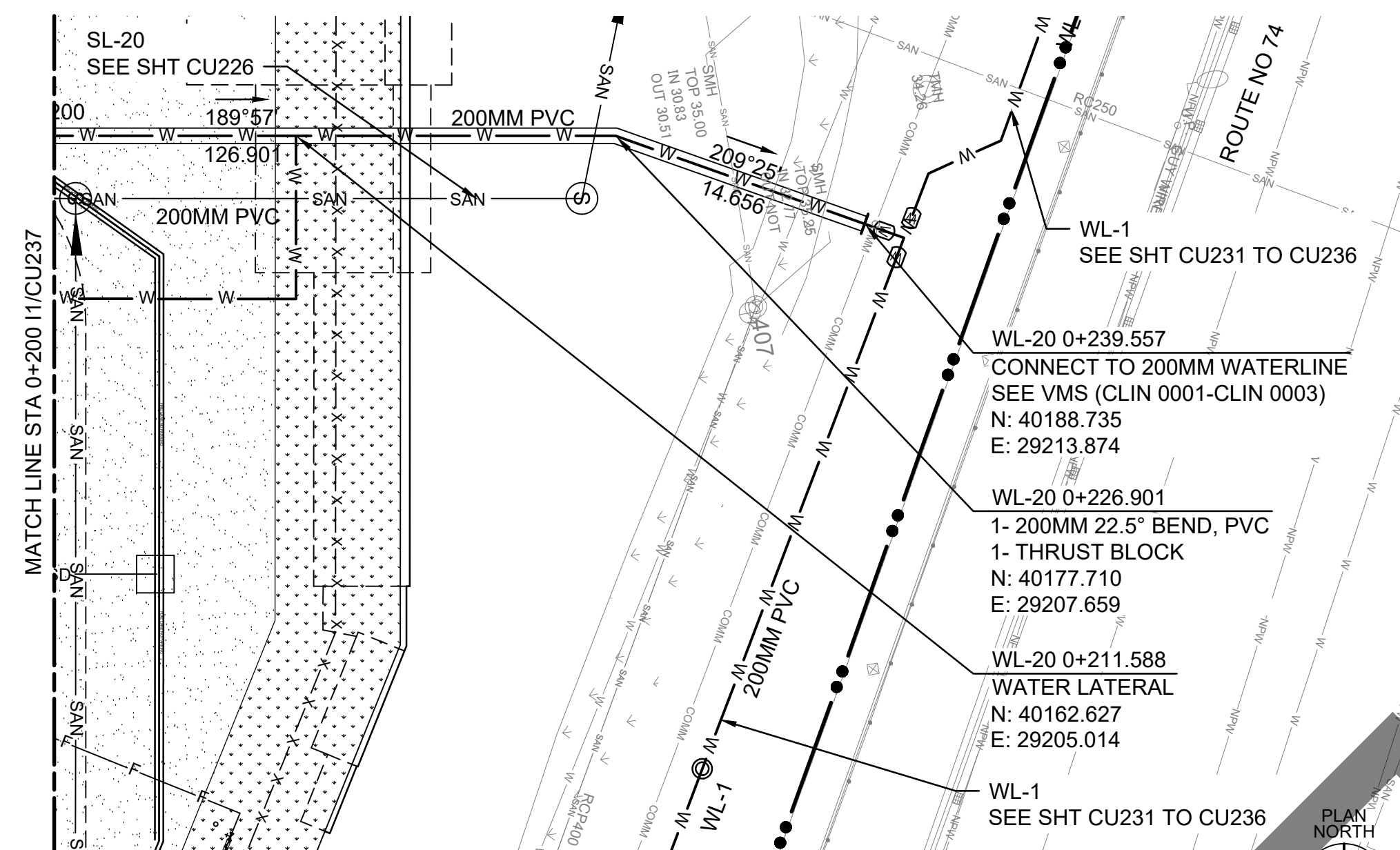
K1 WATERLINE 20 - PLAN (CLIN 0004) SCALE: 1:250
