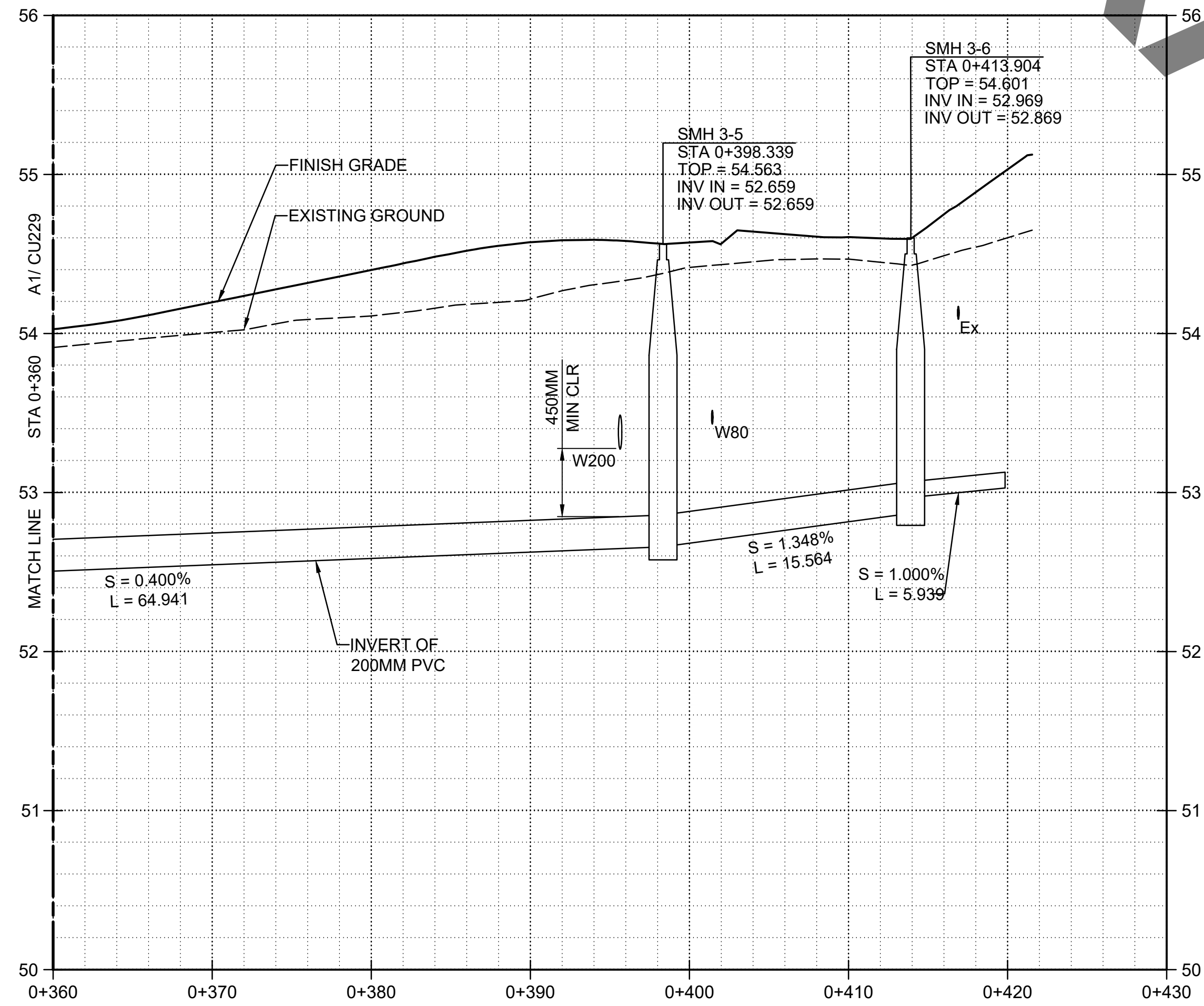
A1 SEWERLINE 30 - PROFILE (CLIN 0004) SCALE: H 1:250 V 1:25
