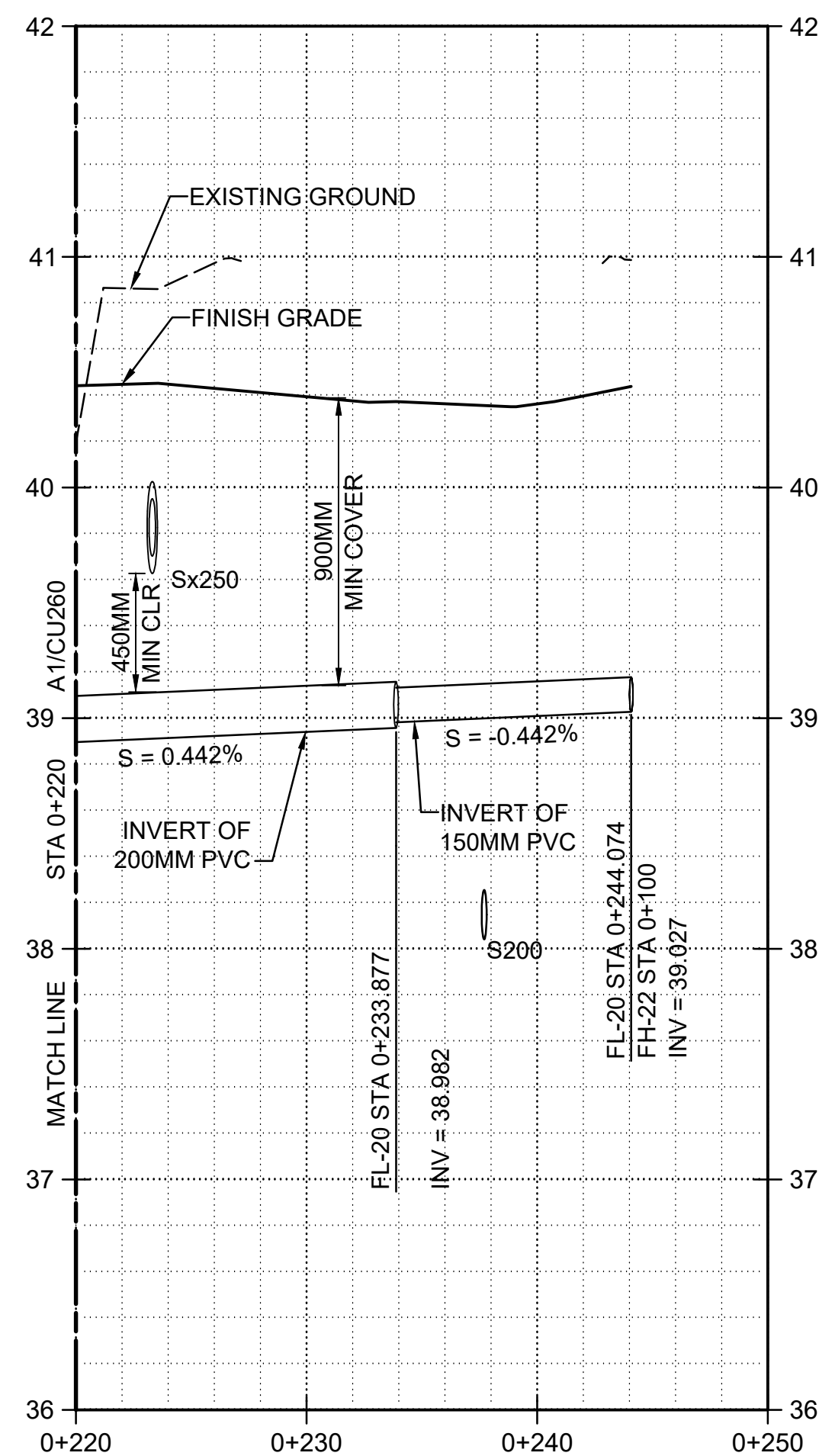
A1 FIRELINE 20 - PROFILE (CLIN 0004)
