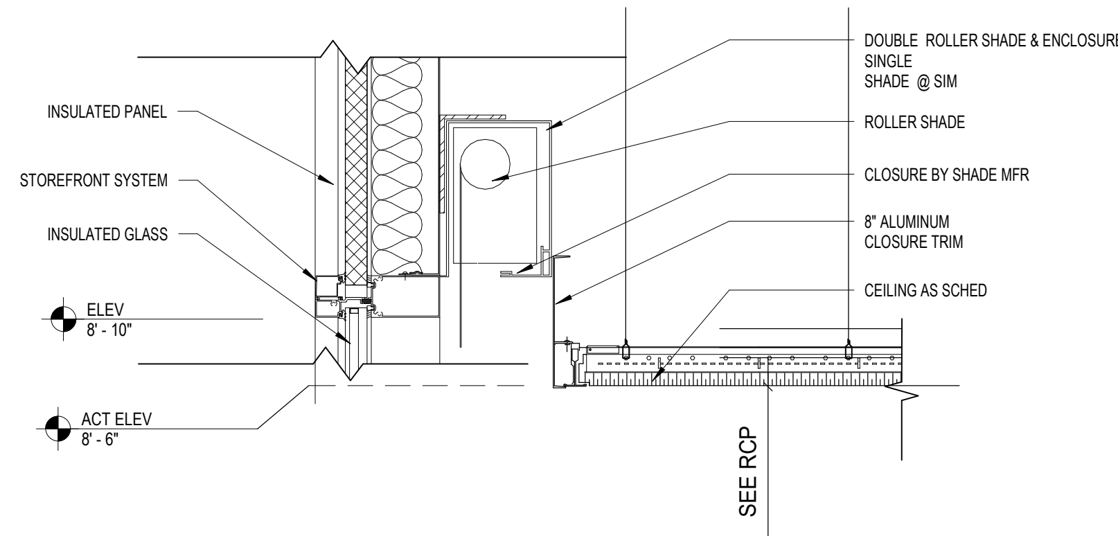
3 ACT CONNECTION AT SINGLE ROLLER SHADE 1 1/2" = 1'-0"
