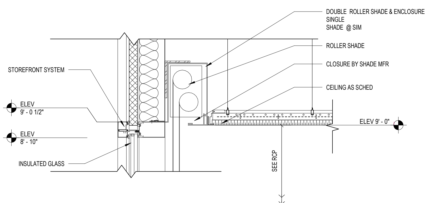
2 ACT CONNECTION AT DOUBLE ROLLER SHADE 1 1/2" = 1'-0"
