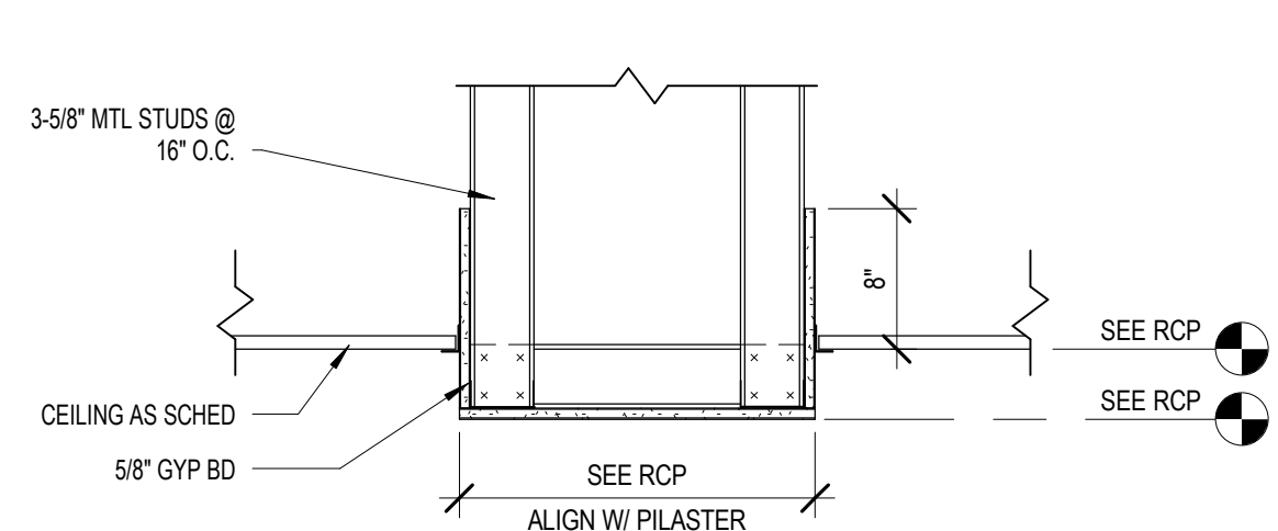
2 TYPICAL CORRIDOR FURDOWN AE111 1\" = 1'-0"
