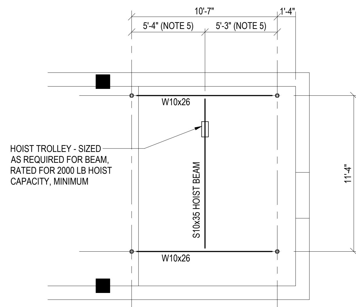
PLAN NORTH 3 HOIST FRAMING PLAN DETAIL 1/4" = 1'-0"
