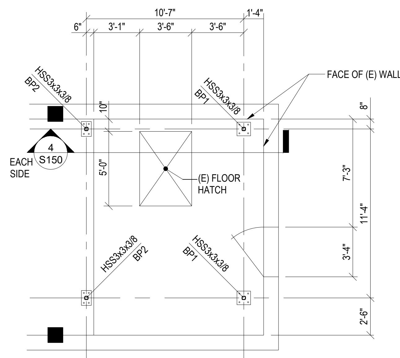
PLAN NORTH 2 HOIST PLAN BASE DETAIL 1/4" = 1'-0"
