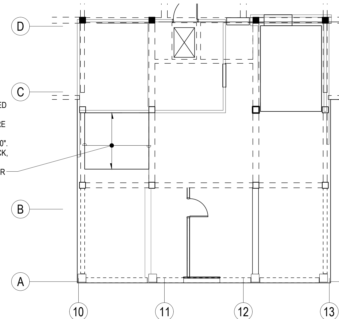
PLAN NORTH 4 PARTIAL ROOF PLAN 1/8" = 1'-0"
