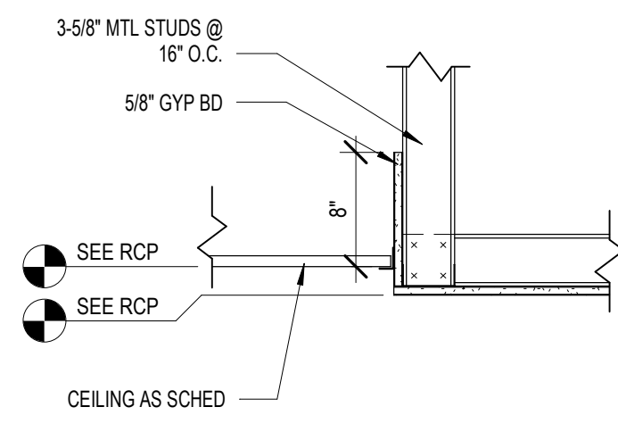
3 TYPICAL CEILING TRANSITION AE111 1\" = 1'-0"
