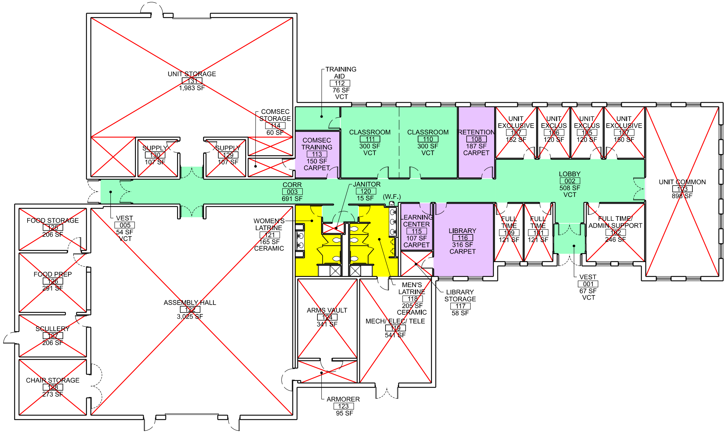
1 CUSTODIAL SERVICE PLAN - USARC SCALE: 1/16" = 1'-0"
