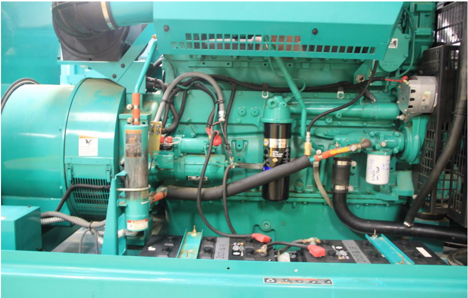
Failed block heater and associated components on Generator #1
