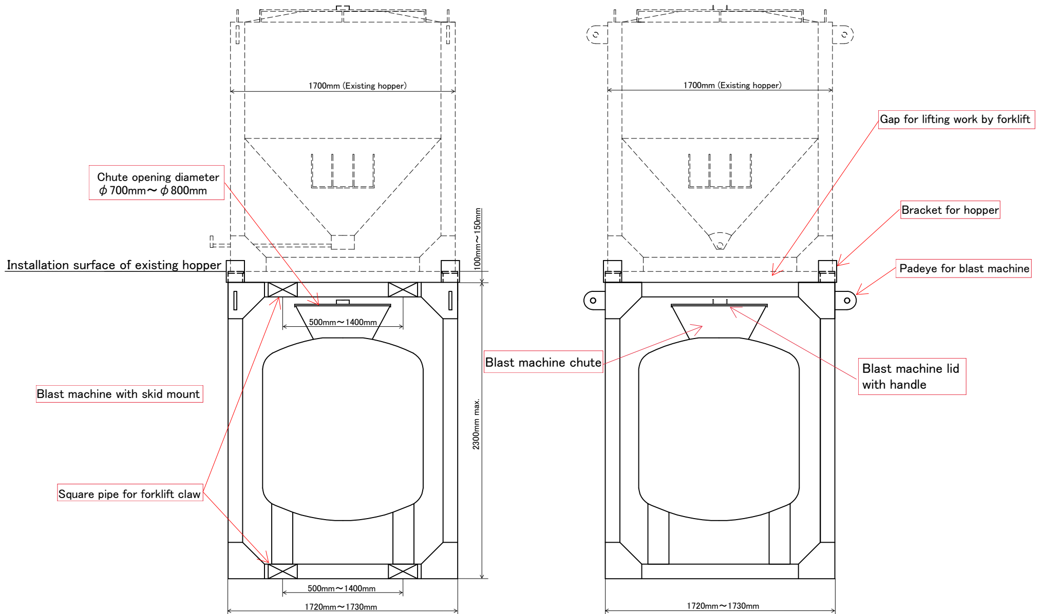
Detail for Blast Machine
