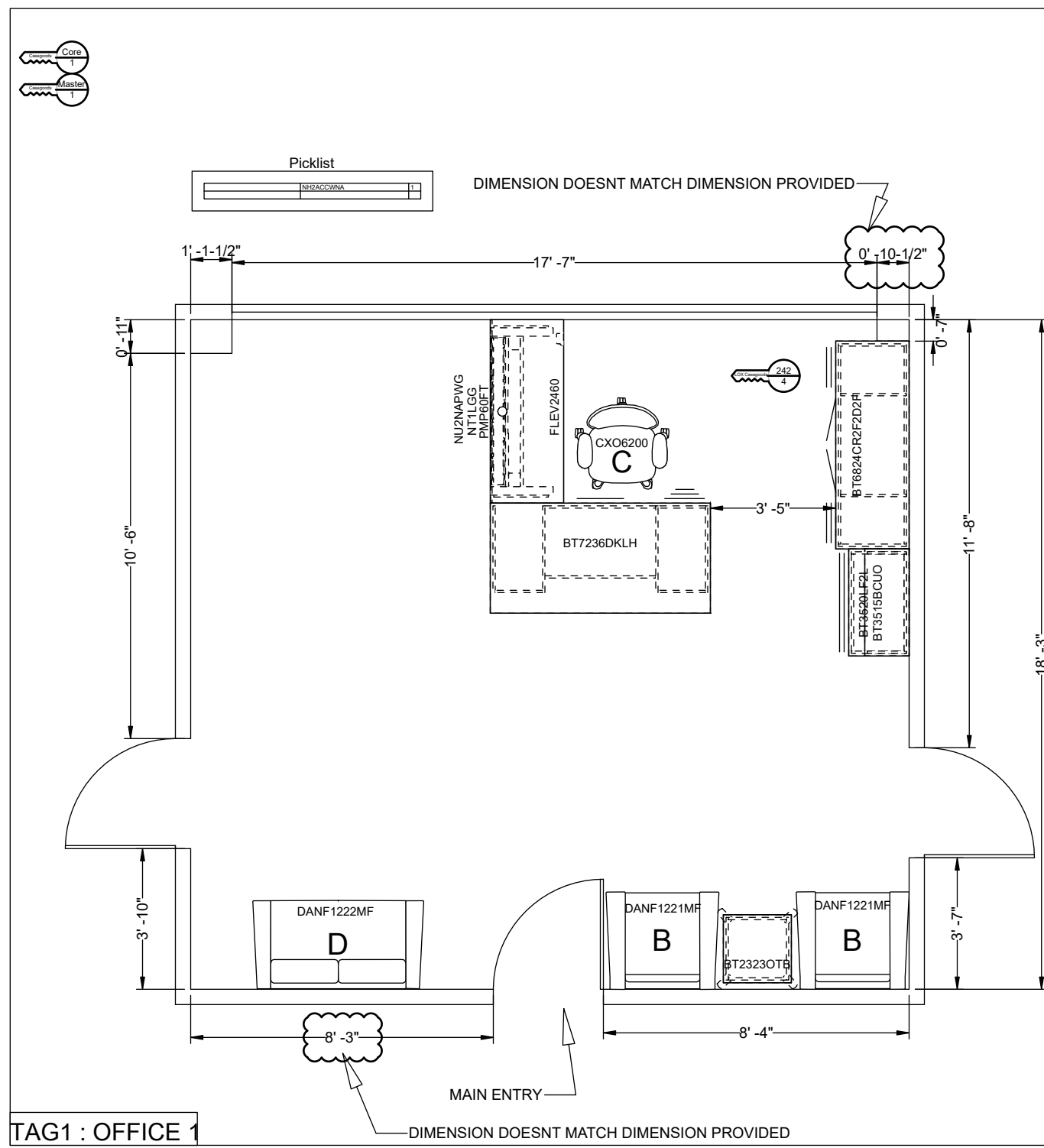
FLOOR PLAN
