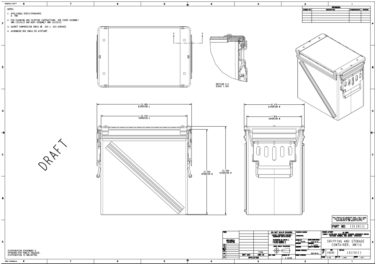
Figure 1: Lightweight Steel Outer Container Representative Drawing
