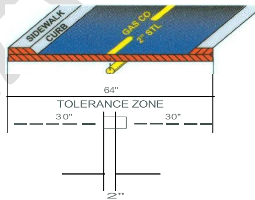
SMALL PIPE OR CABLES
