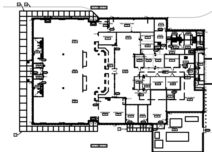
1 128 OVERALL FLOOR PLAN A2 | A2 1/32" = 1'-0" 0 20' 40' 80'
