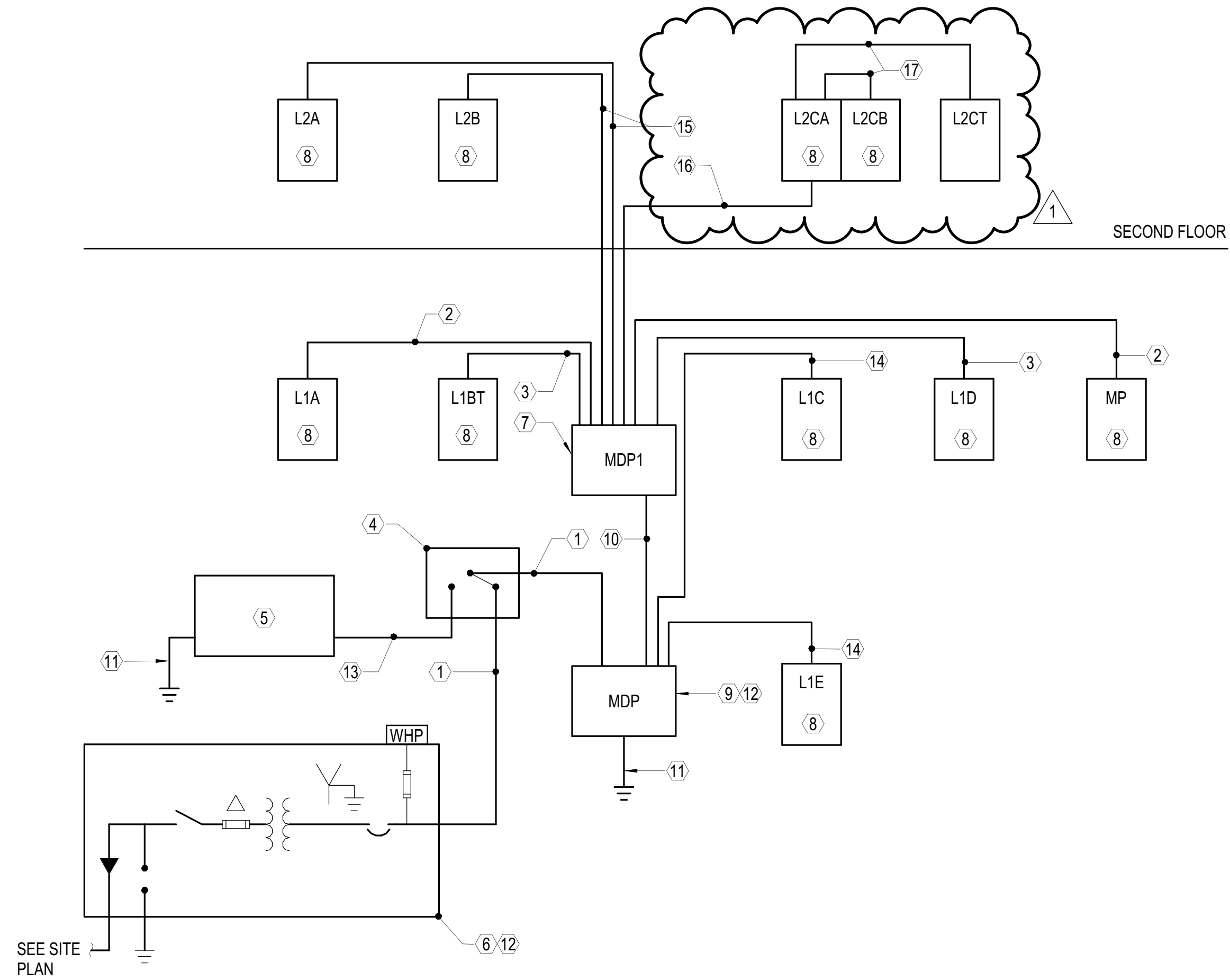
A2 POWER RISER DIAGRAM NOT TO SCALE
