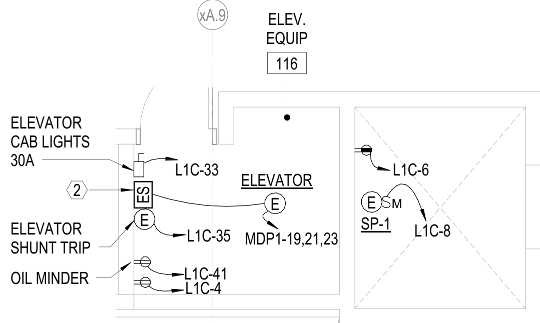
A1 ENLARGED POWER PLAN RM 116 1/4" = 1'-0"
