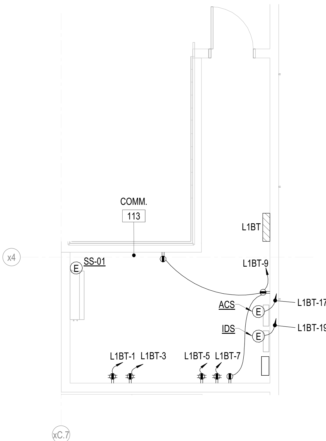
A3 ENLARGED POWER PLAN RM 113 1/4" = 1'-0"
