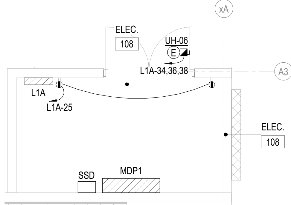
C2 ENLARGED POWER PLAN RM 108 1/4" = 1'-0"
