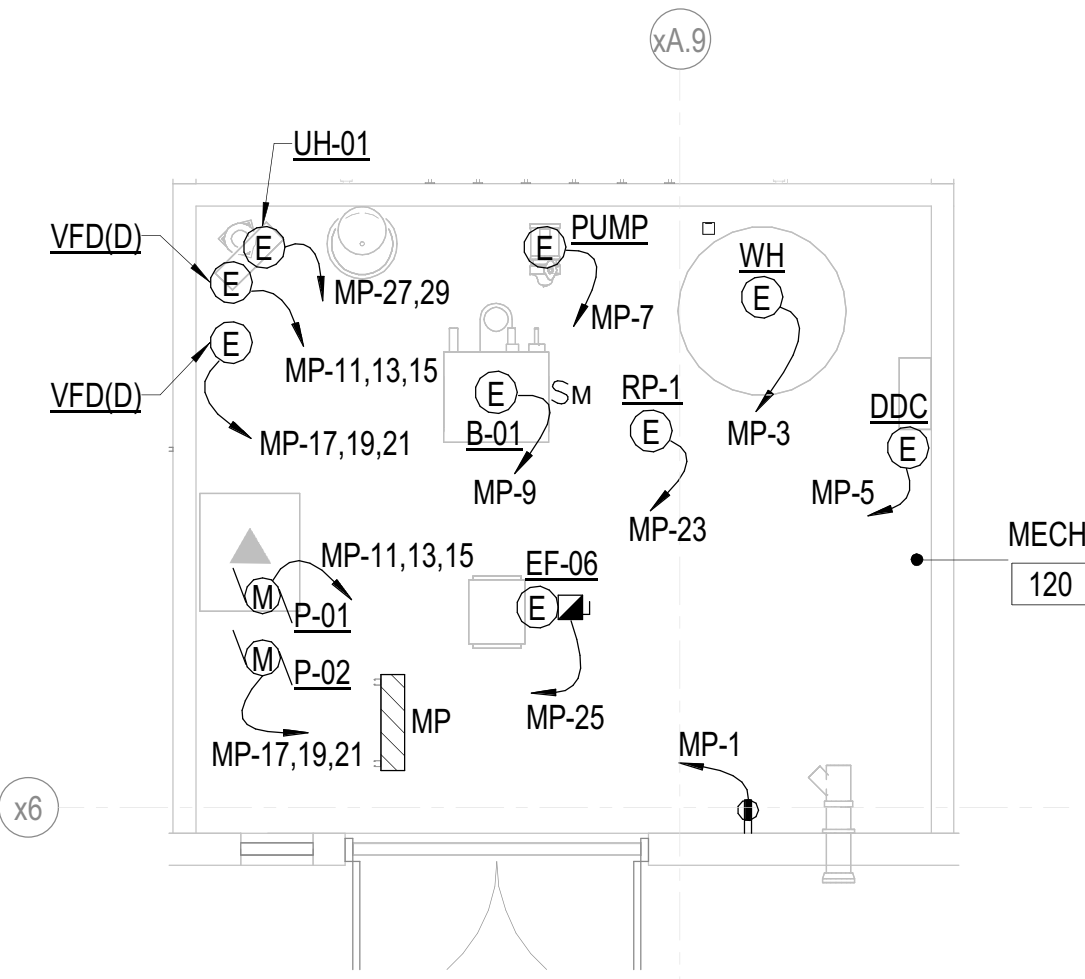
A2 ENLARGED POWER PLAN RM 120 1/4" = 1'-0"
