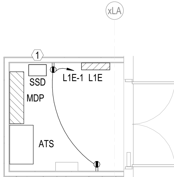
C5 ENLARGED POWER PLAN RM 125 1/4" = 1'-0"
