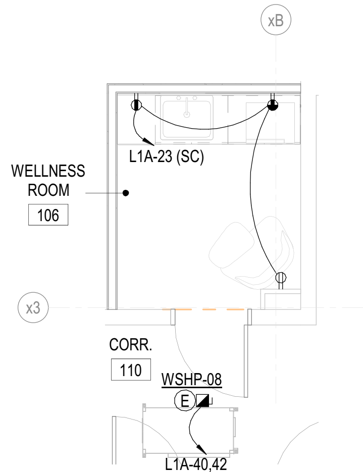
C1 ENLARGED POWER PLAN RM 106 1/4" = 1'-0"
