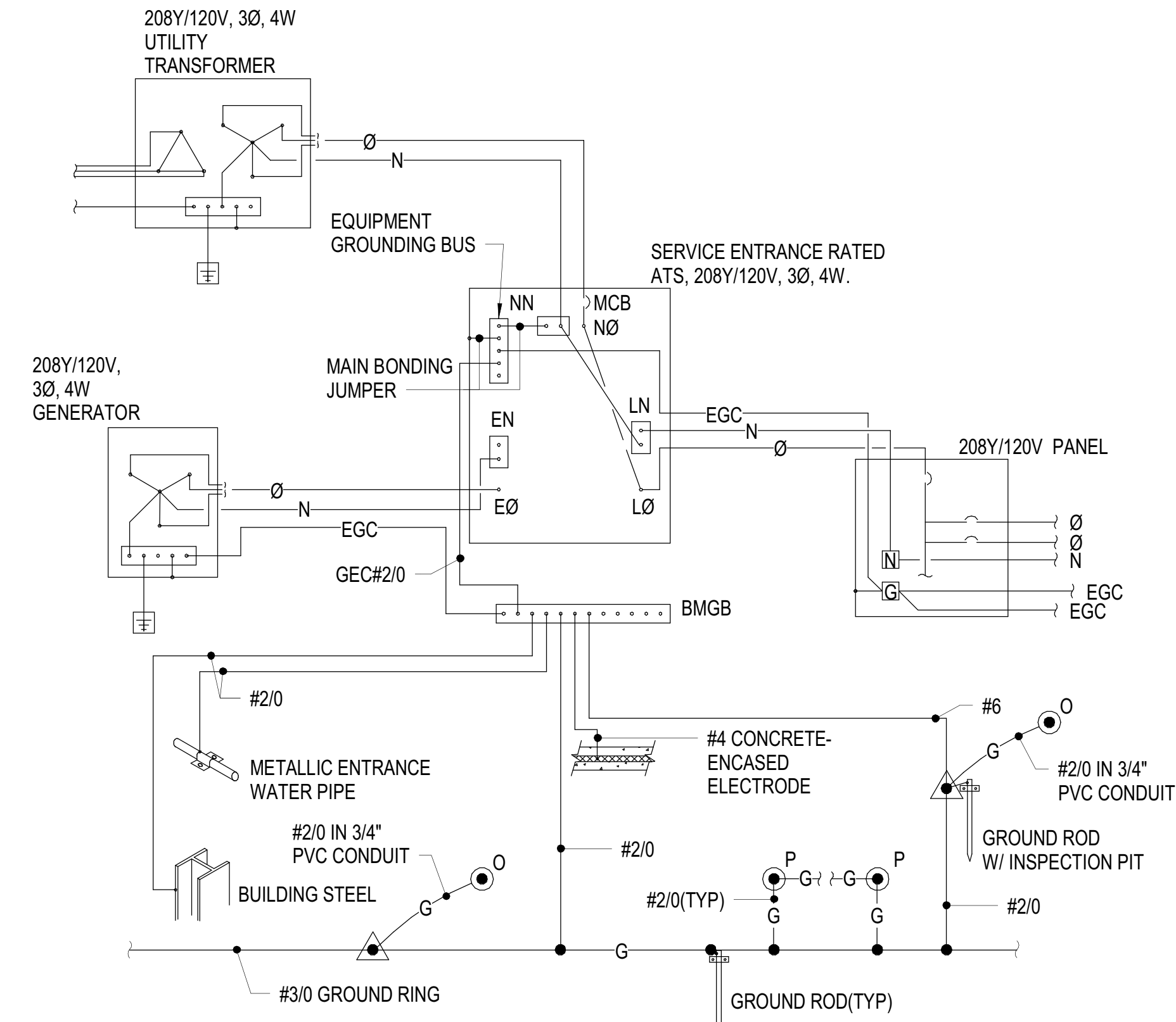
A1 SERVICE GROUNDING DIAGRAM NOT TO SCALE
