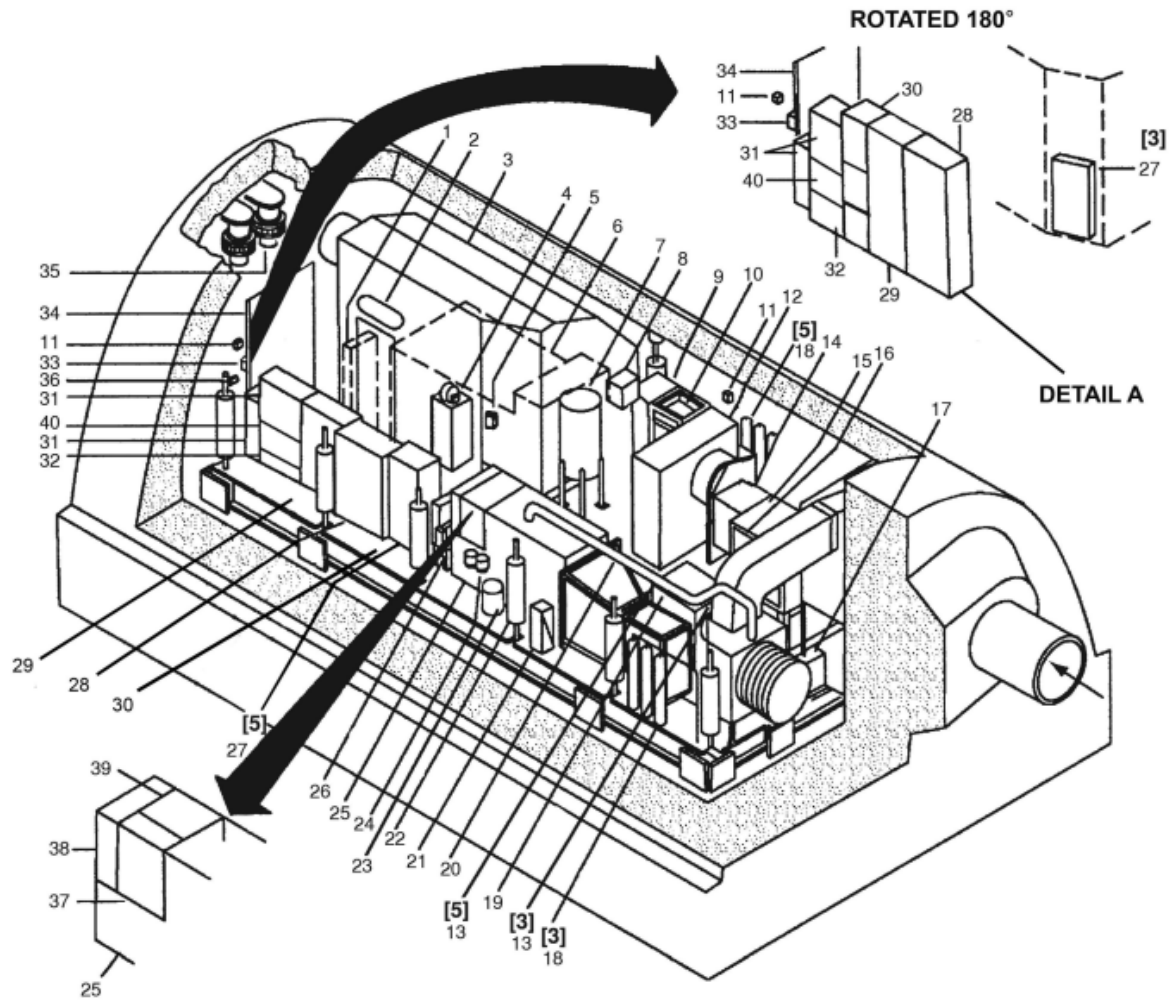
Diagram 3: Launch Control Equipment Building
