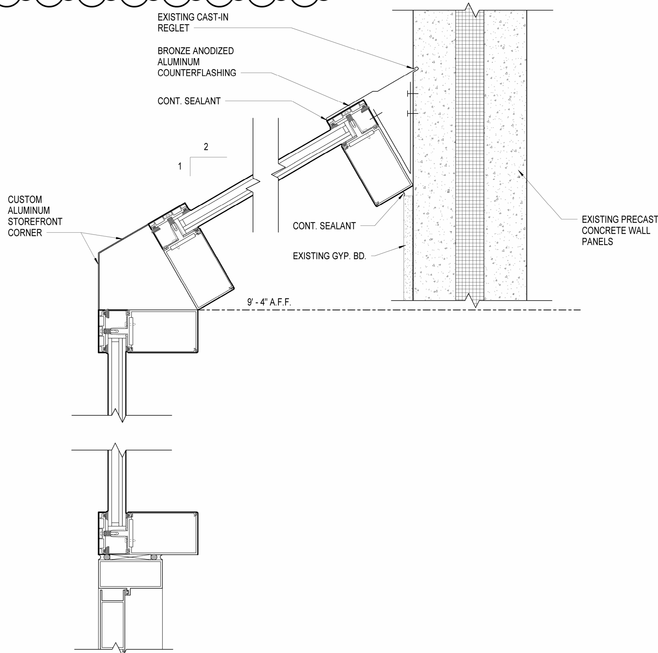
C3 JAMB DETAIL 3" = 1'-0" AT ENTRY STOREFRONT
