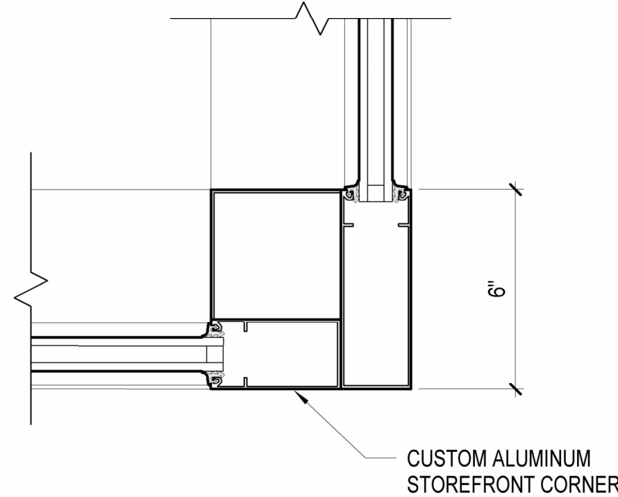
B2 STOREFRONT CORNER DETAIL 3" = 1'-0" AT ENTRY STOREFRONT
