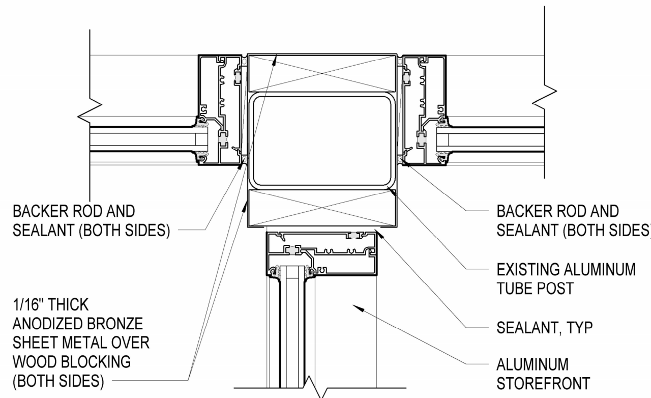
B1 STOREFRONT CORNER DETAIL 3" = 1'-0" AT ENTRY STOREFRONT
