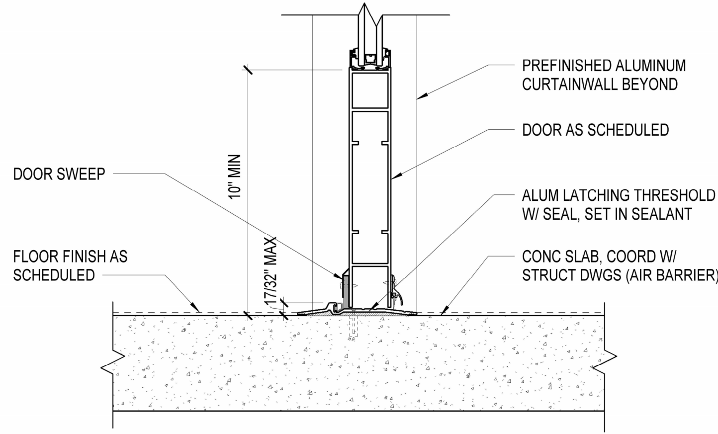
C1 SILL DETAIL 3" = 1'-0" AT ENTRY STOREFRONT
