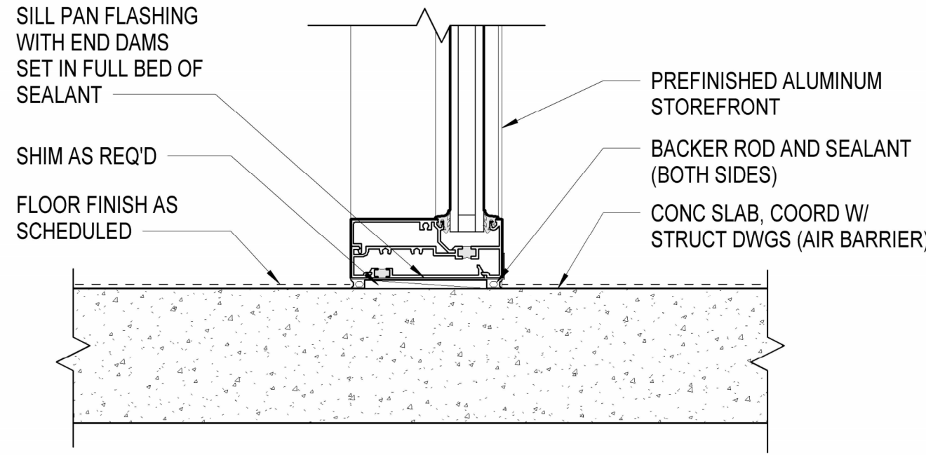
C2 SILL DETAIL 3" = 1'-0" AT ENTRY STOREFRONT
