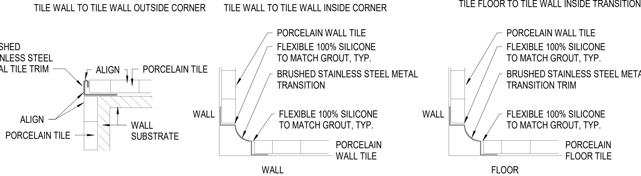
D2 FLOOR AND WALL TILE TRANSITIONS 1 1/2" = 1'-0"
