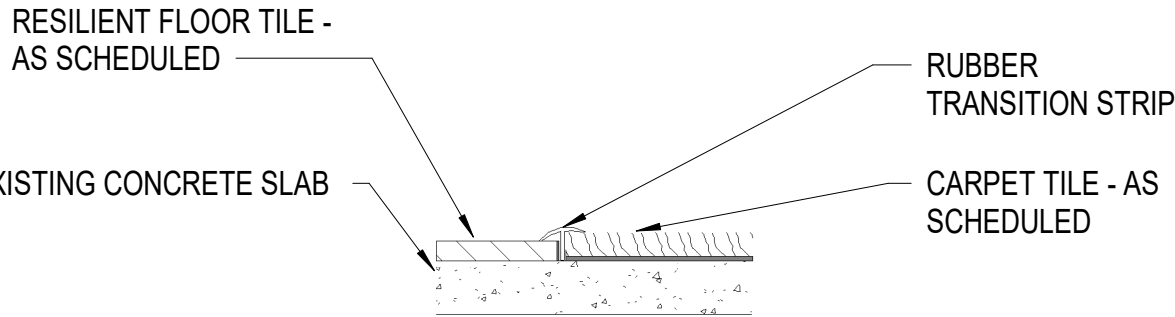
D3 RESILIENT FLOOR TILE TO CARPET TILE TRANSITION 6" = 1'-0"
