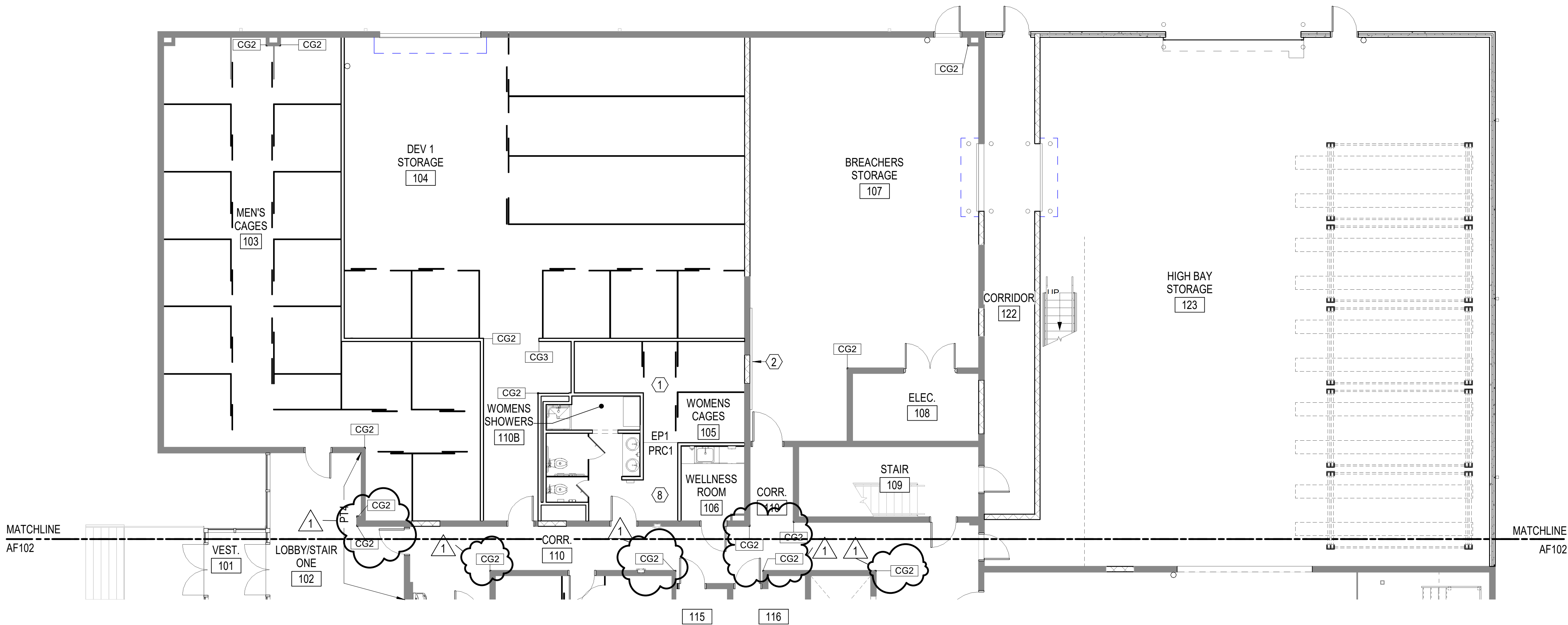
A1 FIRST FLOOR FINISH & SIGNAGE PLAN AREA A 1/8" = 1'-0"
