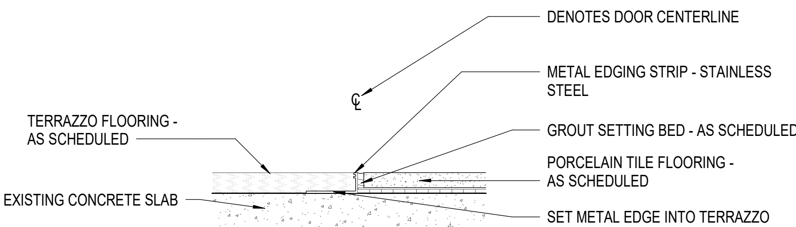
C3 TERRAZZO TO PORCELAIN TILE TRANSITION 3" = 1'-0"
