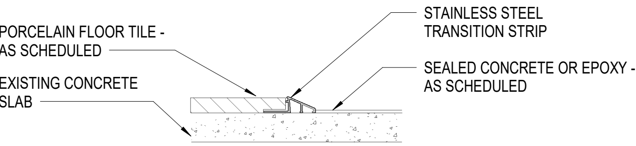
C1 PORCELAIN FLOOR TILE TO CONCRETE FLOOR TRANSITION 6" = 1'-0"
