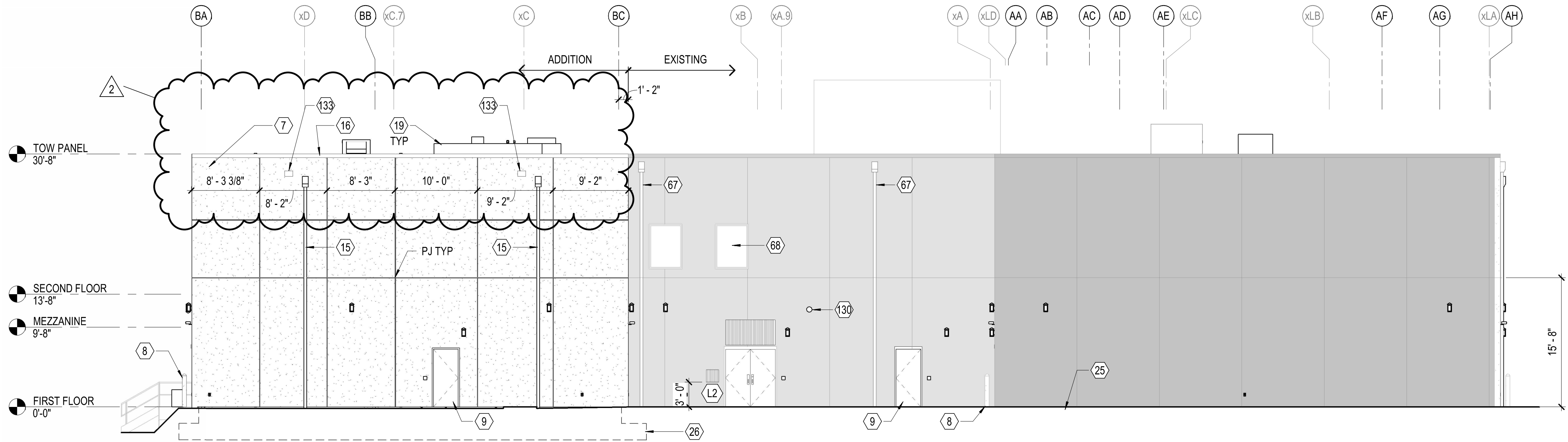
B4 AE101 C1 EXTERIOR BLDG ELEVATION - SOUTH 1/8" = 1'-0"
