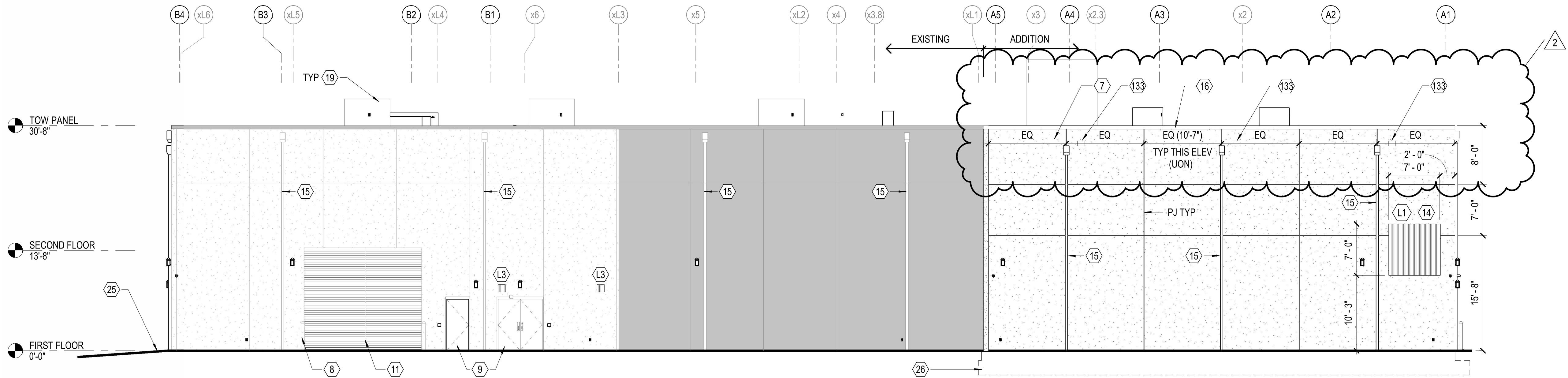
B4 AE101 A1 EXTERIOR BLDG ELEVATION - EAST 1/8" = 1'-0"
