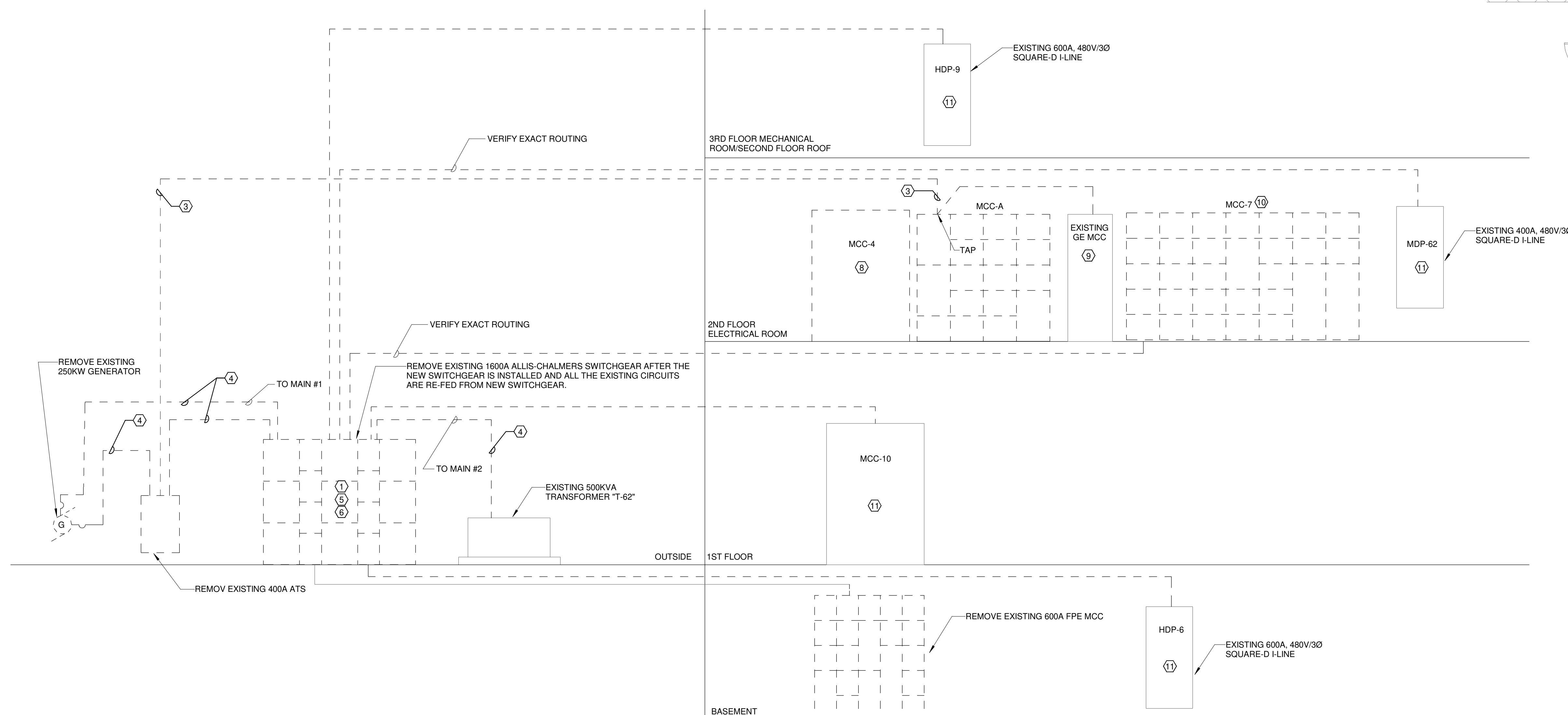
3 ONE-LINE DIAGRAM - BUILDING 62 DEMOLITION NOT TO SCALE
