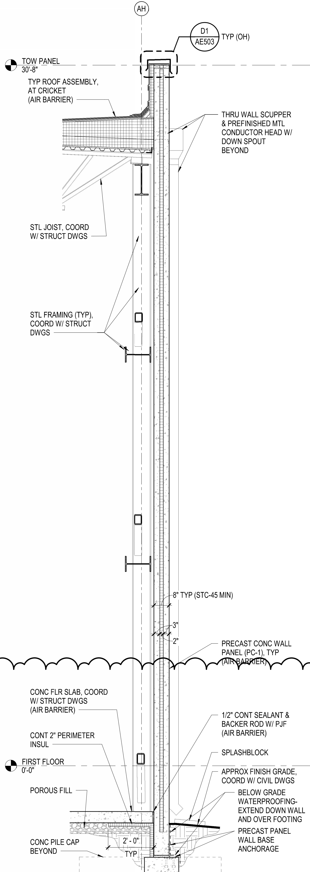
B5 AE301 A1 WALL SECTION 1/2" = 1'-0" TYP WALL SECTION
