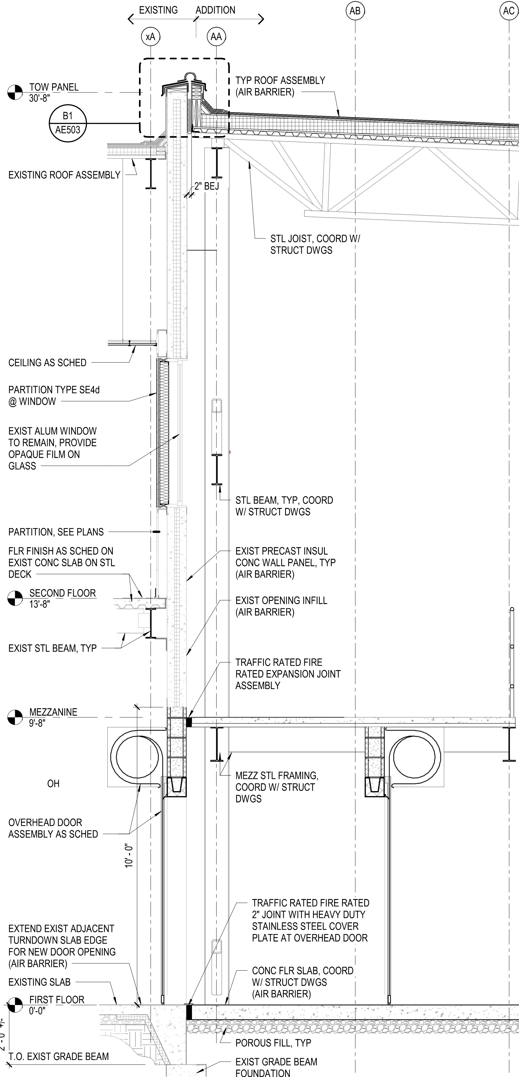
D4 AE103 A2 WALL SECTION 1/2" = 1'-0" AT HIGH BAY 128 WEST WALL
