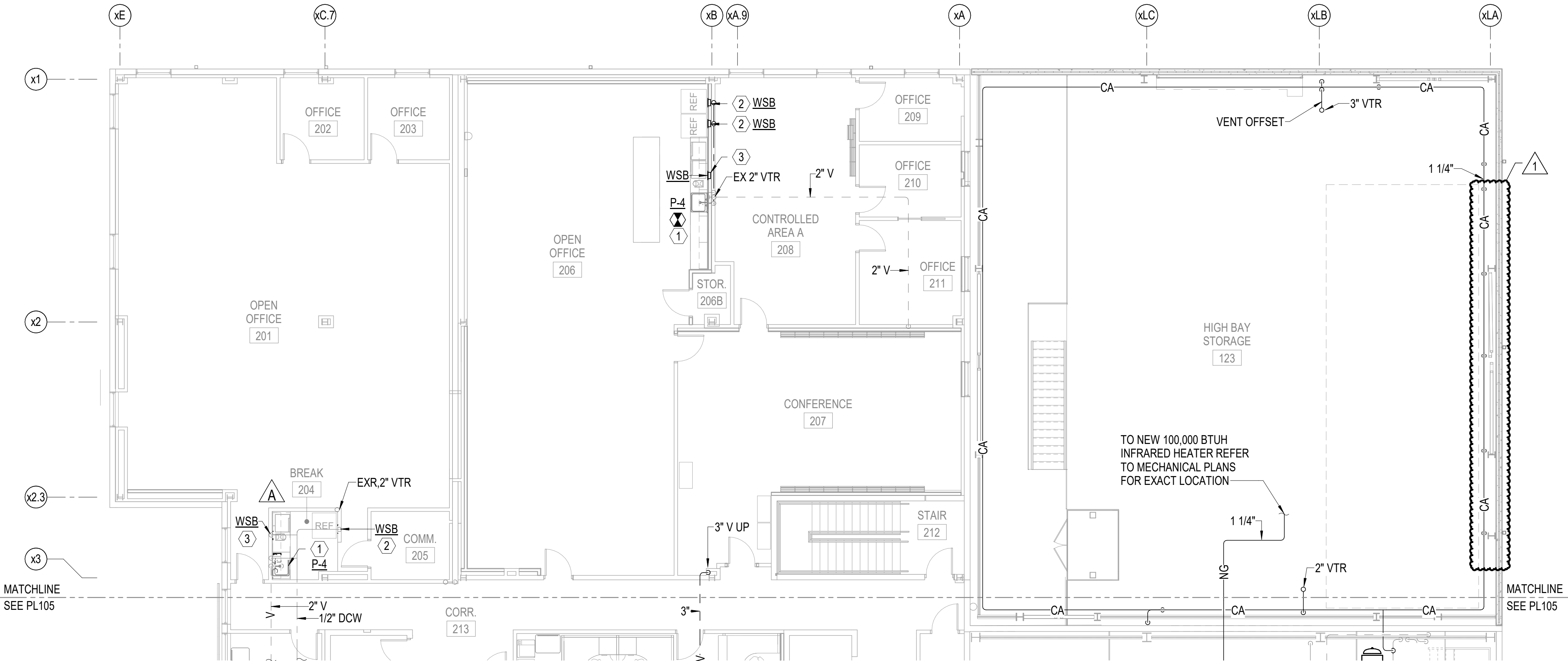
SECOND FLOOR AREA A 1/8" = 1'-0"
