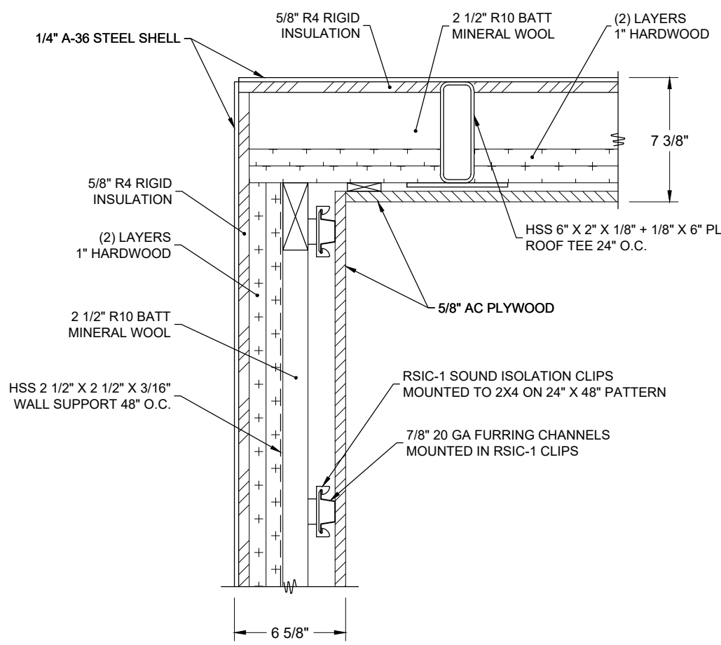
TYPICAL WALL / ROOF CONSTRUCTION
