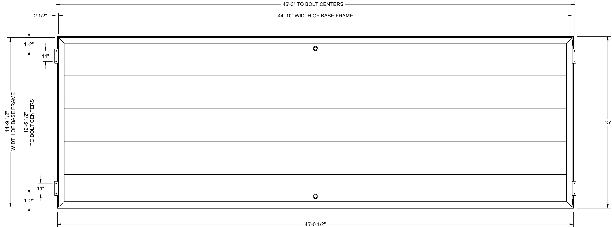
BASE FRAMING PLAN
