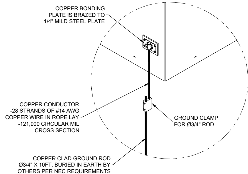
TYPICAL GROUNDING KIT
