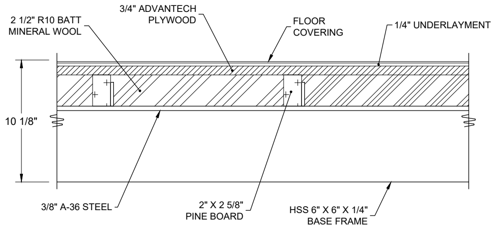
TYPICAL FLOOR CONSTRUCTION
