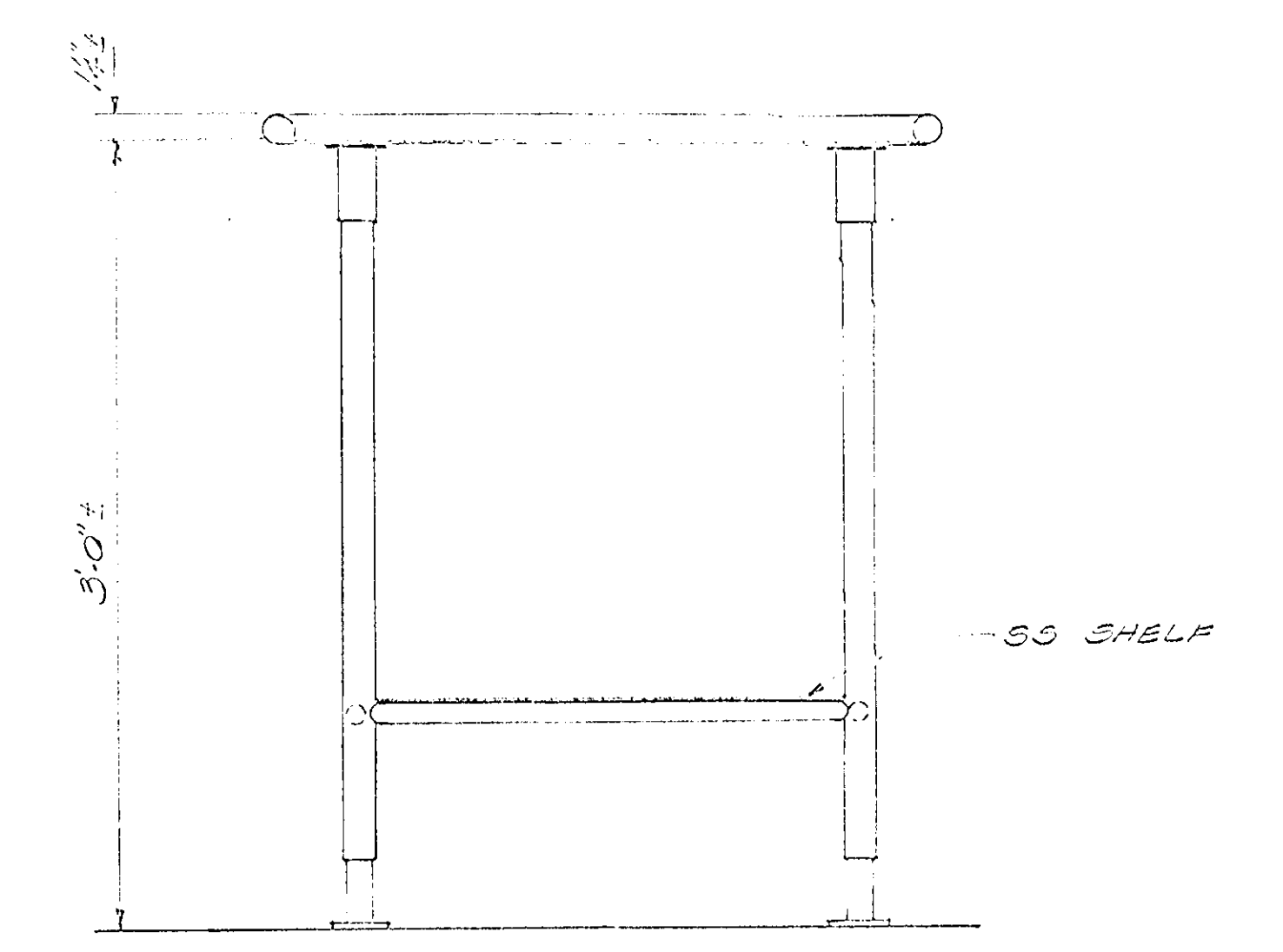
ELEVATION 4 SCALE - 1/2" = 1'-0"
