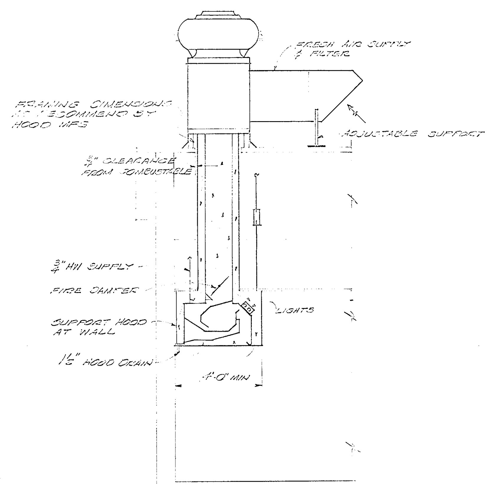
SECTION 1 SCALE - 3/8" = 1'-0"
