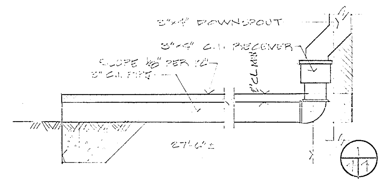
DRAIN DETAIL
