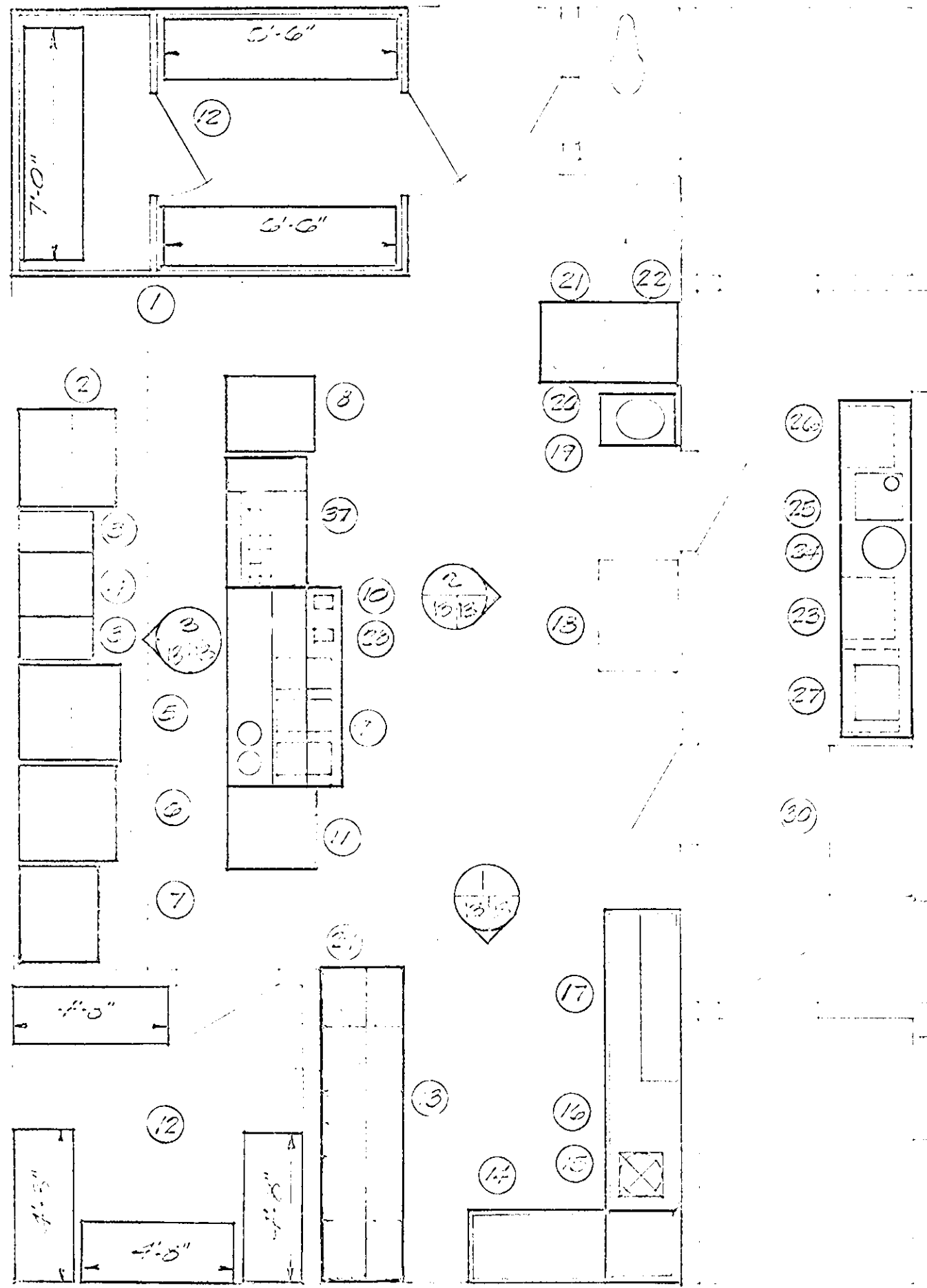
PLAN - KITCHEN & BAR EQUIPMENT SCALE 1/4" = 1'-0"
