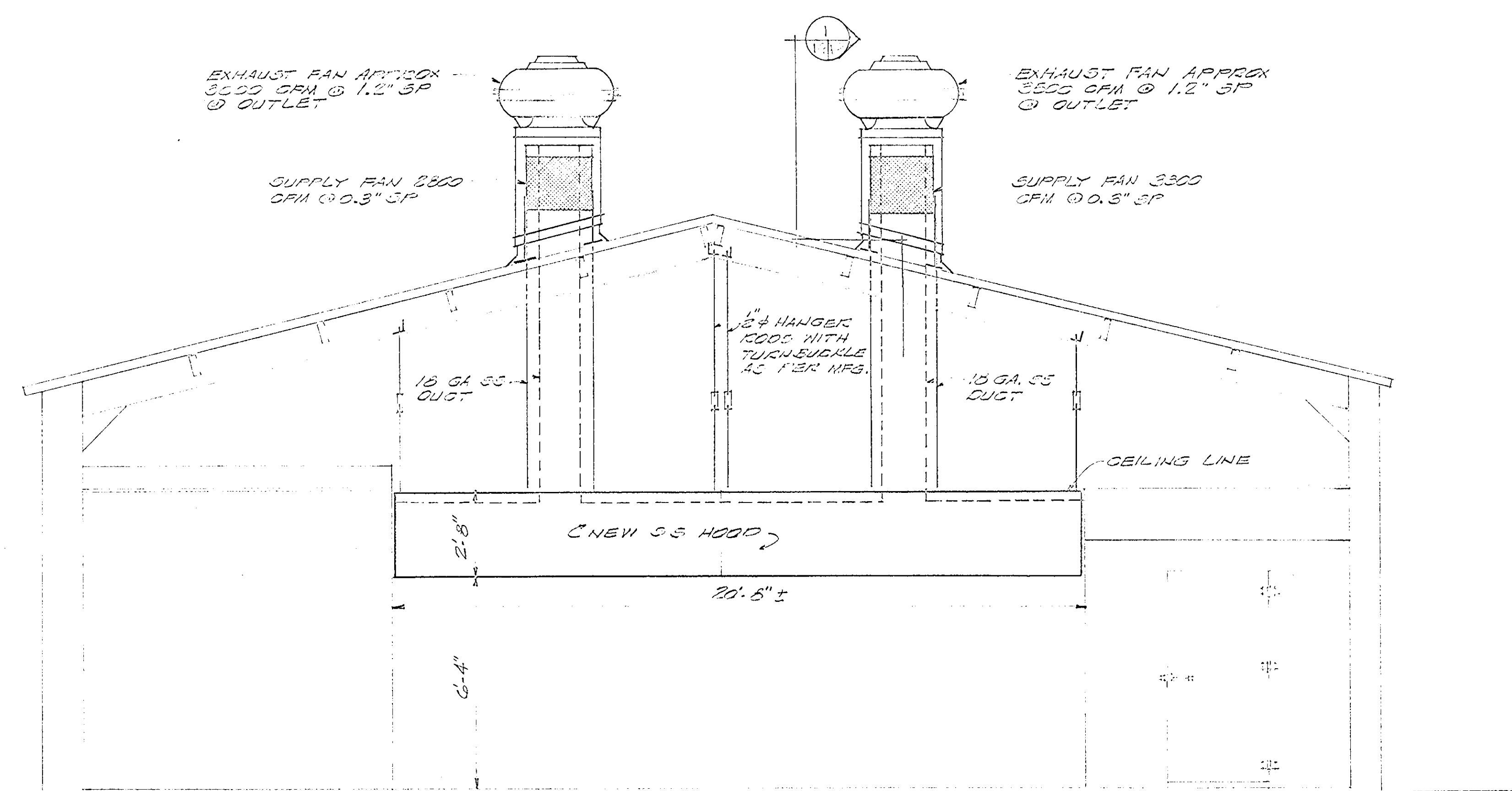
SECTION 0 SCALE - 3/8" = 1'-0"
