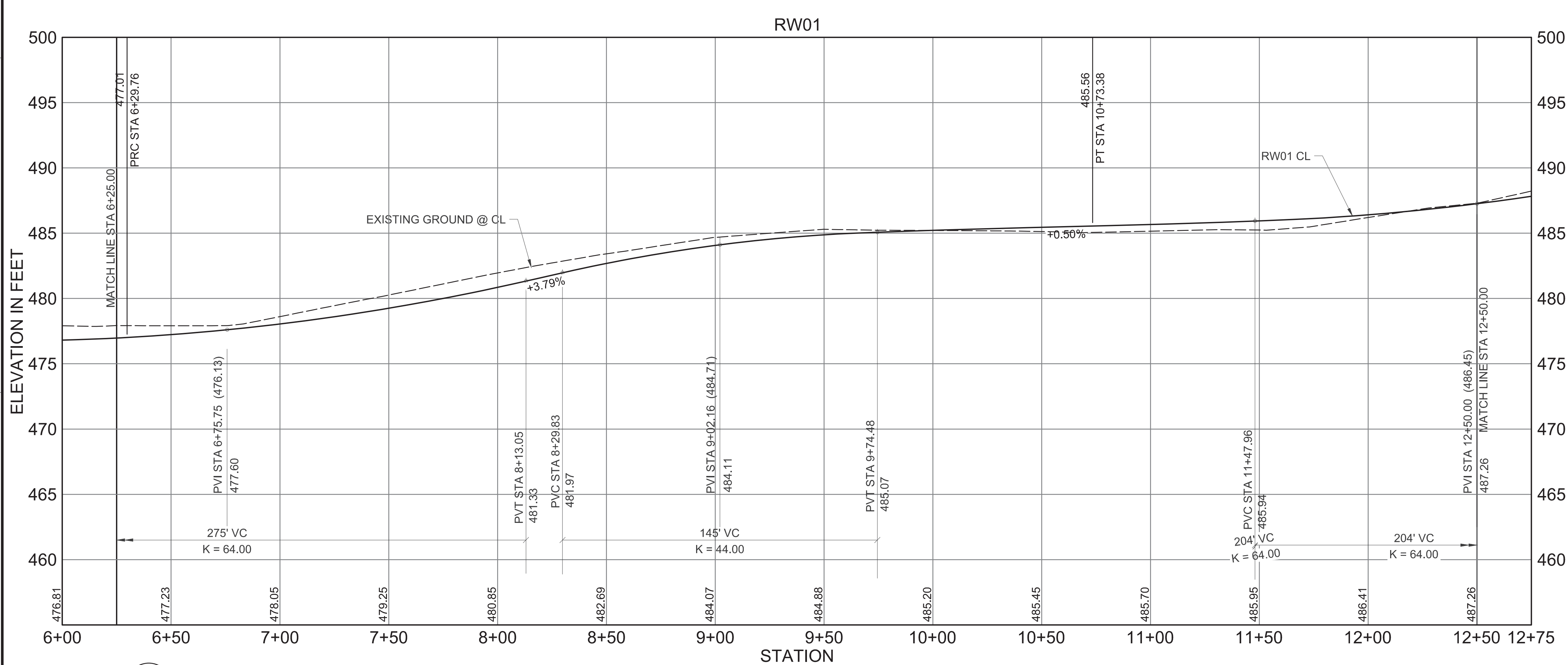
A1 ROADWAY PLAN & PROFILE RW01 STA 6+25-12+50 - AREA 22 & 23 SCALE: HORIZONTAL 1" = 30' VERTICAL 1" = 5'
