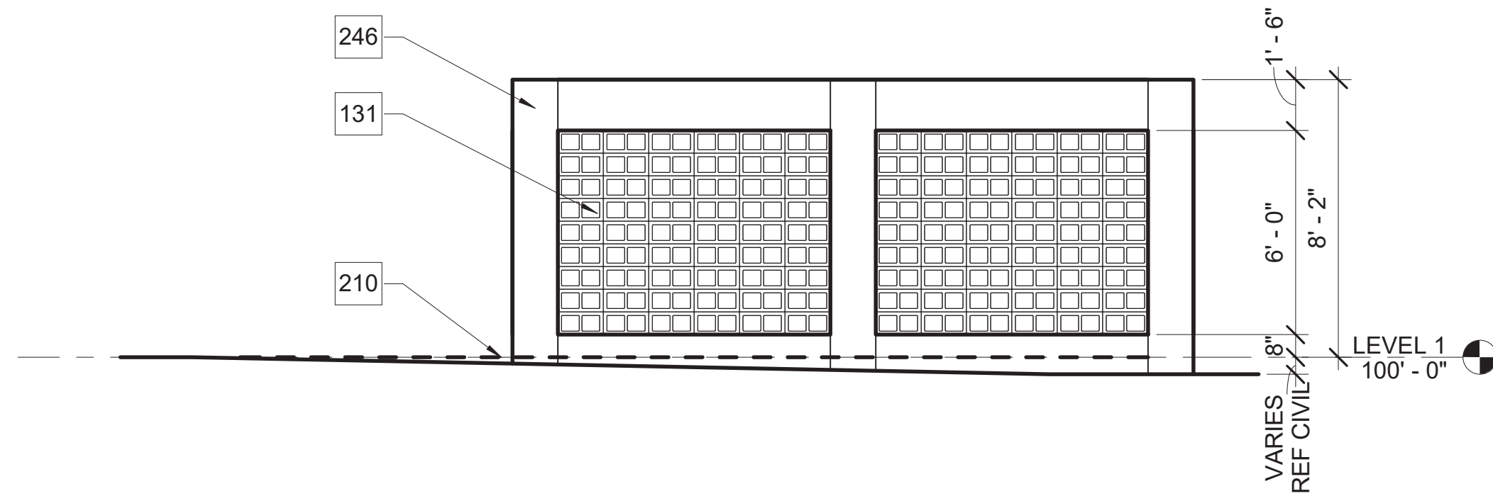
A3 EQUIPMENT YARD - SIDE ELEVATION SCALE 1/4" = 1'-0"
