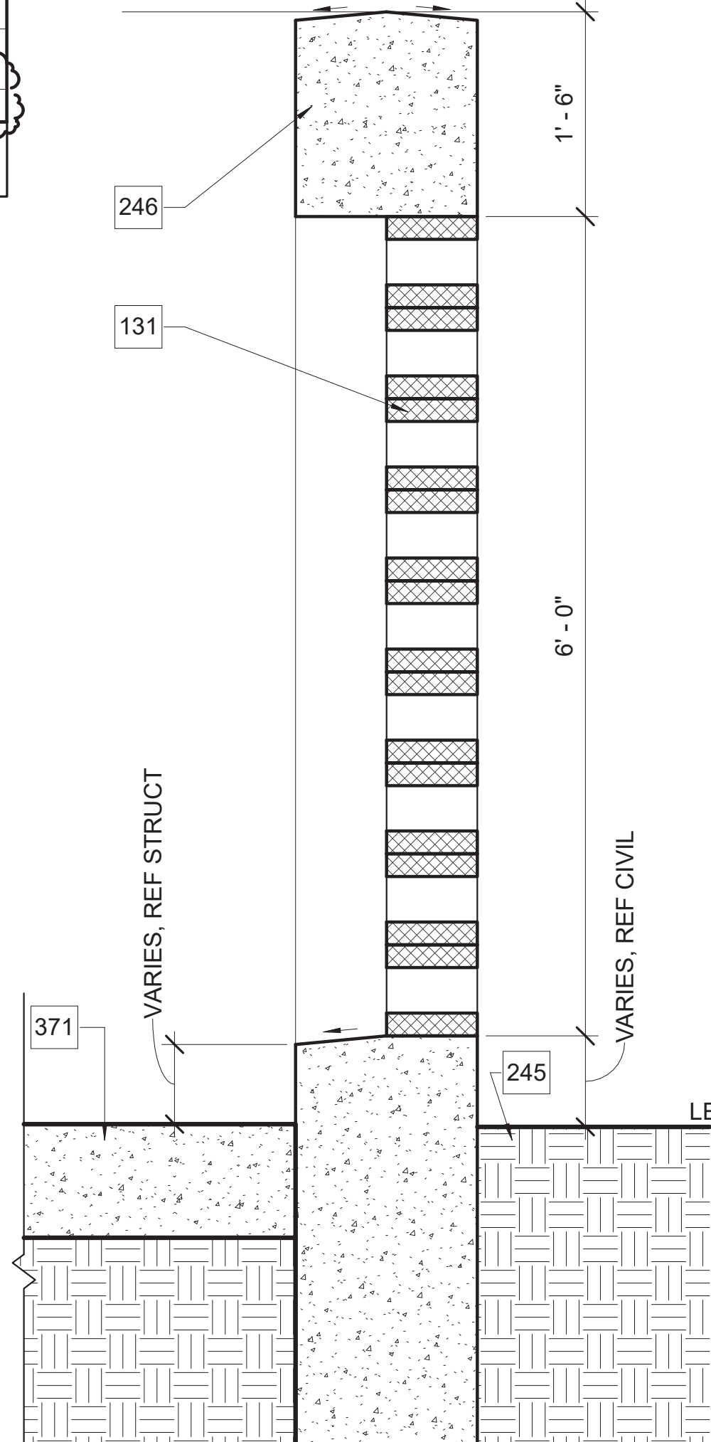
B4 WALL SECTION SCALE NTS
