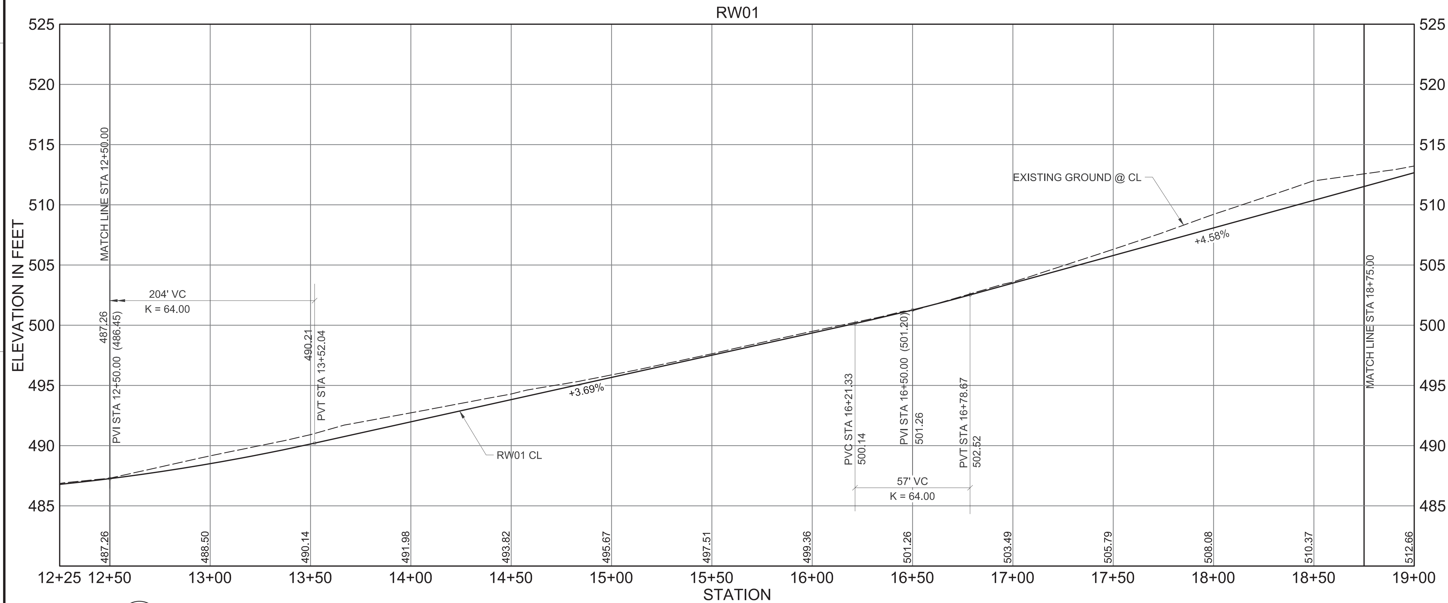
A1 ROADWAY PLAN & PROFILE RW01 STA 12+50-18+75 - AREA 23 & 24 SCALE: HORIZONTAL 1" = 30' VERTICAL 1" = 5'
