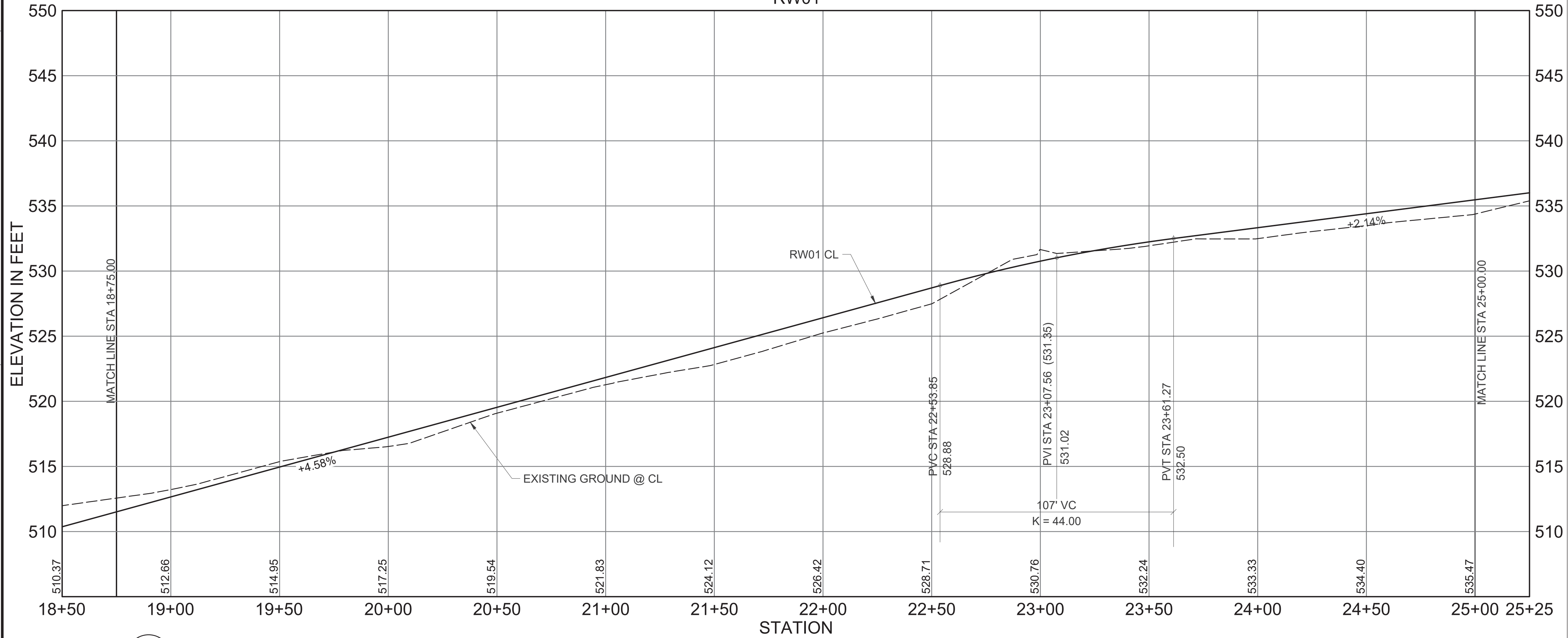
A1 ROADWAY PLAN & PROFILE RW01 STA 18+75-25+00 - AREA 24 & 25 SCALE: HORIZONTAL 1" = 30' VERTICAL 1" = 5'
