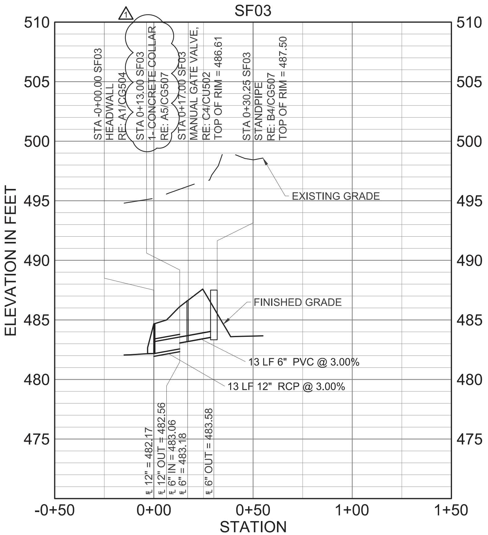
C4 DRAINAGE PROFILES - SF03 SCALE: HORIZONTAL 1" = 30' VERTICAL 1" = 5'
