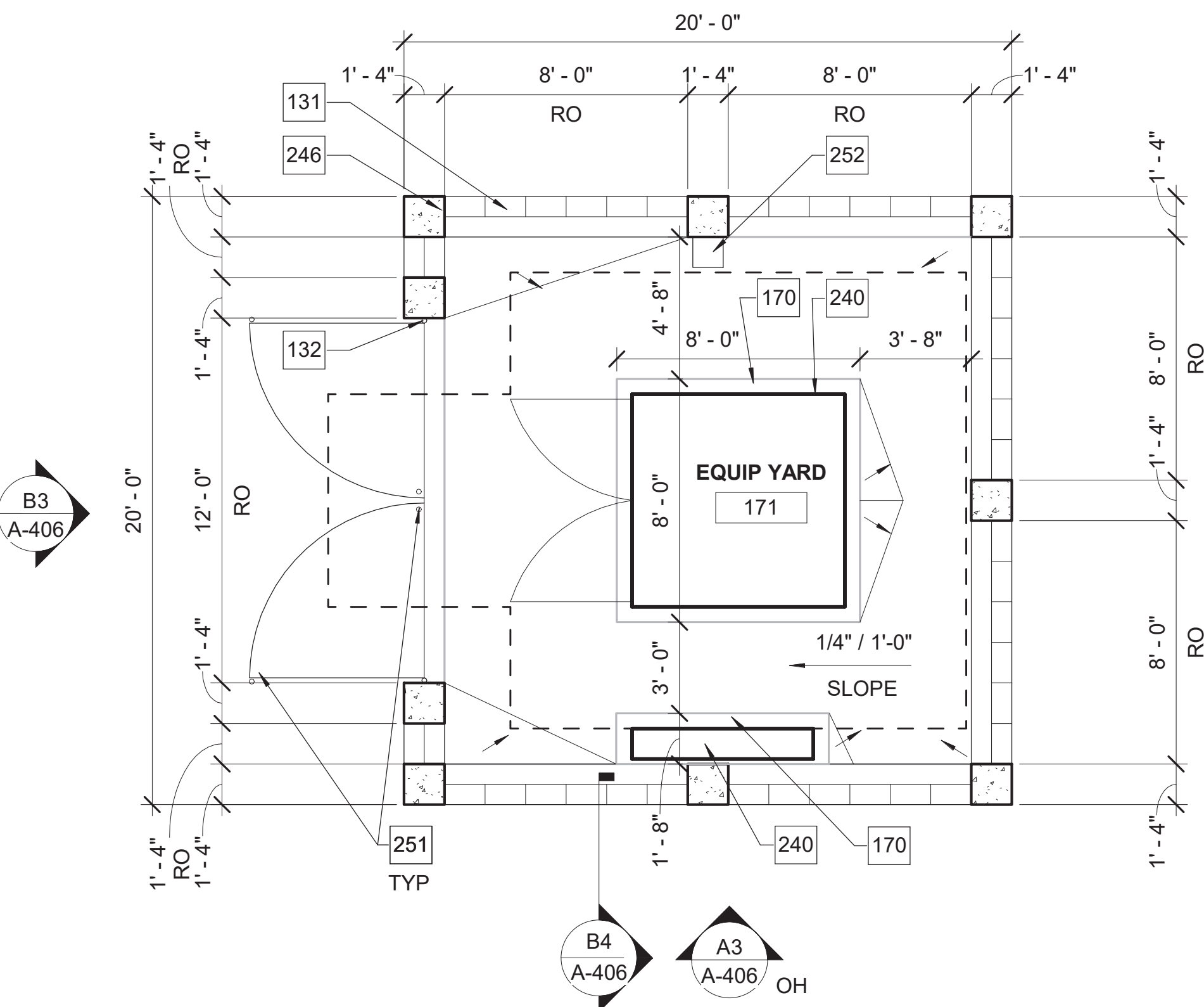
A1 EQUIPMENT YARD - ENLARGED PLAN SCALE 1/4" = 1'-0"
