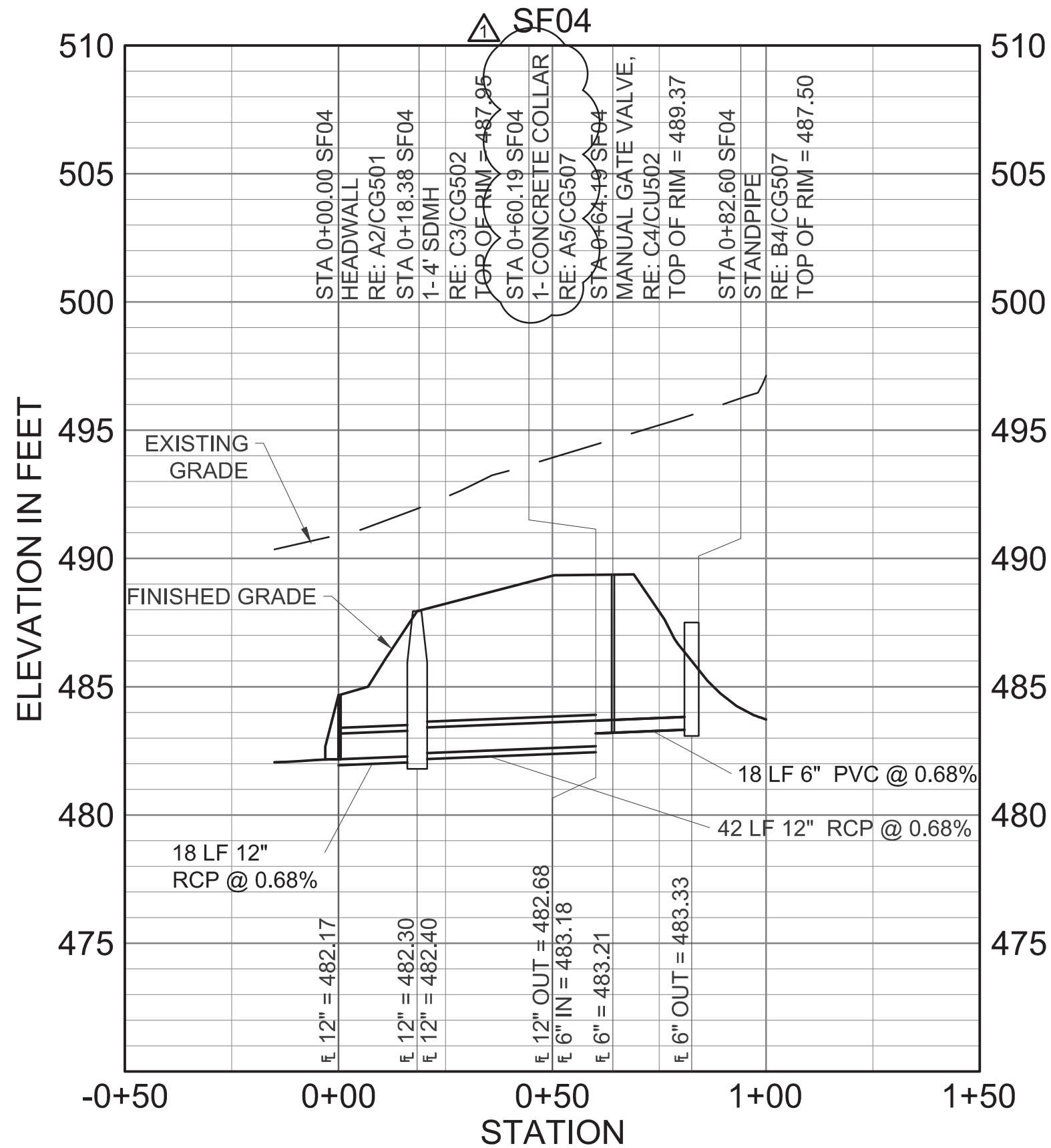
A1 DRAINAGE PROFILES - SF04 SCALE: HORIZONTAL 1" = 30' VERTICAL 1" = 5'
