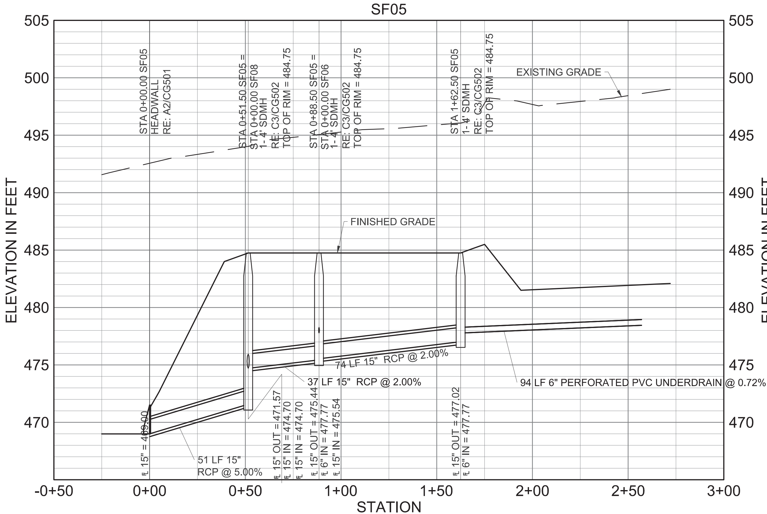
A3 DRAINAGE PROFILES - SF05 SCALE: HORIZONTAL 1" = 30' VERTICAL 1" = 5'
