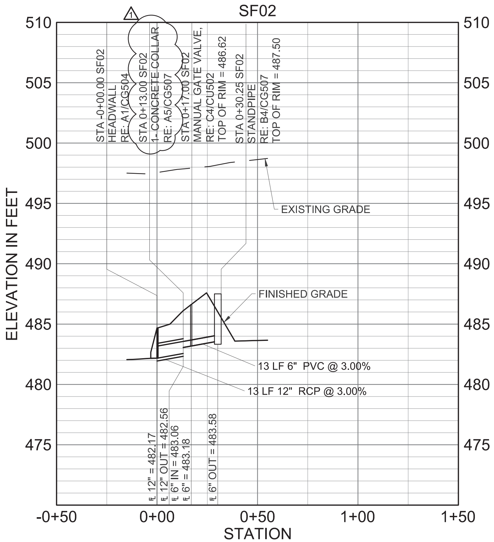
C3 DRAINAGE PROFILES - SF02 SCALE: HORIZONTAL 1" = 30' VERTICAL 1" = 5'
