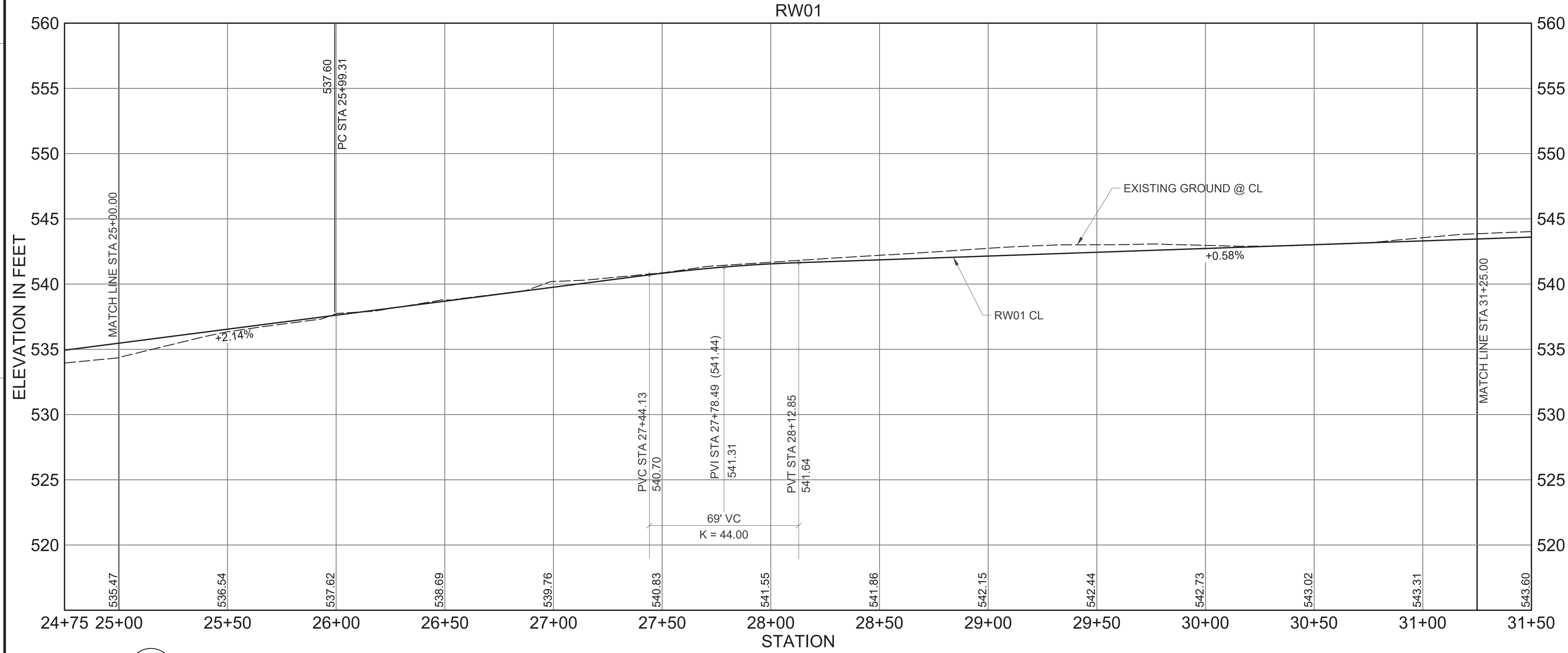
A1 ROADWAY PLAN & PROFILE RW01 STA 25+00-31+25 - AREA 25 & 26 SCALE: HORIZONTAL 1" = 30' VERTICAL 1" = 5'
