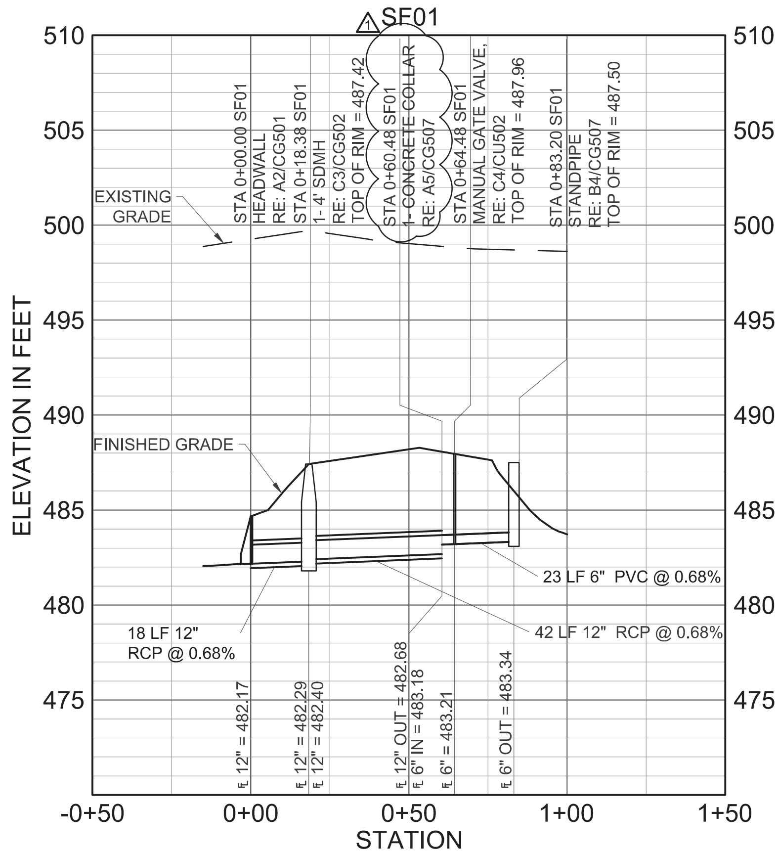
C1 DRAINAGE PROFILES - SF01 SCALE: HORIZONTAL 1" = 30' VERTICAL 1" = 5'
