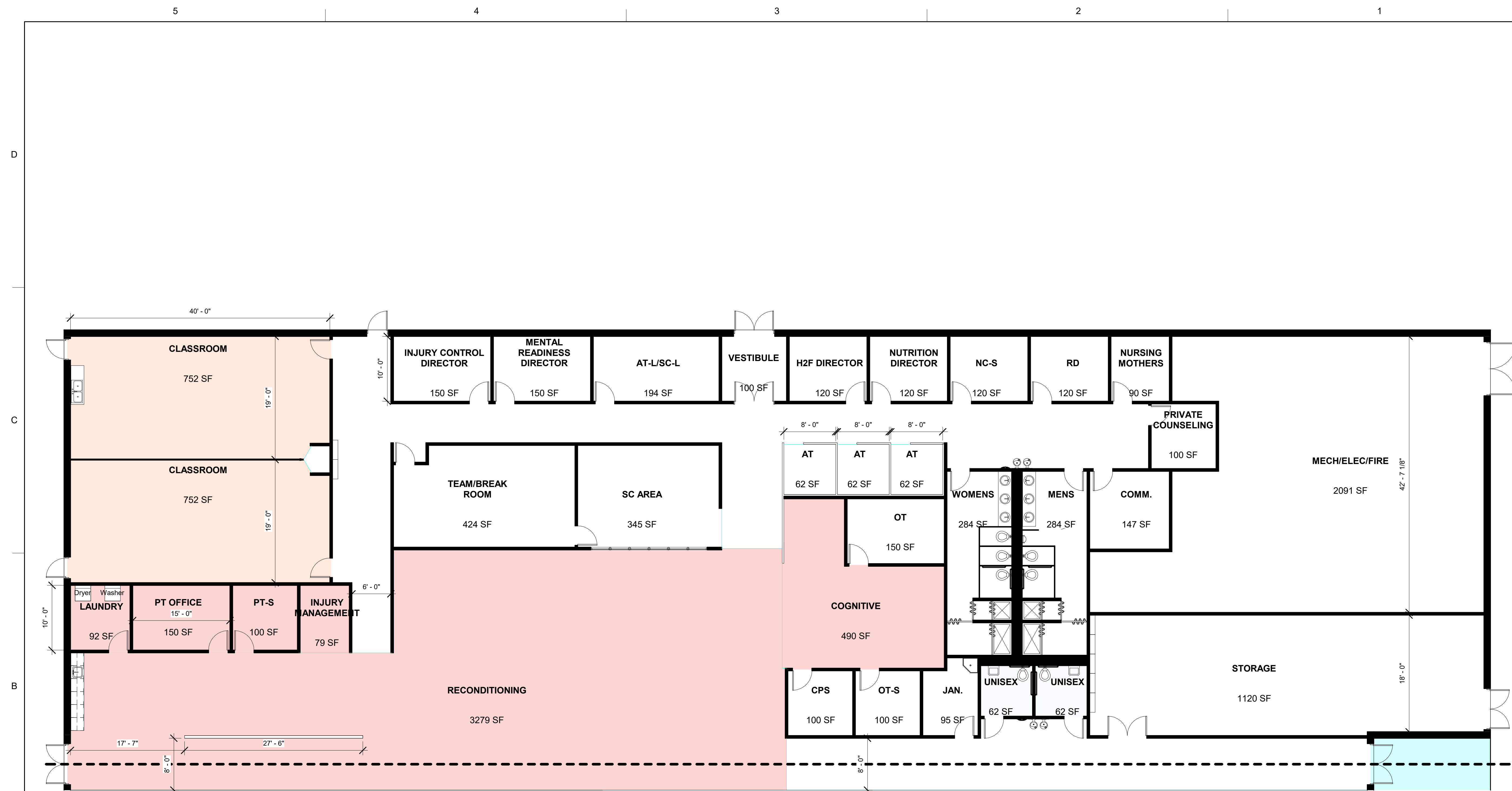
ENLARGED FLOOR PLAN - A
