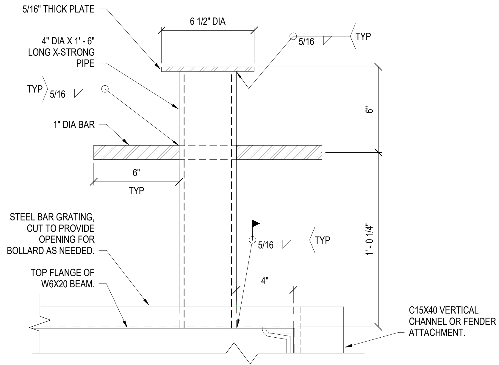
B3 DETAIL - BOLLARD CONNECTION NOT TO SCALE (S-101)
