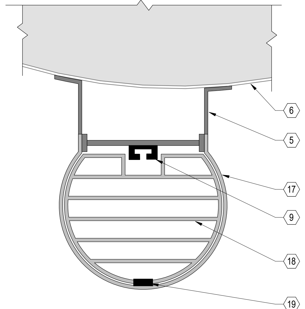
A3 STEEL SECURITY CAGE AND HATCH NOT TO SCALE (S-301)
