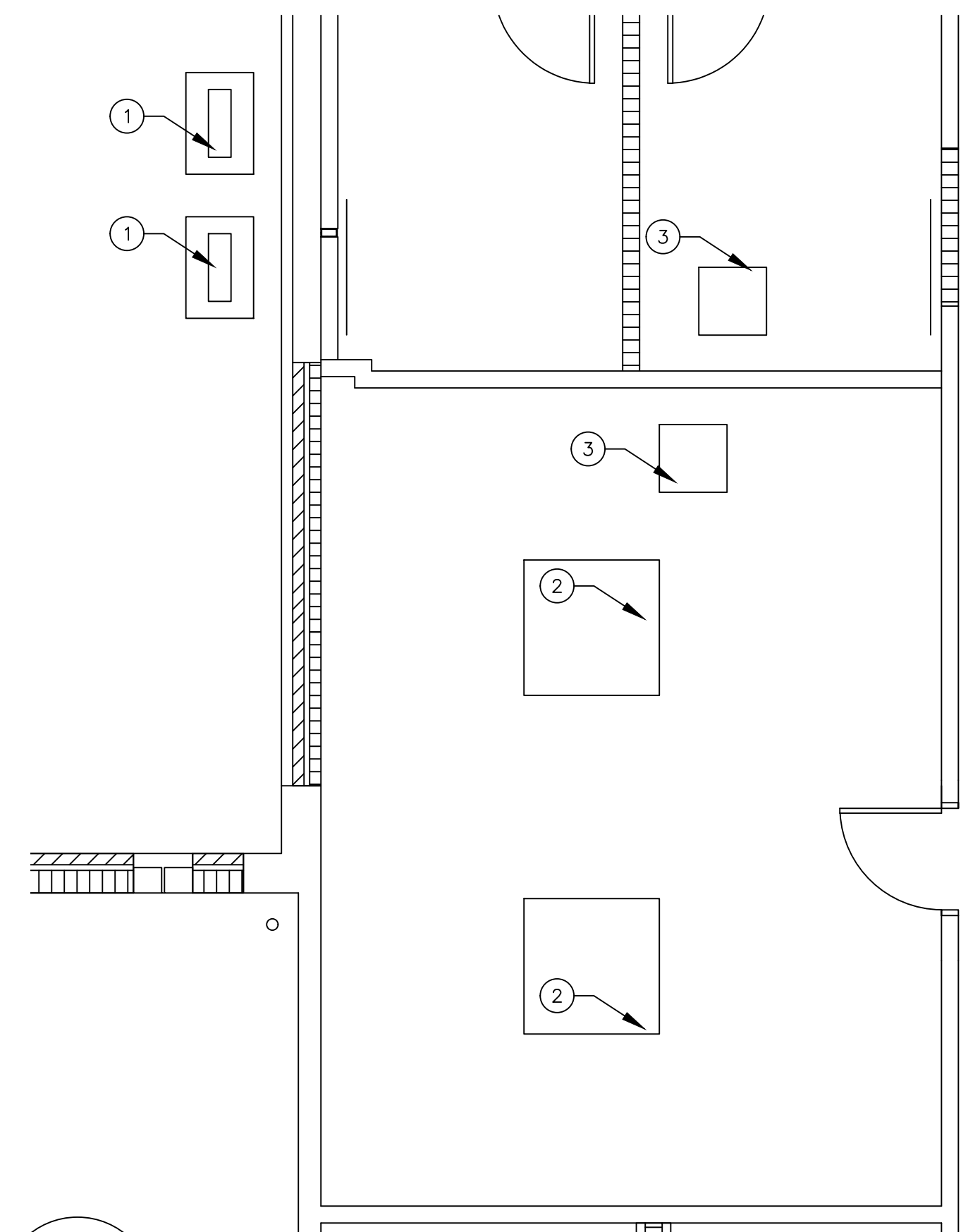
2 M1 SERVER ROOM MECHANICAL RENO PLAN 1/4" = 1'-0" 0 5' 10'
