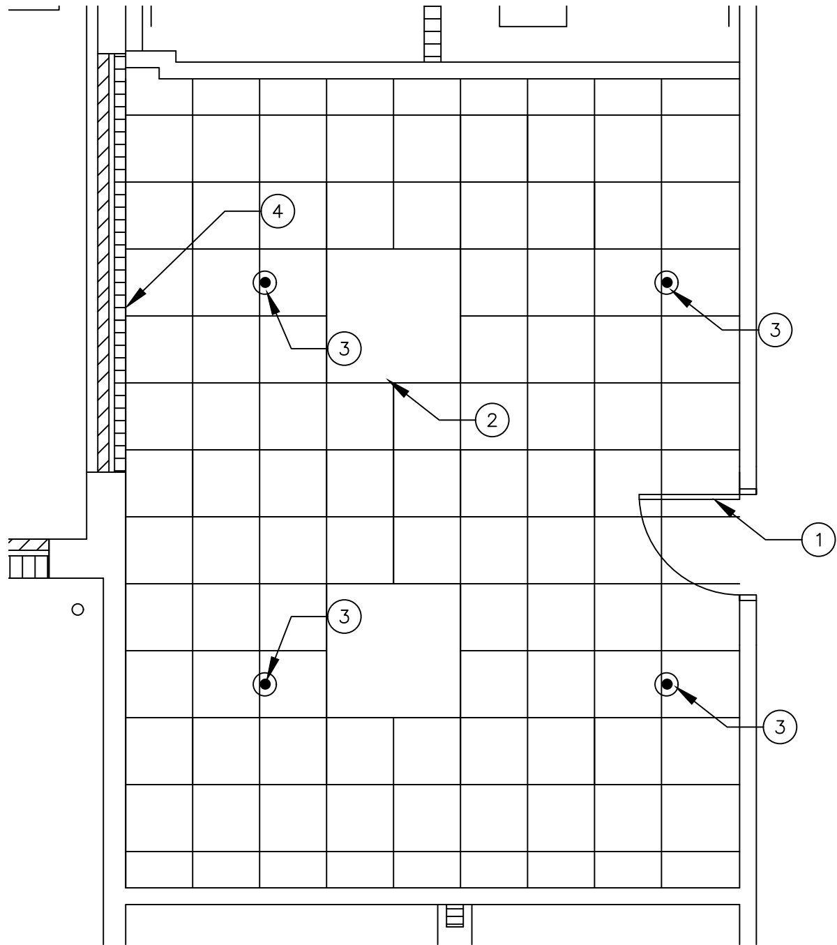
2 A2 SERVER ROOM RENO PLAN 1/4" = 1'-0" 0 5' 10'
