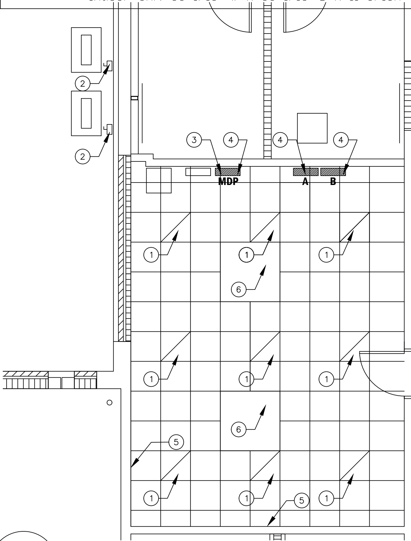
SERVER ROOM ELECTRICAL RENO PLAN
