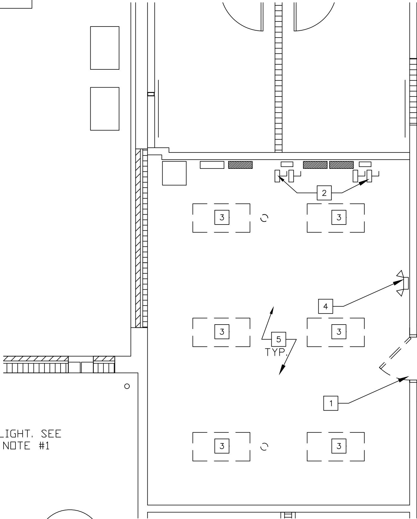
SERVER ROOM ELECTRICAL DEMO PLAN
