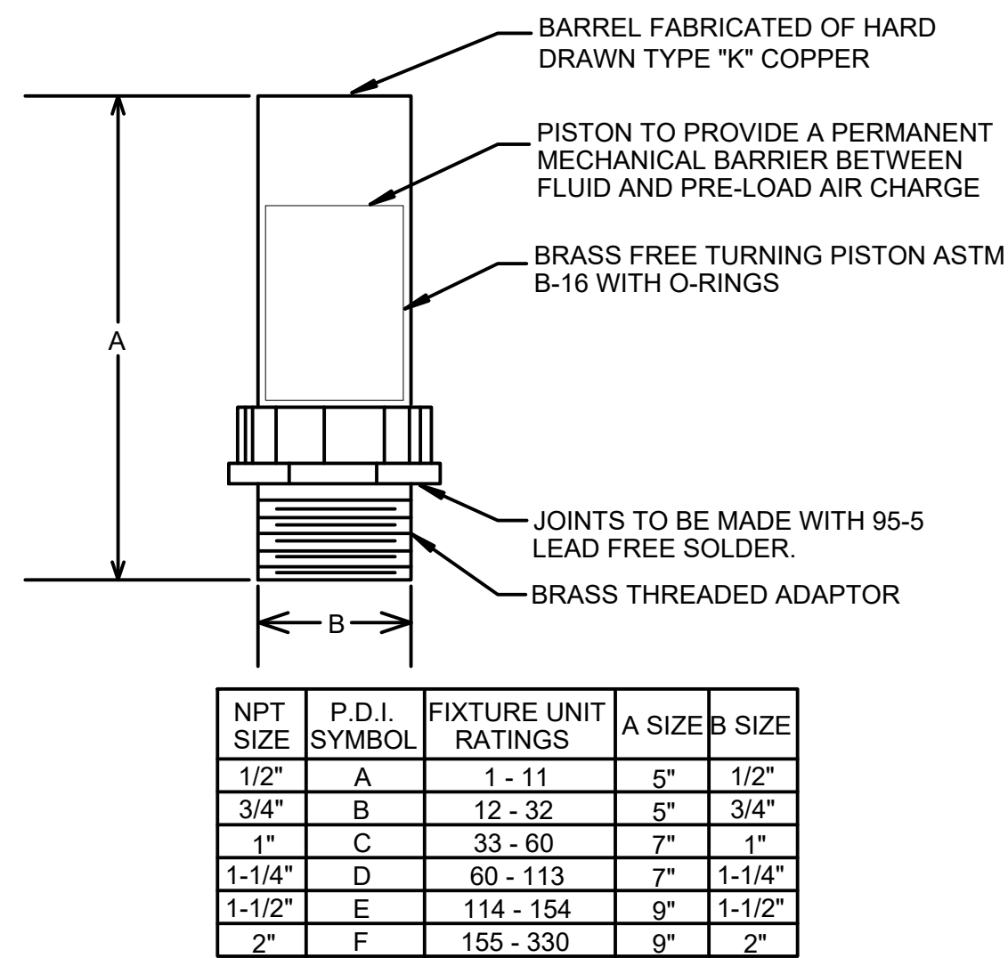
B1 SHOCK ABSORBER DETAIL NTS
