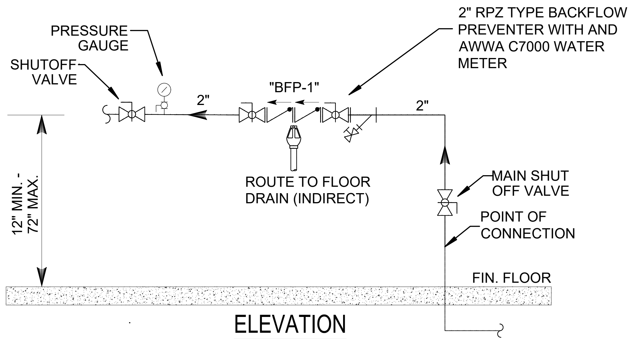
A1 BACKFLOW PREVENTER DETAIL (BFP-1) NTS
