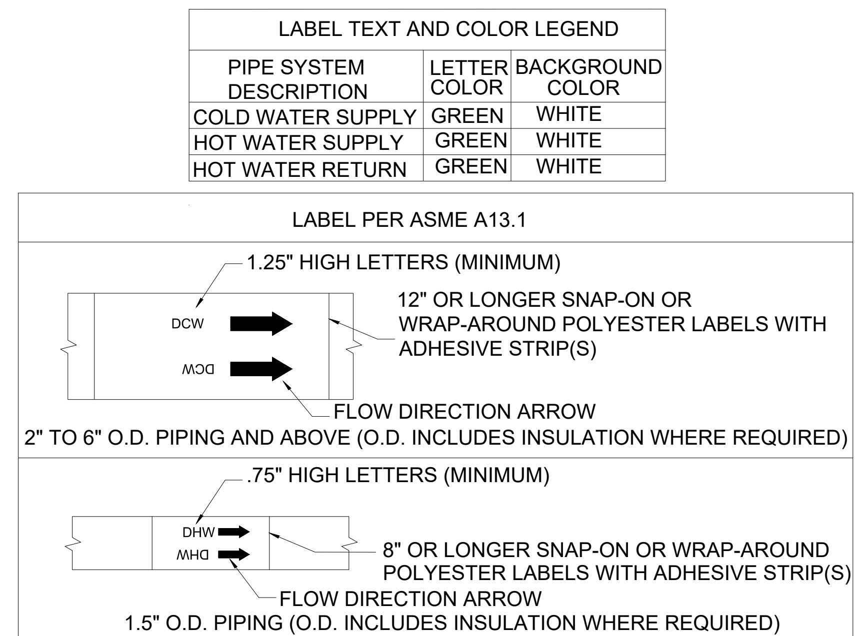
C1 PIPE LABELING DETAIL NTS
