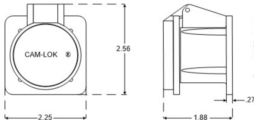
SNAPBACK ENCLOSURE ASSEMBLY
