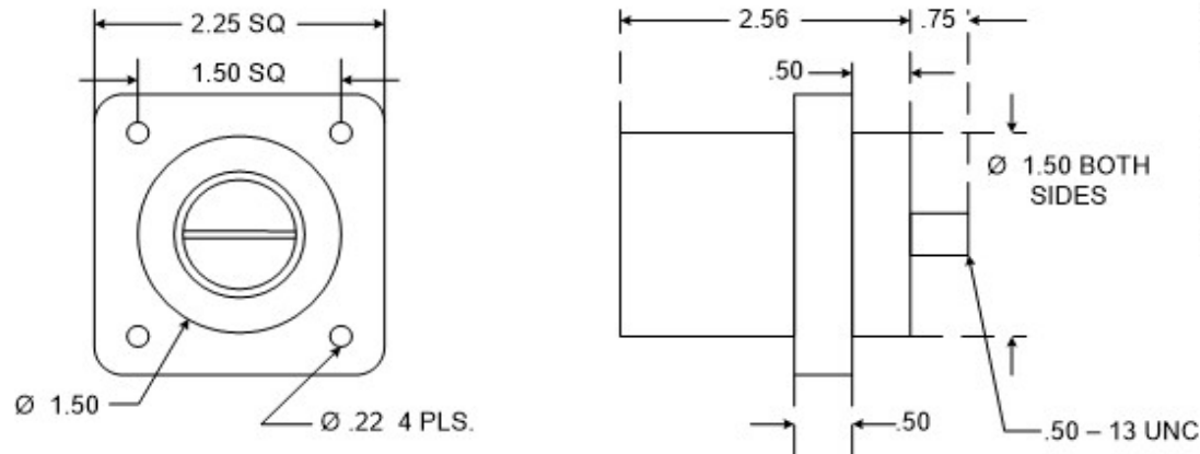
MALE RECEPTACLE 3/4" STUD
