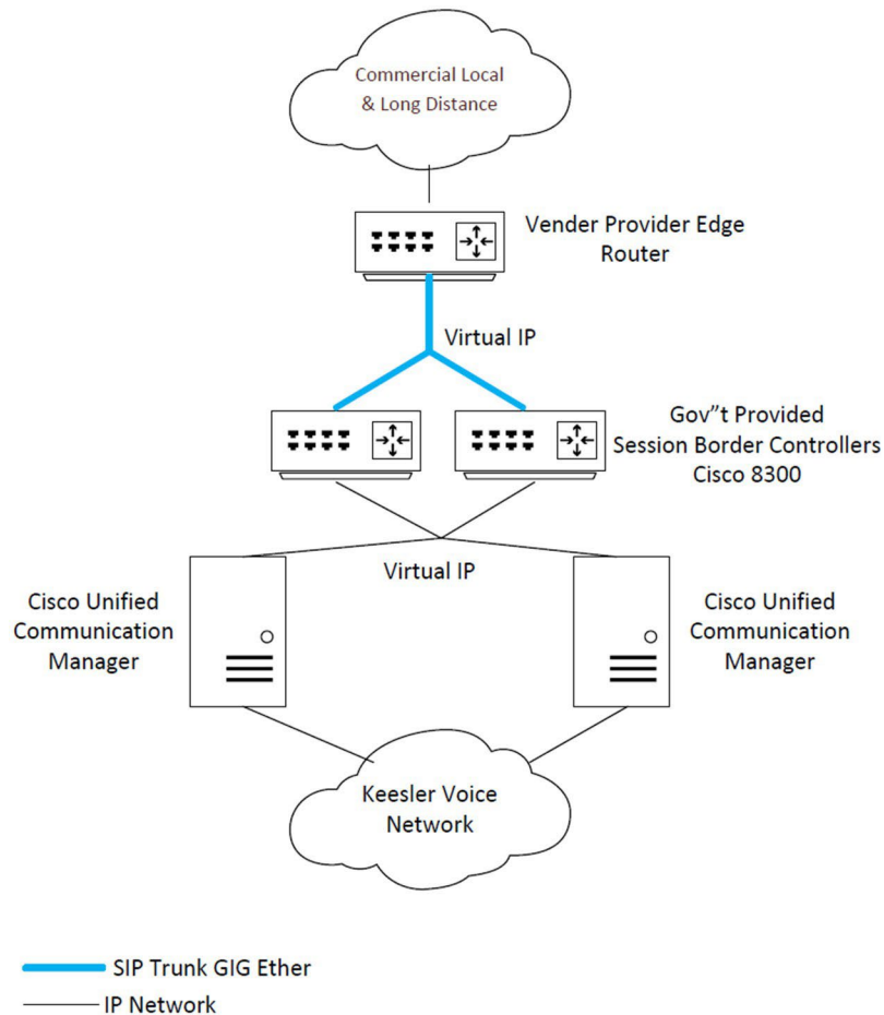
Diagram 2 UTILIZING SIP TRUNKING
