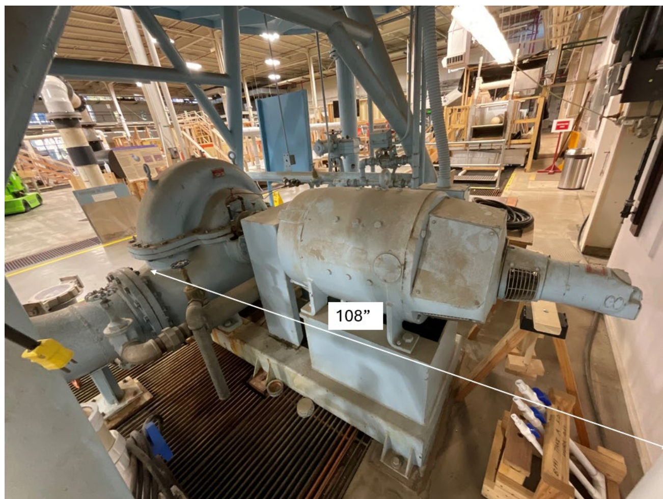
Figure 6. Pump and 100 hp motor to be replaced with the approximate distance from the centerline of the pump piping connections to the back wall.
