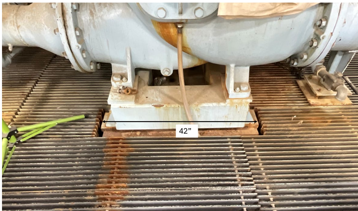
Figure 7. Approximate width dimension of the existing base plate.
