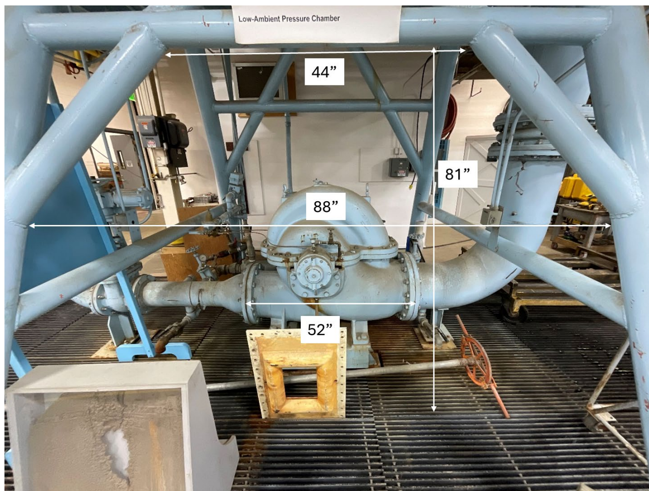
Figure 5. 4,500 gpm pump to be replaced with approximate dimensions of space constraints beneath the chamber.
