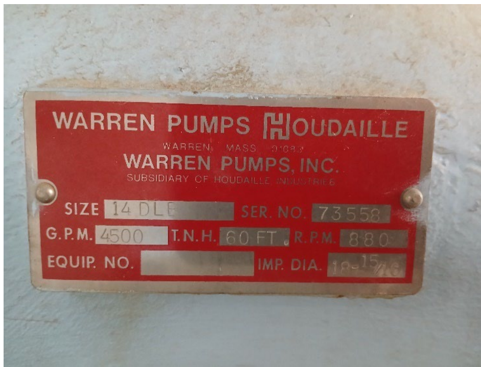
Figure 2. Nameplate of existing 4,500 gpm pump to be replaced.
