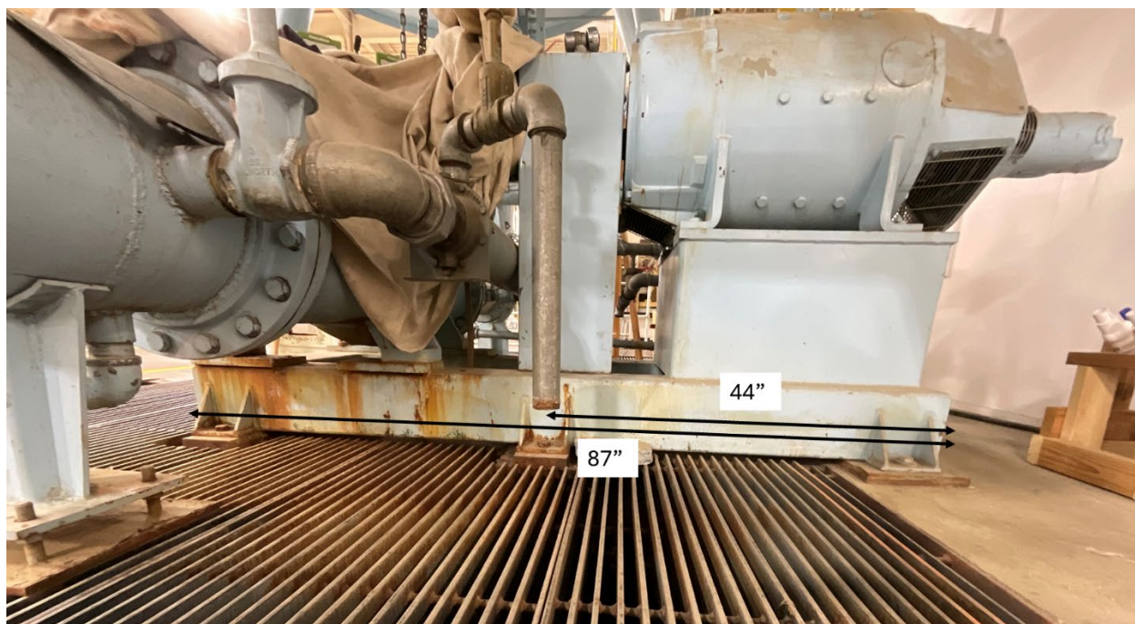
Figure 8. Approximate length dimension of the existing base and mid span support.
