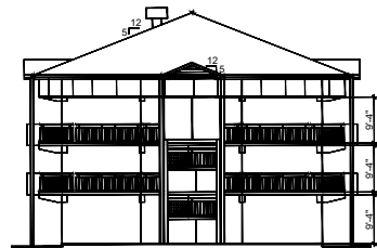
BLDG. HP275 - EAST/WEST ELEVATION - EXISTING CONDITIONS NTS
