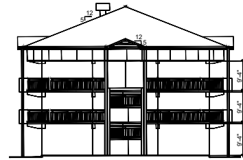
1 BLDG. HP285 - NORTH/SOUTH ELEVATION - EXISTING CONDITIONS NTS
