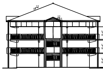
1 BLDG. HP295 - NORTH/SOUTH ELEVATION - EXISTING CONDITIONS NTS
