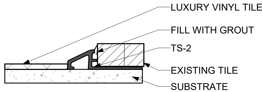
C3 LVT TO TILE DETAIL SCALE: 12" = 1'-0"
