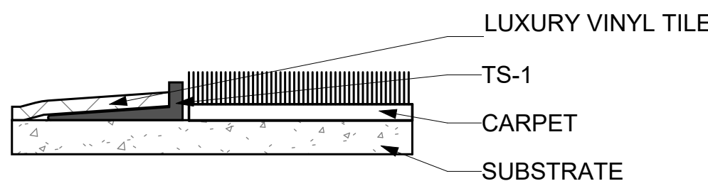
B3 LVT TO CARPET DETAIL SCALE: 12" = 1'-0"
