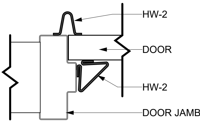
B1 FINGER PINCH GUARD DETAIL SCALE: 3" = 1'-0"
