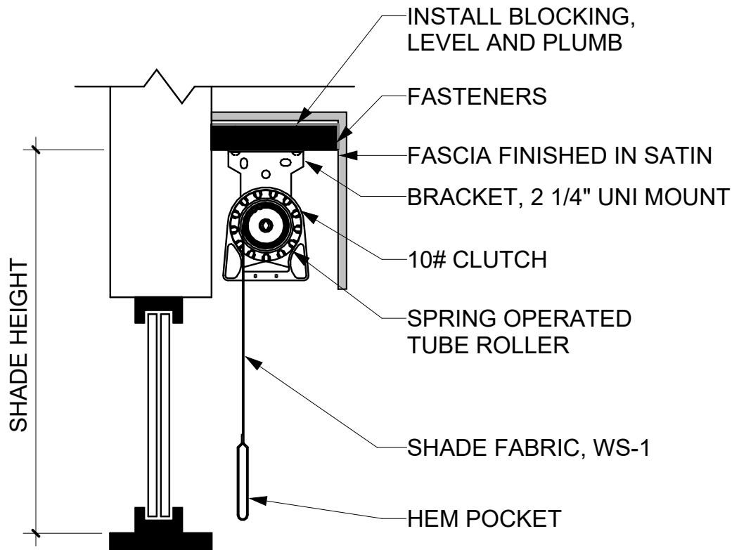
C1 SINGLE ROLLER SHADE DETAIL SCALE: 3" = 1'-0"
