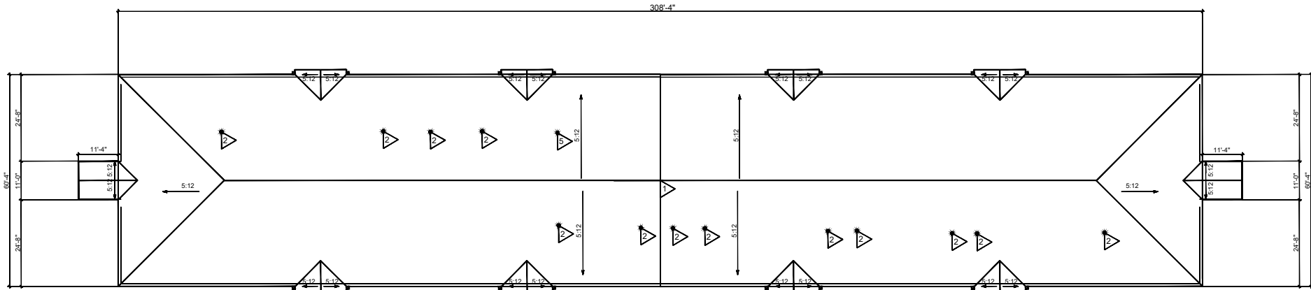
BLDG. HP245 - ROOF PLAN - EXISTING CONDITIONS NTS
