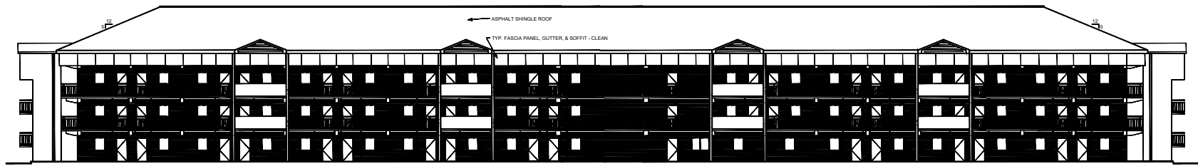
BLDG. HP235 - SOUTH ELEVATION - EXISTING CONDITIONS NTS
