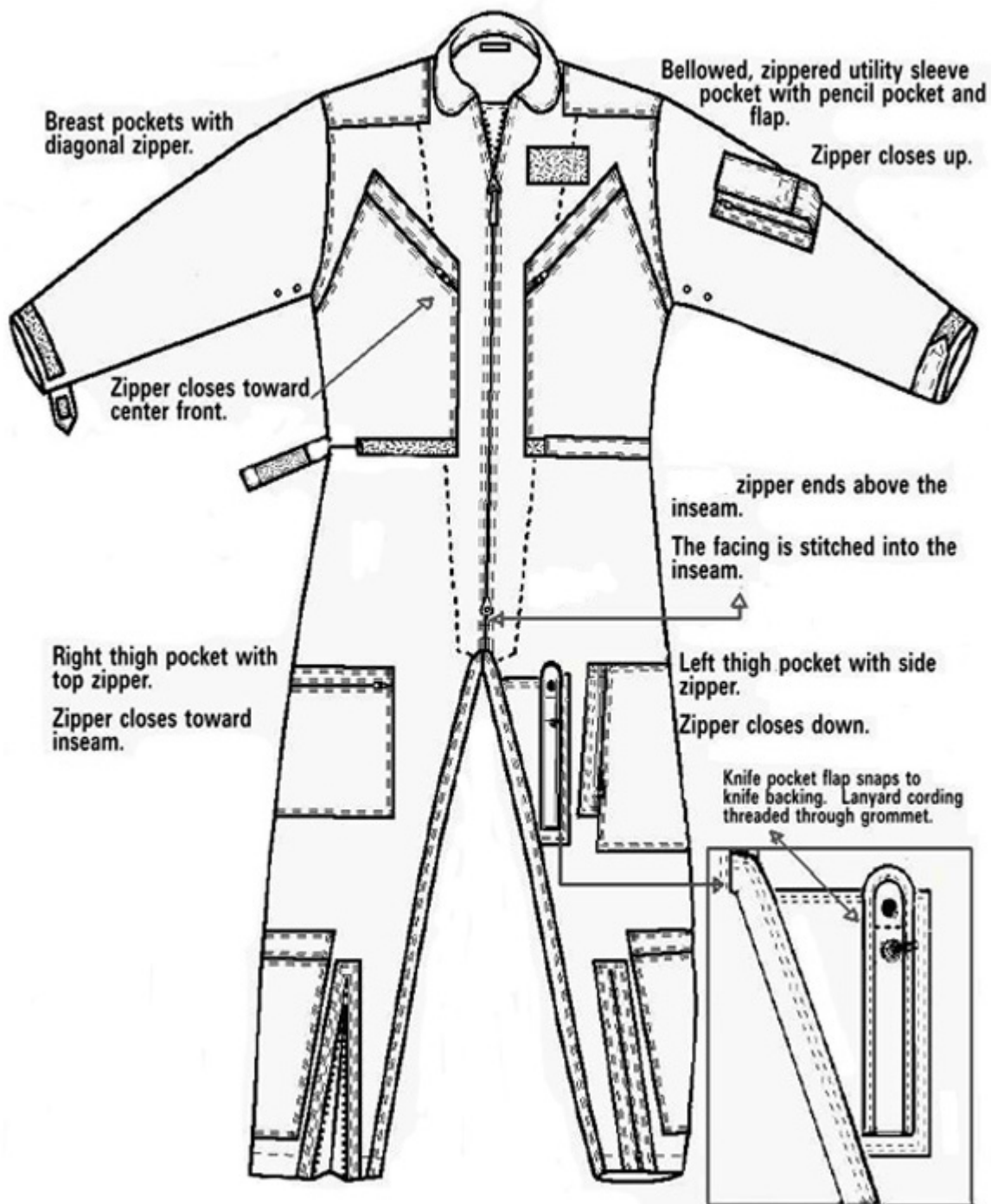
Figure 1. Coverall Front View
