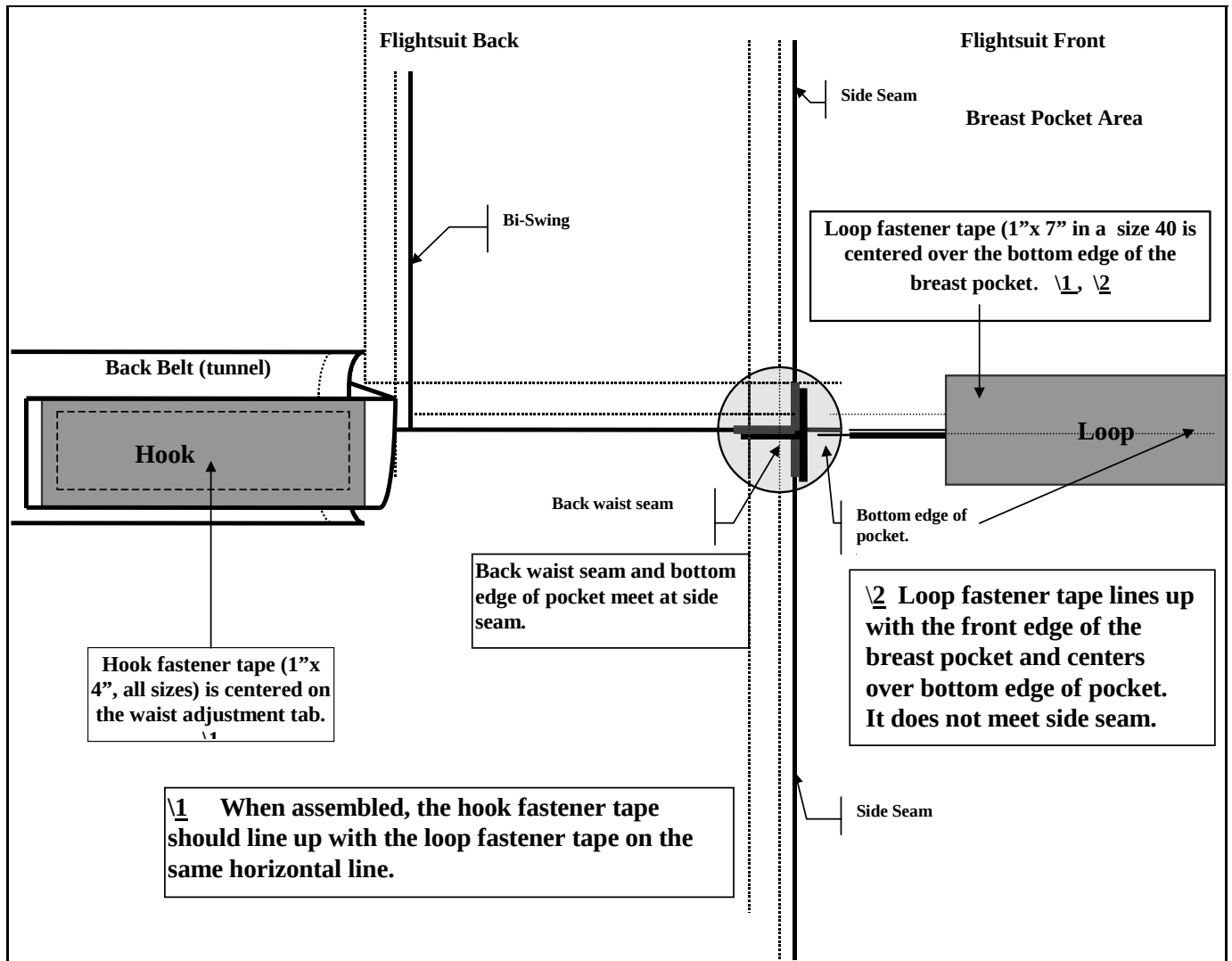
Figure 10. Detail: bottom of breast pocket to align with back waist seam
