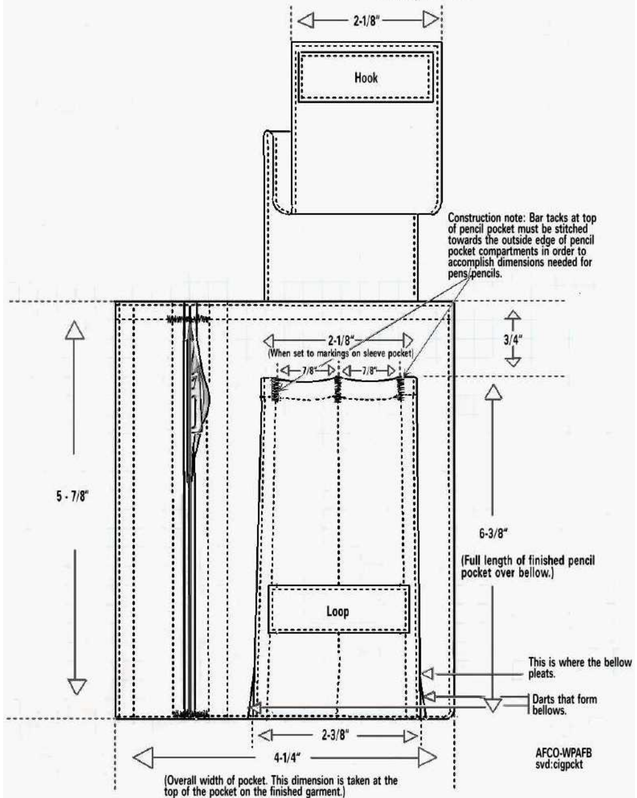
Figure 5., Sleeve Pocket/Pencil Pocket Configuration
