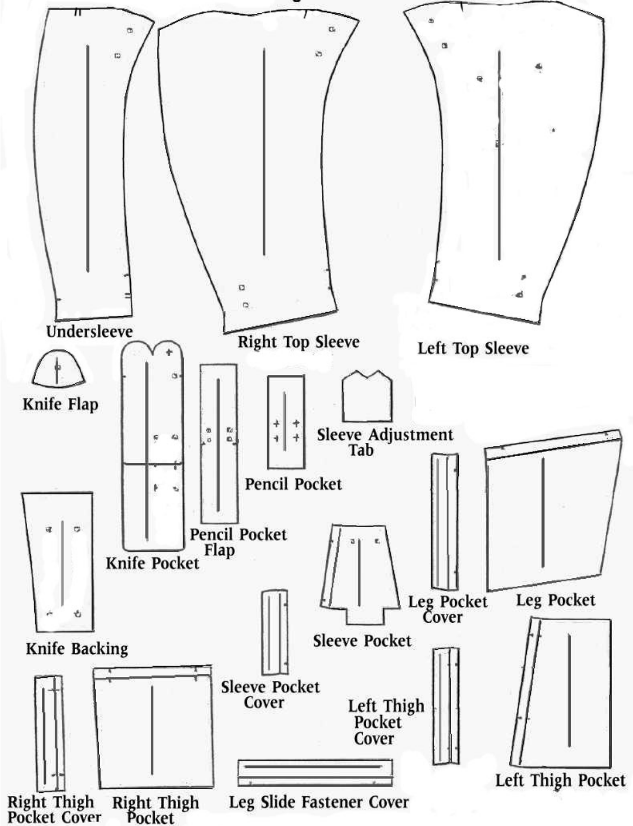
Figure 13. General Pattern Guide
