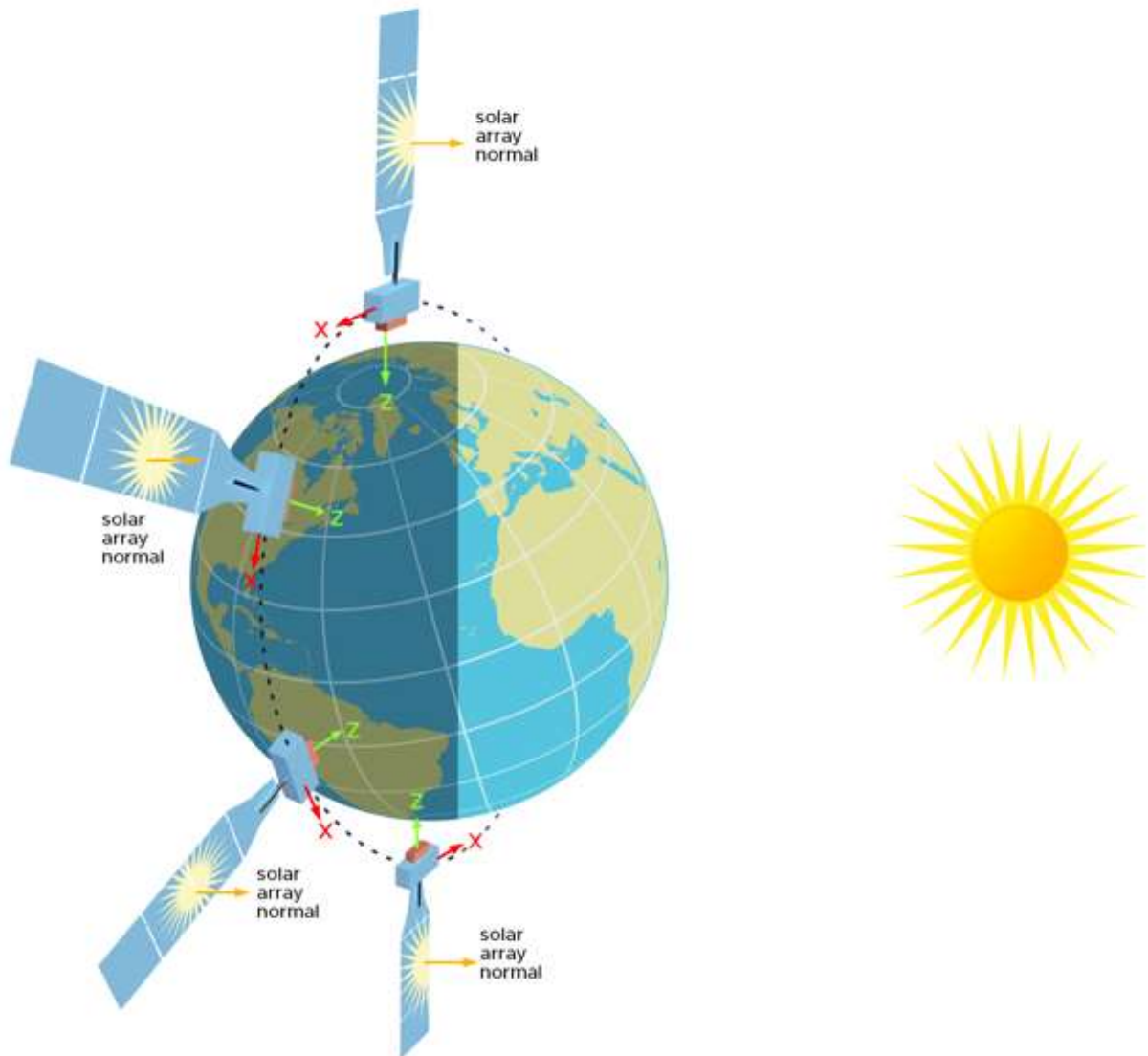
Figure 5.6.1-4. Typical Spacecraft Configuration for Engineering Mode and Science Operations Mode
