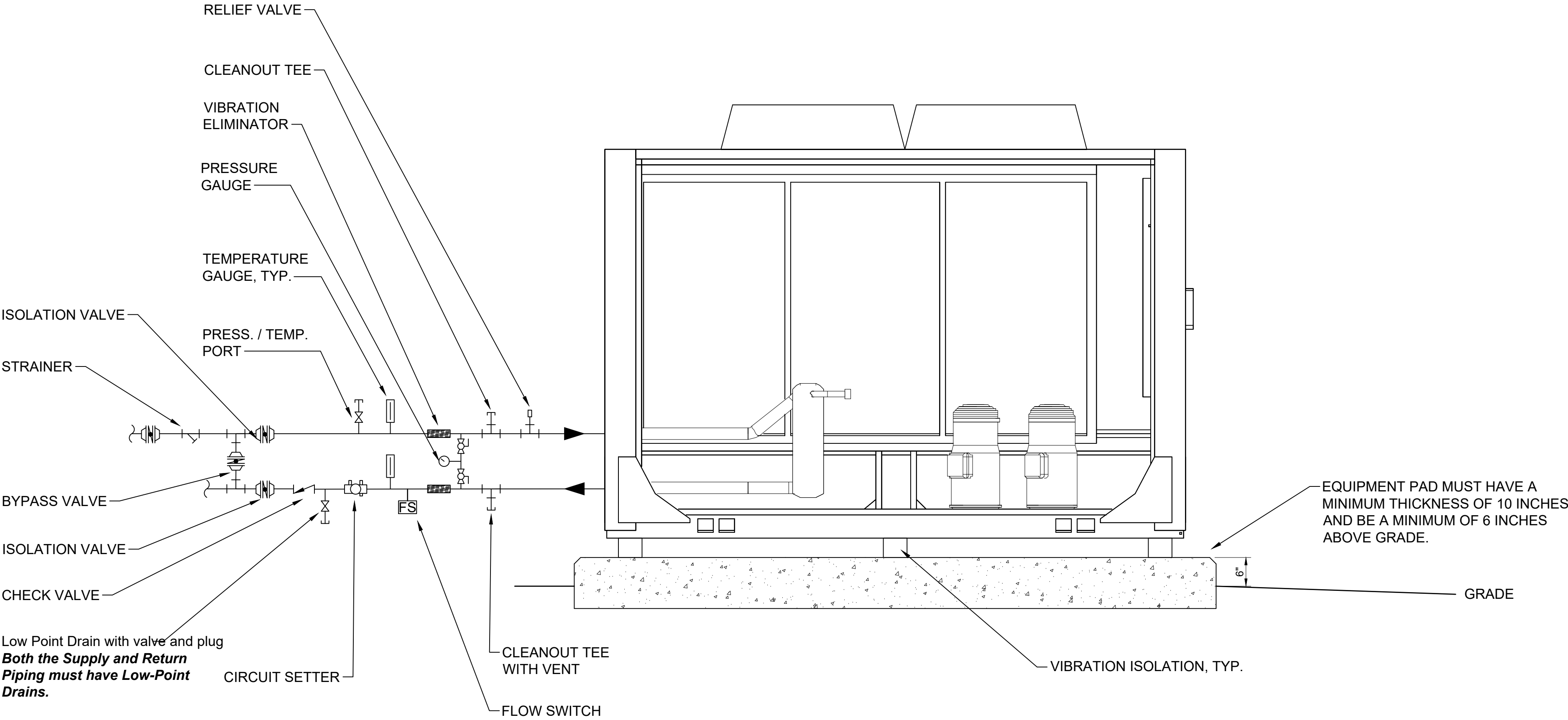
1 CHILLER DETAIL NOT TO SCALE
