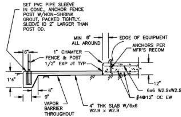
1 M1M1 CONCRETE PAD SECTION SCALE 1/2"=1'-0"
