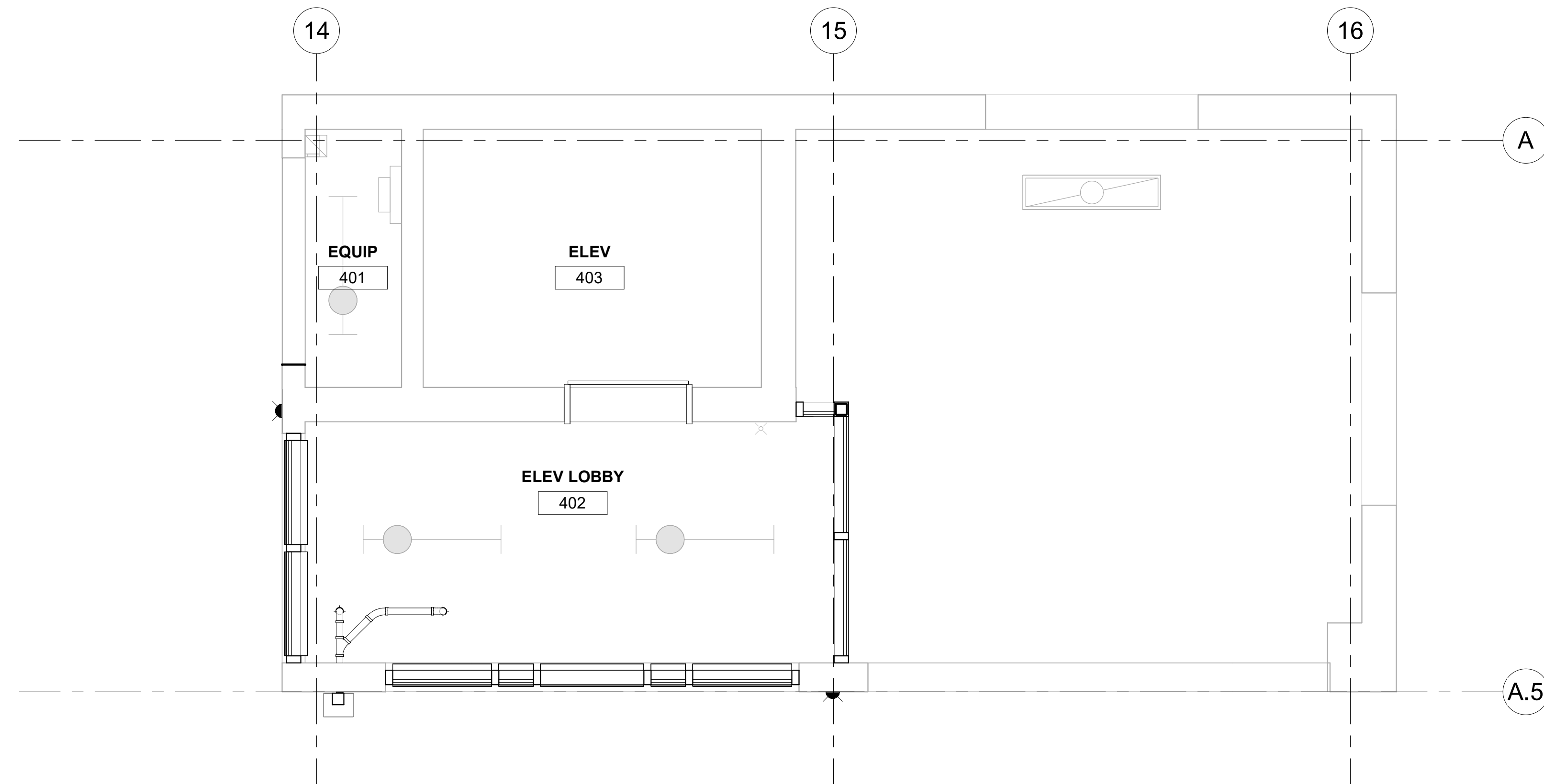
2 LEVEL 4 - ELEVATOR LOBBY - ENLARGED RCP 3/8" = 1'-0"
