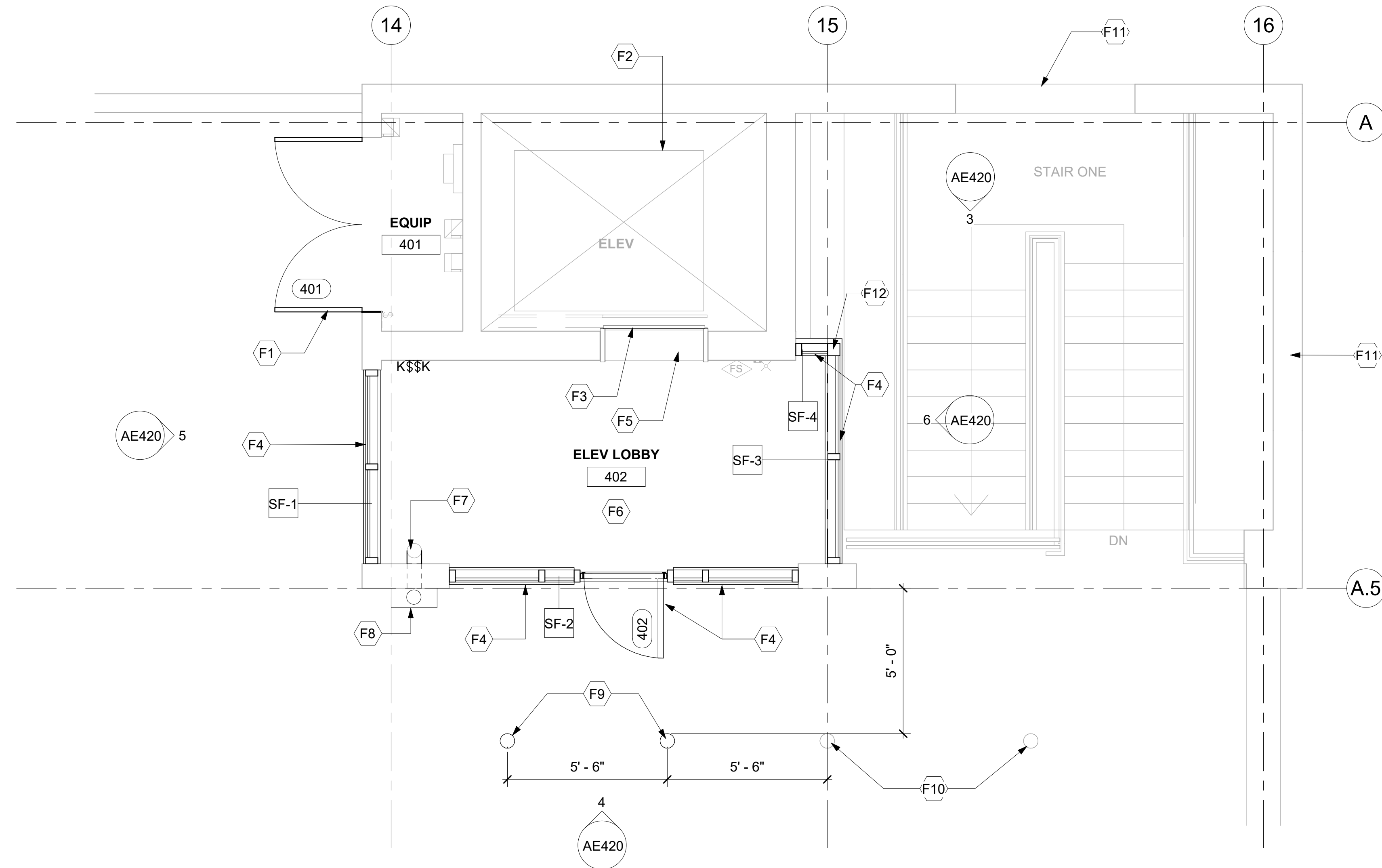
1 LEVEL 4 - ELEVATOR LOBBY - ENLARGED PLAN 3/8" = 1'-0"
