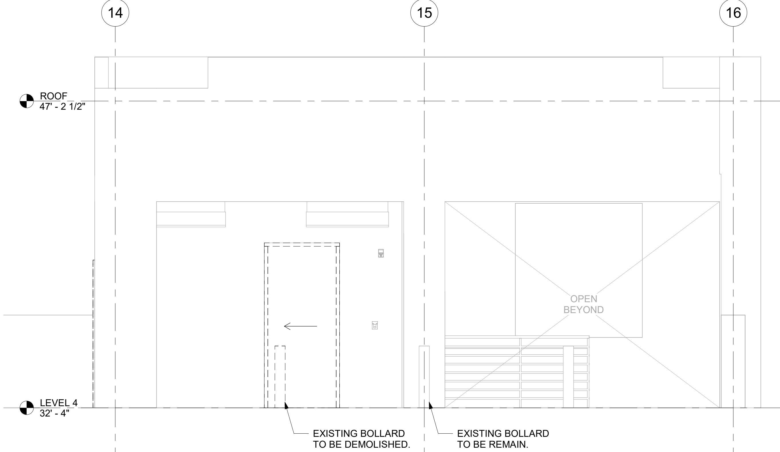
1 ELEVATOR LOBBY - SOUTH ELEVATION - EXISTING CONDITIONS 3/8" = 1'-0"
