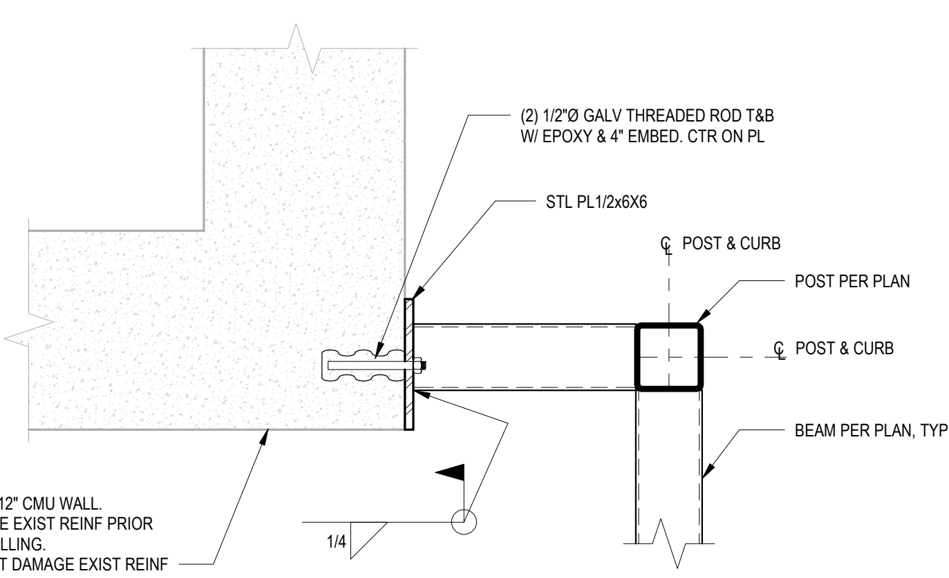
E3 POST BASE 1 1/2" = 1'-0"
