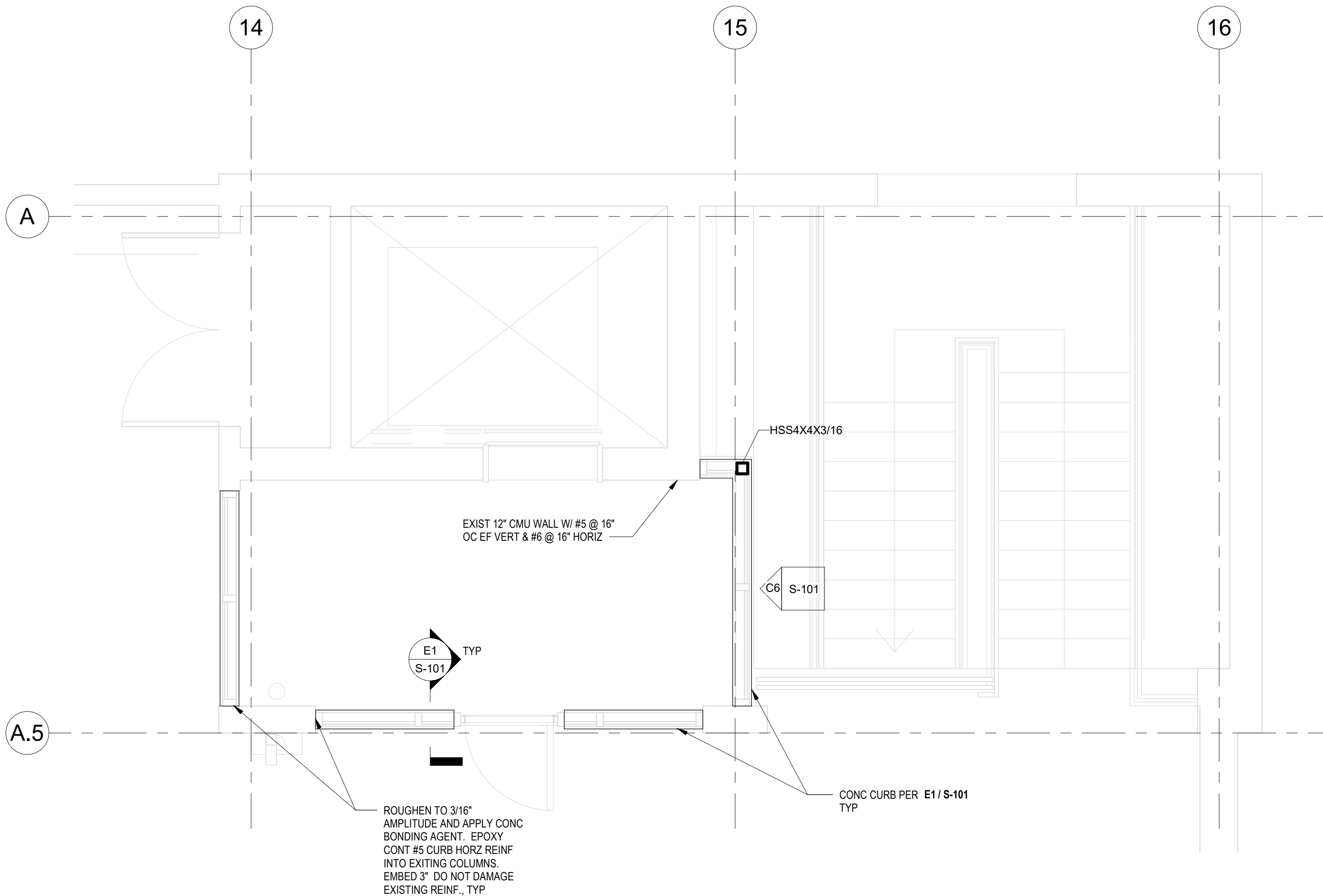
C1 LEVEL 4 - STRUCTURAL PLAN 3/8" = 1'-0"
