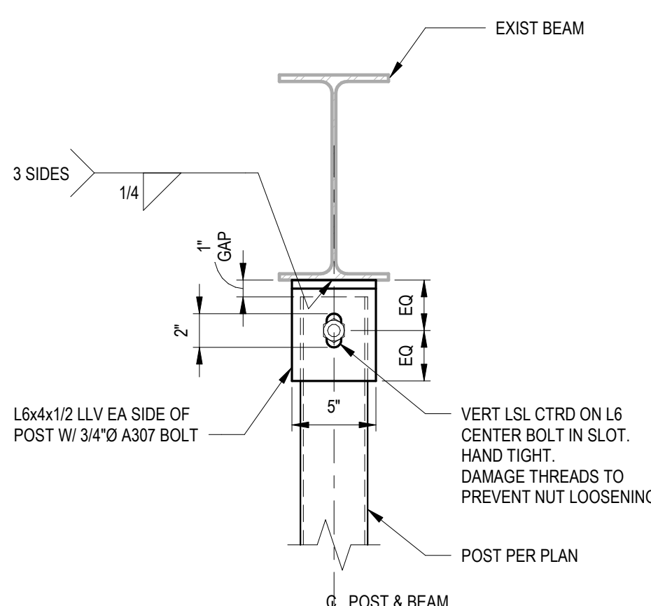
E7 POST TO EXIST CONN 1 1/2" = 1'-0"
