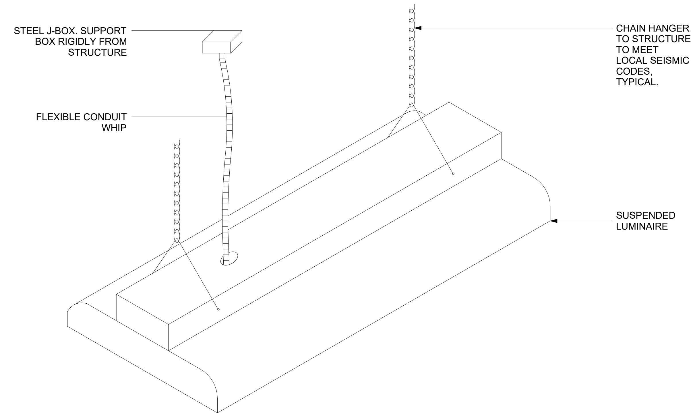
1 TYPICAL SUSPENDED LUMINAIRE INSTALLATION
