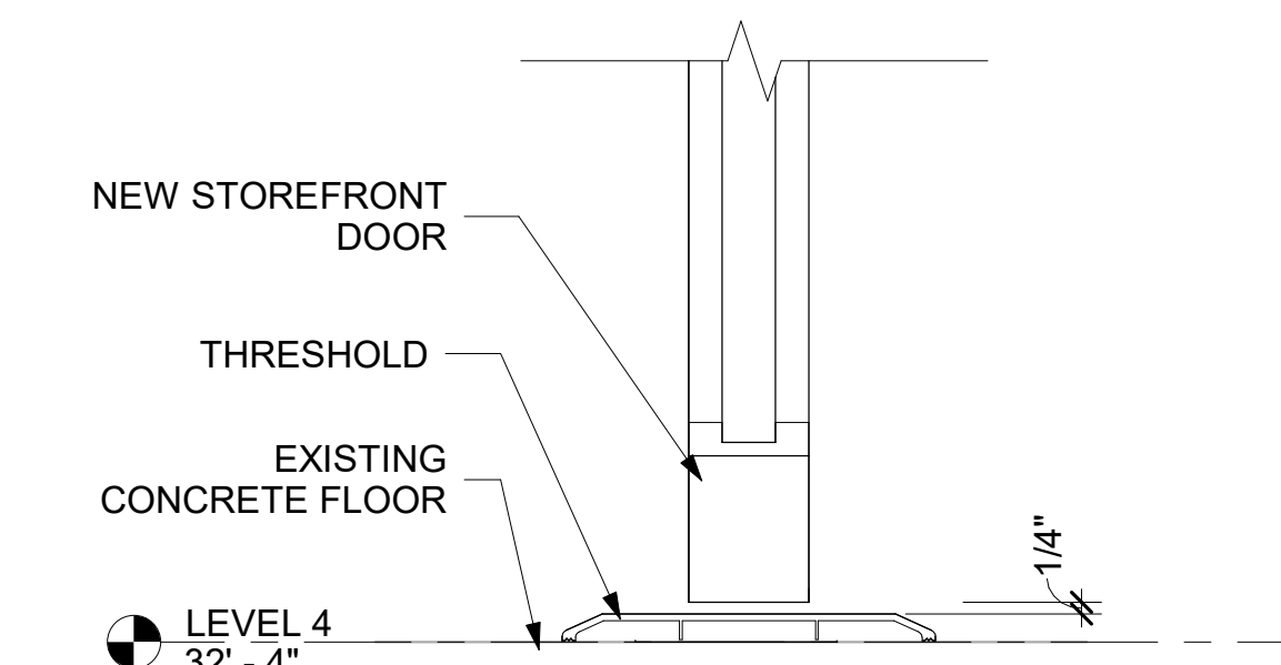
8 DOOR THRESHOLD @ STOREFRONT 3" = 1'-0"
