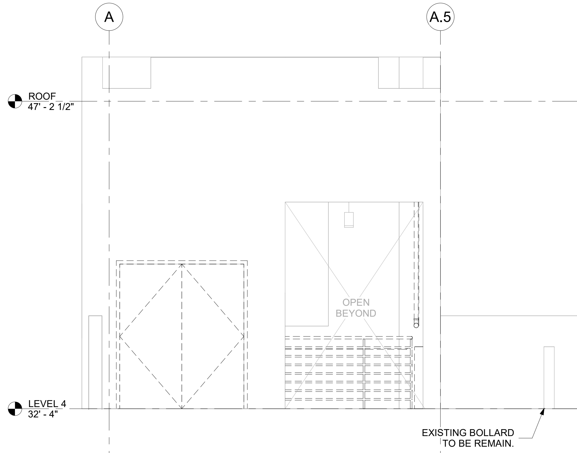
2 ELEVATOR LOBBY - WEST ELEVATION - EXISTING CONDITIONS 3/8" = 1'-0"
