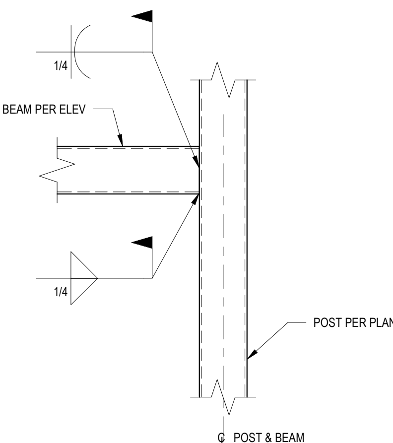
E5 TYP POST TO BEAM CONN 1 1/2" = 1'-0"
