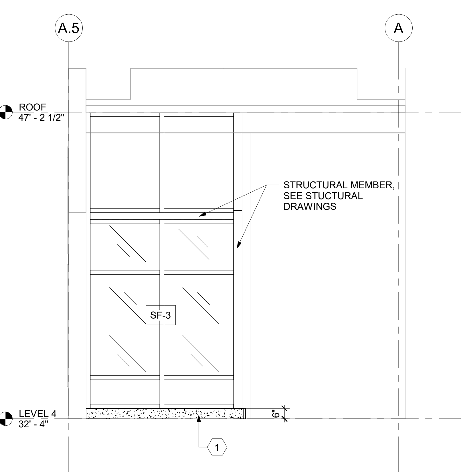
6 ELEVATOR LOBBY - EAST ELEVATION 3/8" = 1'-0"
