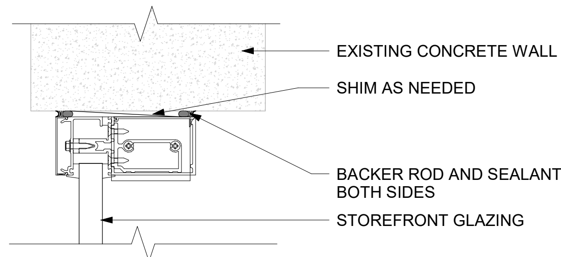
3 STOREFRONT HEAD DETAIL 3" = 1'-0"
