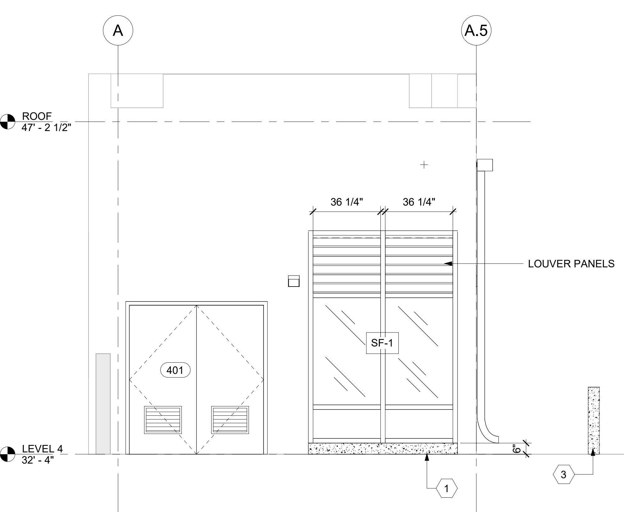
5 ELEVATOR LOBBY - WEST ELEVATION 3/8" = 1'-0"
