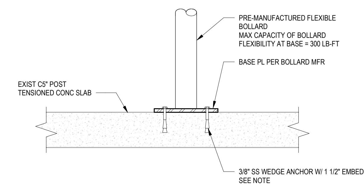
F7 BOLLARD TO EXIST SLAB CONN 1 1/2" = 1'-0"
