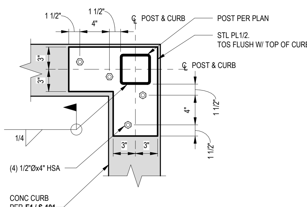
E3 POST BASE 1 1/2" = 1'-0"
