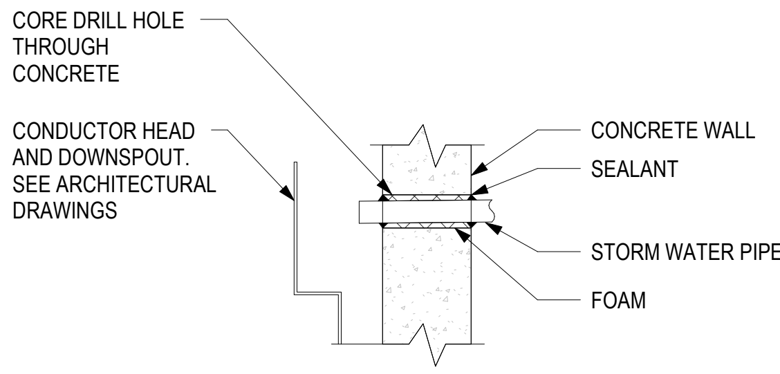
3 STORM WATER PIPE THROUGH CONCRETE WALL DETAIL NTS
