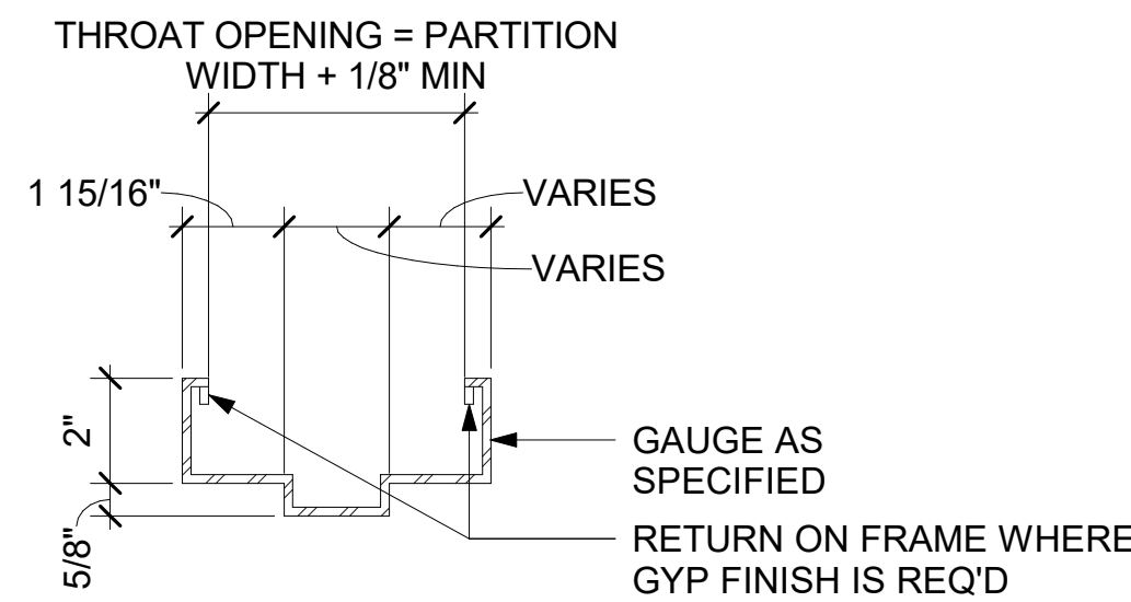
6 STANDARD DOOR FRAME 3" = 1'-0"
