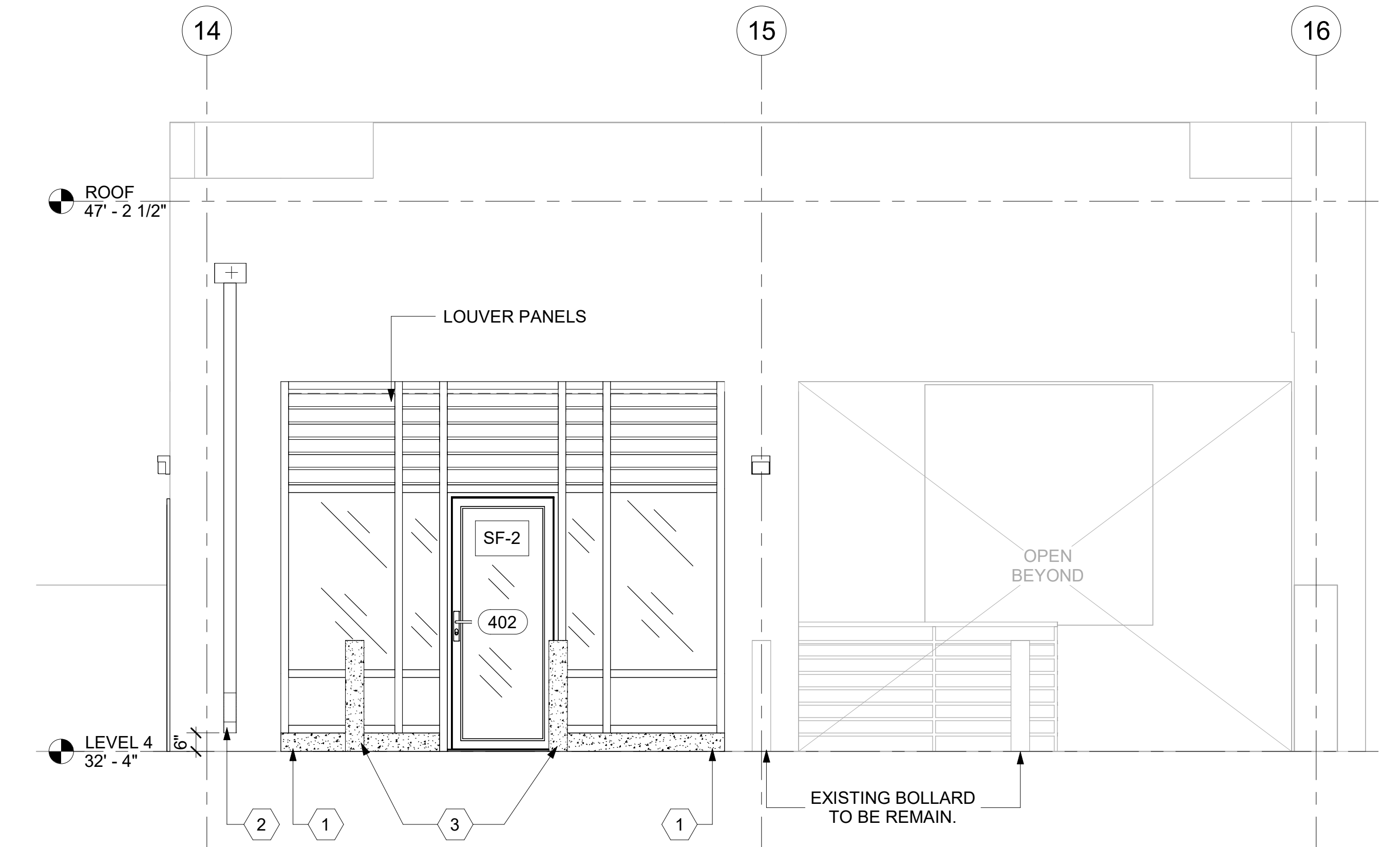
4 ELEVATOR LOBBY - SOUTH ELEVATION 3/8" = 1'-0"
