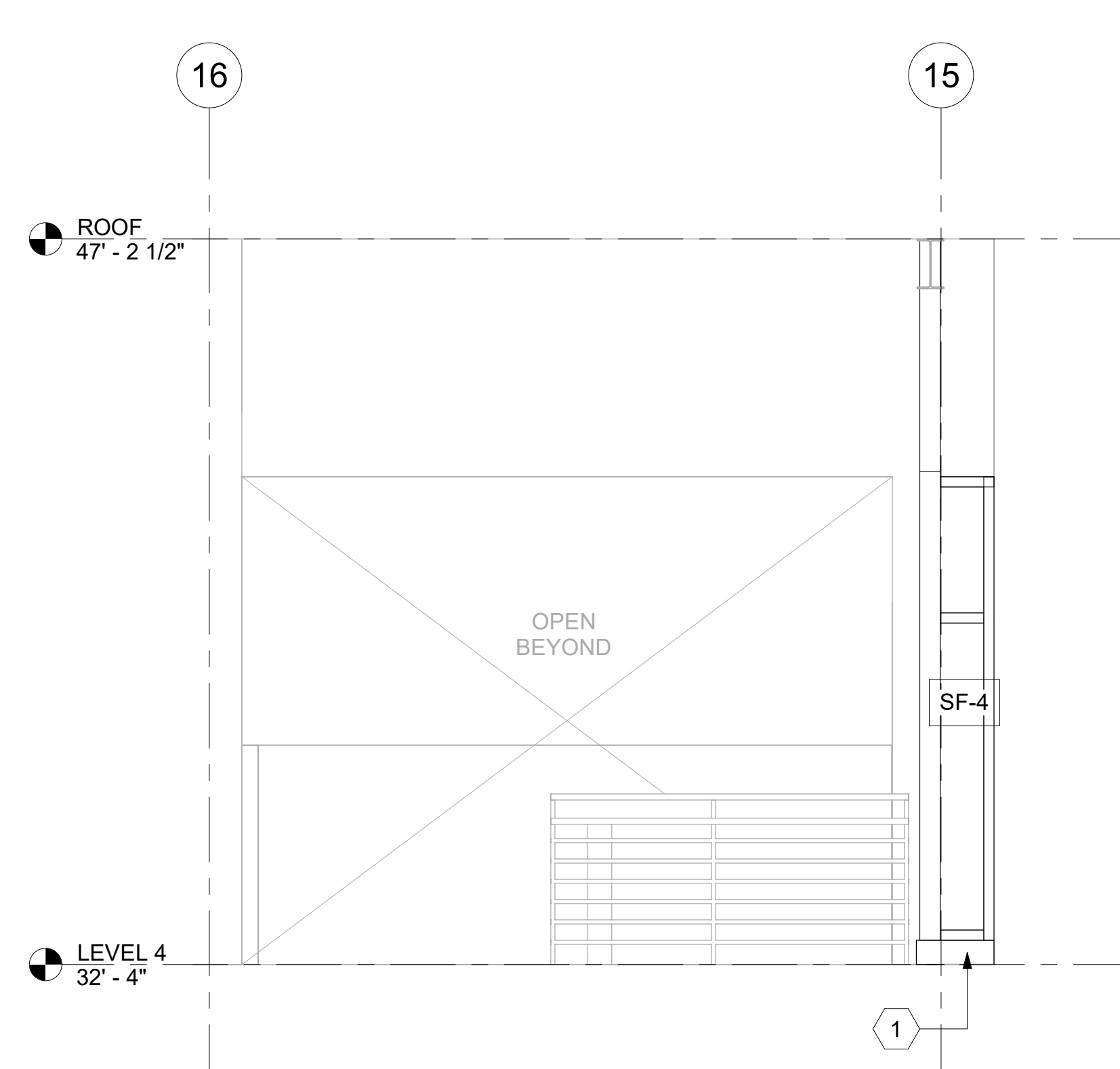
3 ELEVATOR LOBBY - SOUTH INTERIOR ELEVATION 3/8" = 1'-0"
