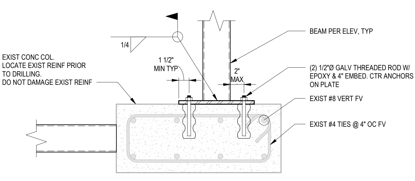
F5 BEAM TO EXIST CONC COL CONN 1 1/2" = 1'-0"
