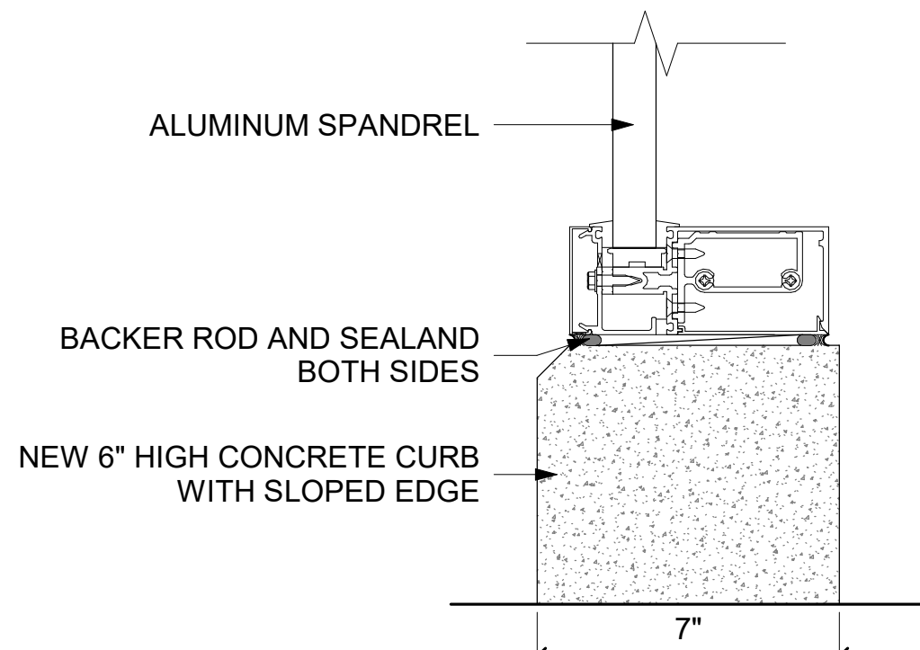
5 STOREFRONT SILL DETAIL 3" = 1'-0"
