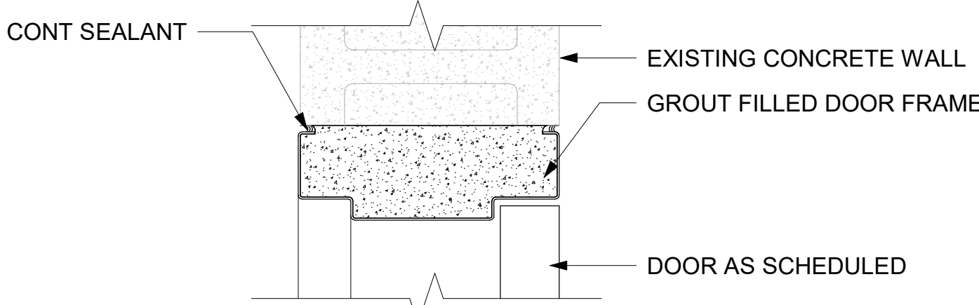
7 FRAMES @ EXISTING CONCRETE WALL 3" = 1'-0"
