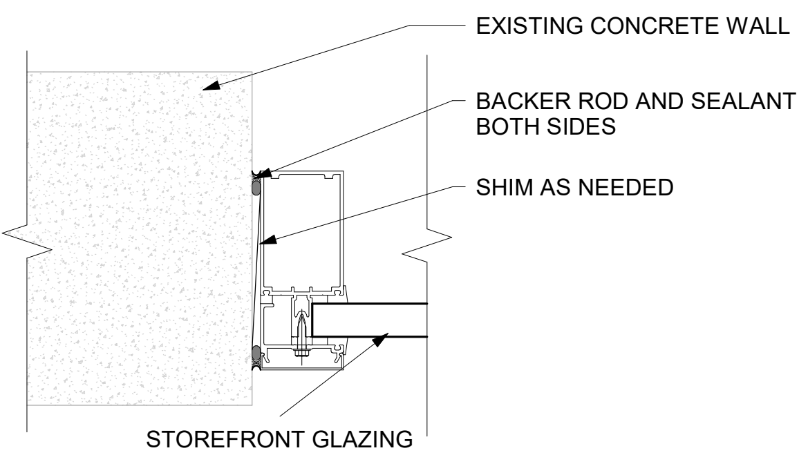
2 STOREFRONT JAMB DETAIL 3" = 1'-0"
